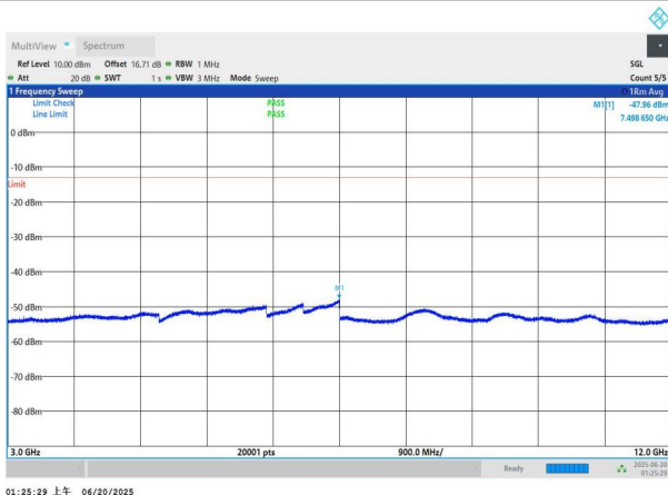
NTNV-n66-PC3-15-5-M-DFT-QPSK-Edge_1RB_Left-3000-12000-PASS
