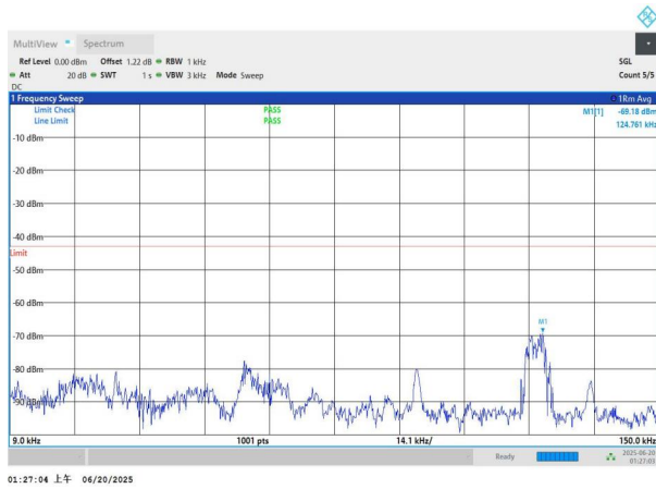
NTNV-n66-PC3-15-5-H-DFT-QPSK-Edge_1RB_Left-0.009-0.15-PASS
