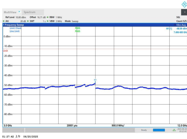
NTNV-n66-PC3-15-5-H-DFT-QPSK-Edge_1RB_Left-3000-12000-PASS
