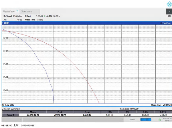
NTNV-n66-PC3-15-20-L-DFT-BPSK-Outer_Full-PASS
