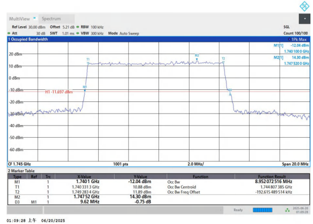
NTNV-n66-PC3-15-10-M-DFT-64QAM-Outer_Full-Ant1-PASS
