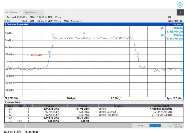
NTNV-n66-PC3-15-5-M-DFT-BPSK-Outer_Full-Ant1-PASS
