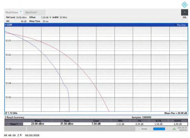
NTNV-n66-PC3-15-20-L-DFT-QPSK-Outer_Full-PASS
