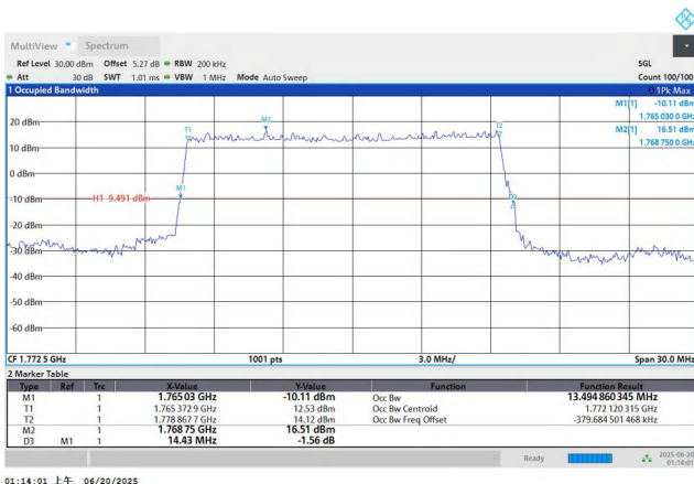
NTNV-n66-PC3-15-15-H-DFT-BPSK-Outet_Full-Ant1-PASS
