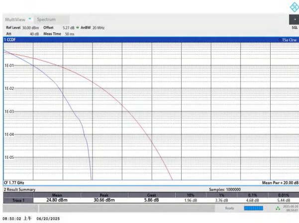
NTNV-n66-PC3-15-20-H-DFT-BPSK-Outer_Full-PASS
