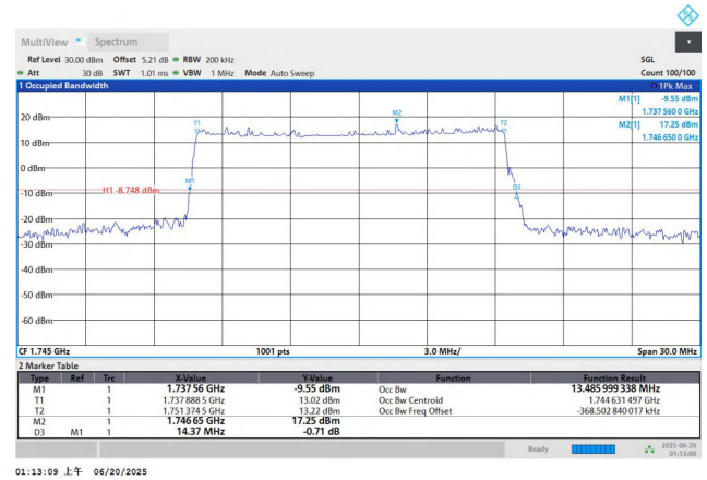
NTNV-n66-PC3-15-15-M-DFT-16QAM-Outet_Full-Ant1-PASS
