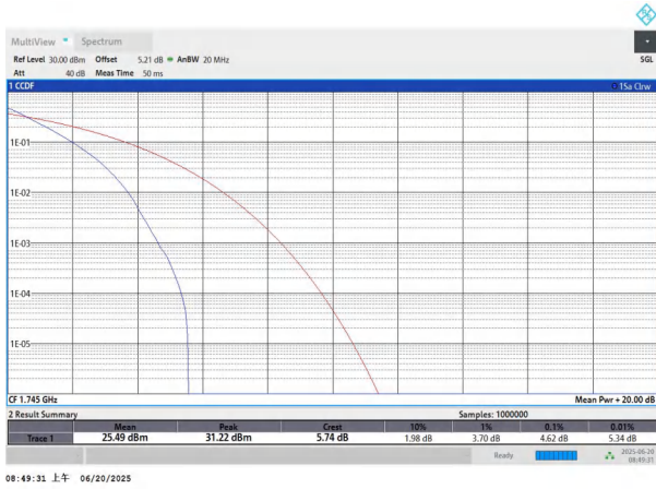
NTNV-n66-PC3-15-20-M-DFT-BPSK-Outer_Full-PASS
