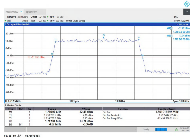
NTNV-n66-PC3-15-5-L-DFT-64QAM-Outer_Full-Ant1-PASS
