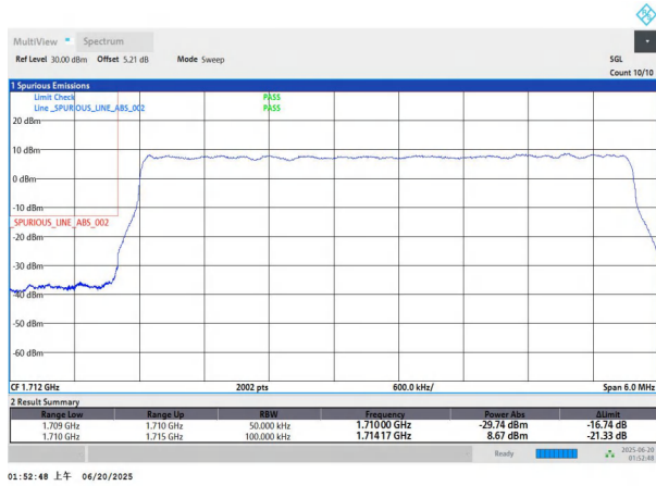
NTNV-n66-PC3-15-5-L-DFT-QPSK-Outer_Full-PASS
