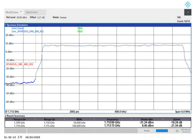
NTNV-n66-PC3-15-5-L-DFT-BPSK-Outer_Full-PASS
