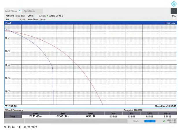
NTNV-n66-PC3-15-20-M-DFT-QPSK-Outer_Full-PASS
