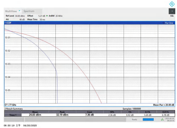
NTNV-n66-PC3-15-20-H-DFT-QPSK-Outer_Full-PASS
