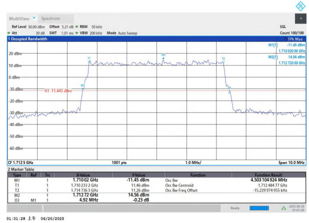
NTNV-n66-PC3-15-5-L-DFT-QPSK-Outer_Full-Ant1-PASS
