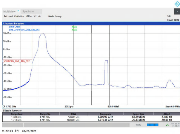
NTNV-n66-PC3-15-5-L-DFT-BPSK-Edge_1RB_Left-PASS
