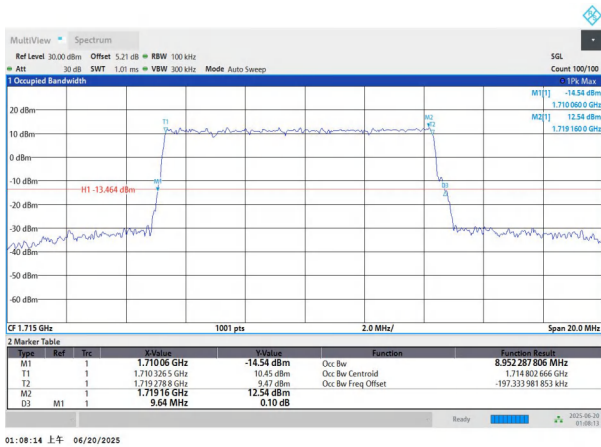
NTNV-n66-PC3-15-10-L-DFT-64QAM-Outer_Full-Ant1-PASS
