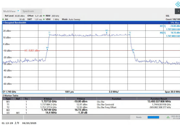
NTNV-n66-PC3-15-15-M-DFT-64QAM-Outet_Full-Ant1-PASS
