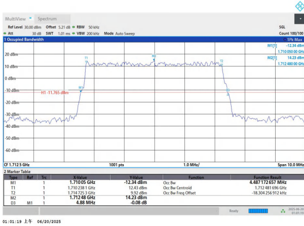
NTNV-n66-PC3-15-5-L-DFT-BPSK-Outer_Full-Ant1-PASS
