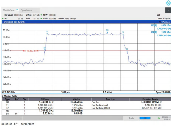
NTNV-n66-PC3-15-10-M-DFT-BPSK-Outer_Full-Ant1-PASS
