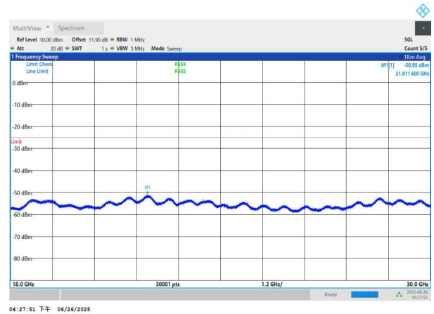
NTNV-n41-PC3-30-80-H-DFT-BPSK-Edge_1RB_Left-18000-3000 0-PASS
