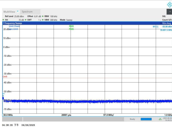
NTNV-n41-PC3-30-100-H-DFT-QPSK-Edge_1RB_Left-30-1000- PASS
