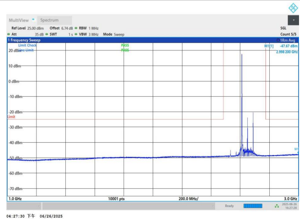
NTNV-n41-PC3-30-80-H-DFT-BPSK-Edge_1RB_Left-1000-3000-P ASS
