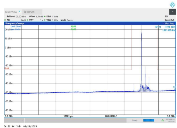
NTNV-n41-PC3-30-90-H-DFT-BPSK-Edge_1RB_Left-1000-3000-P ASS
