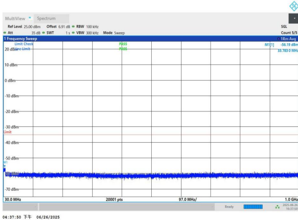
NTNV-n41-PC3-30-100-H-DFT-BPSK-Edge_1RB_Left-30-1000-P ASS
