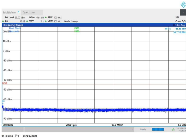
NTNV-n41-PC3-30-100-M-DFT-QPSK-Edge_1RB_Left-30-1000- PASS
