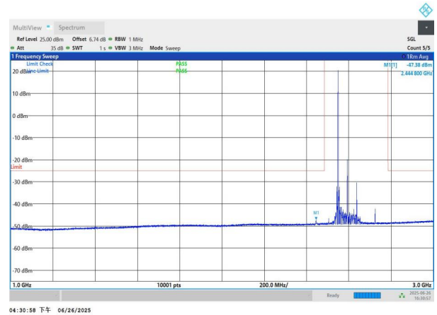
NTNV-n41-PC3-30-90-M-DFT-BPSK-Edge_1RB_Left-1000-3000-P PASS
