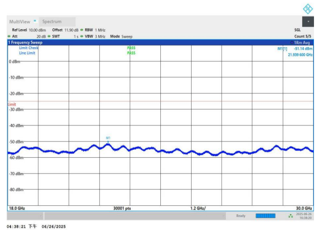
NTNV-n41-PC3-30-100-H-DFT-BPSK-Edge_1RB_Left-18000-300 00-PASS
