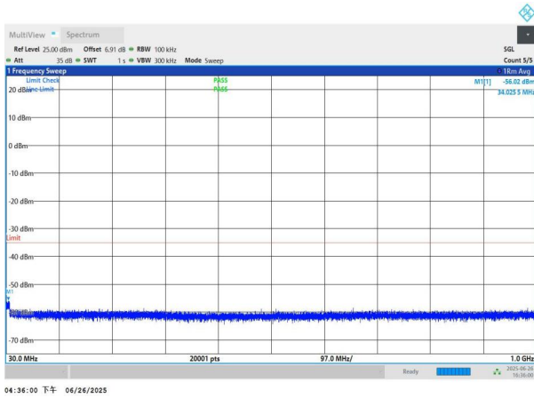
NTNV-n41-PC3-30-100-M-DFT-BPSK-Edge_1RB_Left-30-1000- PASS
