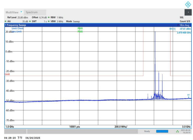
NTNV-n41-PC3-30-80-H-DFT-QPSK-Edge_1RB_Left-1000-3000-P PASS
