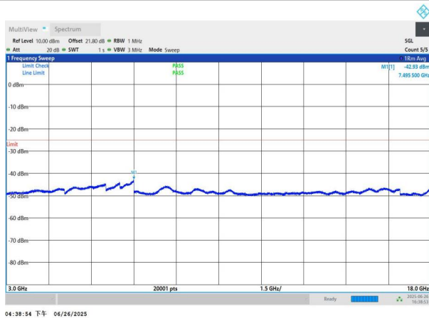
NTNV-n41-PC3-30-100-H-DFT-QPSK-Edge_1RB_Left-3000-180 00-PASS
