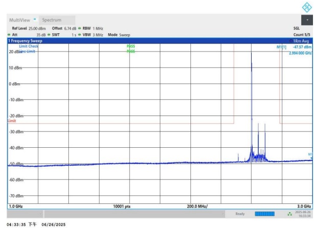
NTNV-n41-PC3-30-90-H-DFT-QPSK-Edge_1RB_Left-1000-3000-P PASS
