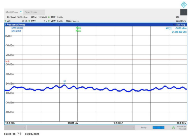
NTNV-n41-PC3-30-90-H-DFT-BPSK-Edge_1RB_Left-18000-3000 0-PASS
