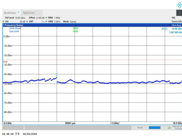
NTNV-n41-PC3-30-100-H-DFT-BPSK-Edge_1RB_Left-3000-180 00-PASS
