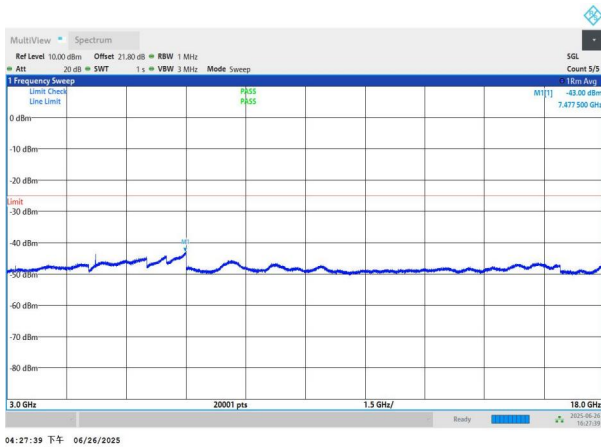
NTNV-n41-PC3-30-80-H-DFT-BPSK-Edge_1RB_Left-3000-1800 0-PASS
