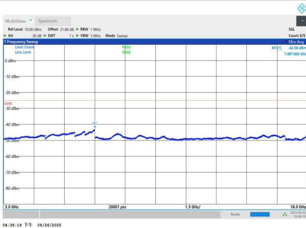
NTNV-n41-PC3-30-100-M-DFT-BPSK-Edge_1RB_Left-3000-180 00-PASS
