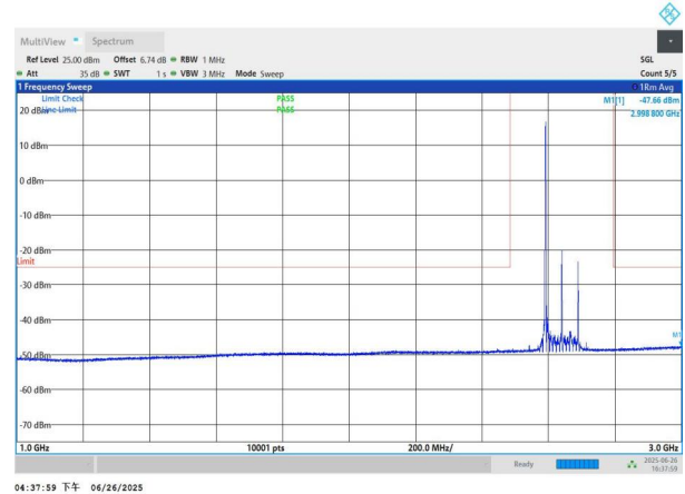
NTNV-n41-PC3-30-100-H-DFT-BPSK-Edge_1RB_Left-1000-3000- PASS
