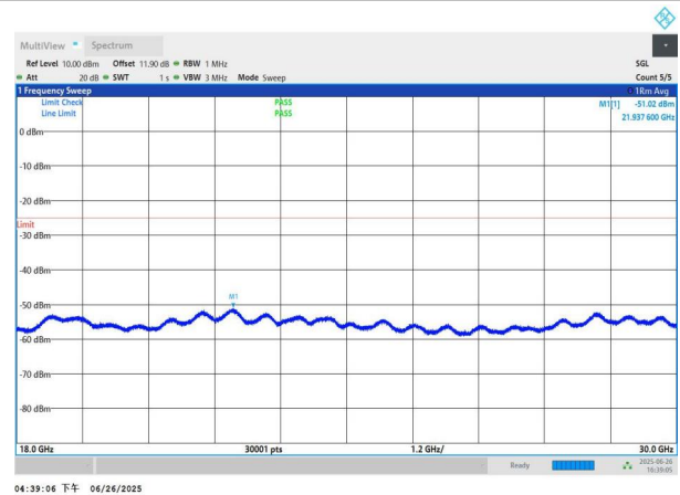
NTNV-n41-PC3-30-100-H-DFT-QPSK-Edge_1RB_Left-18000-300 00-PASS
