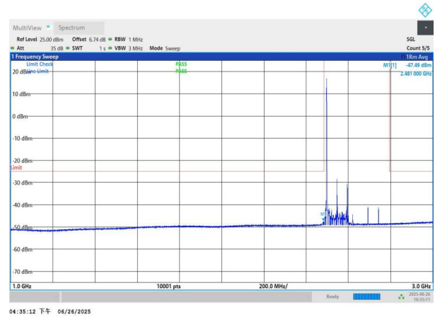
NTNV-n41-PC3-30-100-L-DFT-QPSK-Edge_1RB_Left-1000-3000-P PASS
