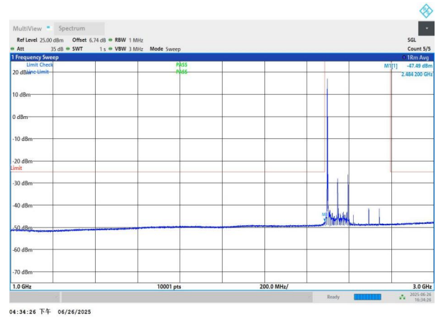
NTNV-n41-PC3-30-100-L-DFT-BPSK-Edge_1RB_Left-1000-3000-P PASS
