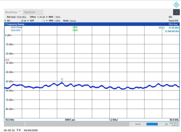
NTNV-n41-PC3-30-100-M-DFT-BPSK-Edge_1RB_Left-18000-300 00-PASS
