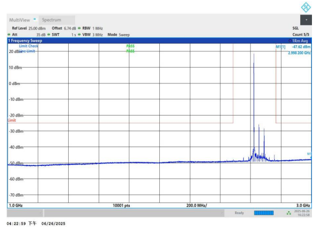
NTNV-n41-PC3-30-70-H-DFT-QPSK-Edge_1RB_Left-1000-3000-P PASS
