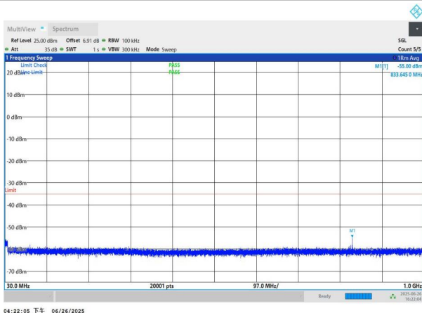
NTNV-n41-PC3-30-70-H-DFT-BPSK-Edge_1RB_Left-30-1000-P ASS
