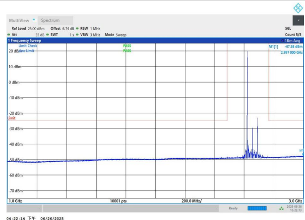
NTNV-n41-PC3-30-70-H-DFT-BPSK-Edge_1RB_Left-1000-3000-P ASS
