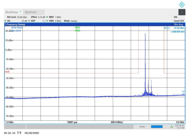
NTNV-n41-PC3-30-70-M-DFT-QPSK-Edge_1RB_Left-1000-3000- PASS
