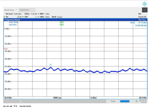
NTNV-n41-PC3-30-70-M-DFT-BPSK-Edge_1RB_Left-18000-3000 0-PASS
