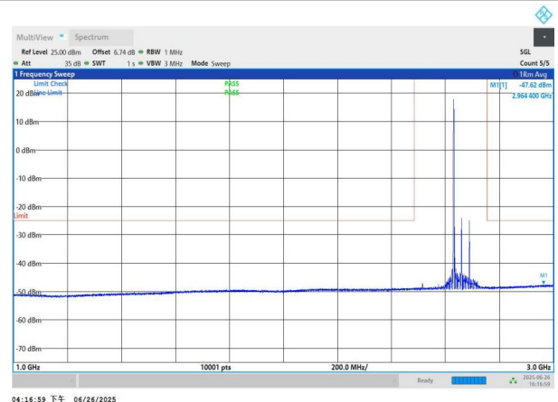
NTNV-n41-PC3-30-60-H-DFT-BPSK-Edge_1RB_Left-1000-3000-P ASS
