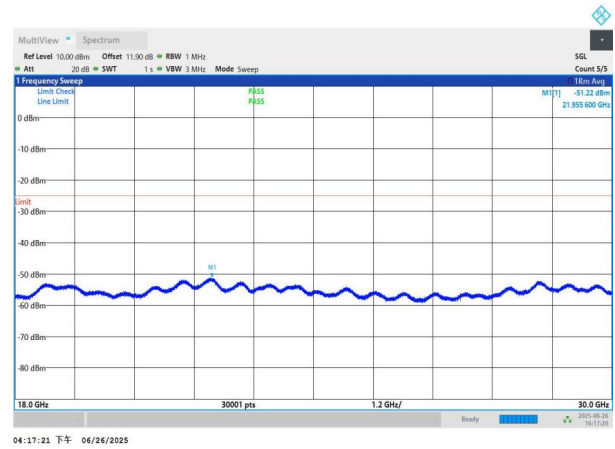
NTNV-n41-PC3-30-60-H-DFT-BPSK-Edge_1RB_Left-18000-3000 0-PASS
