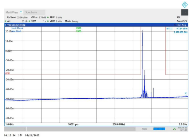
NTNV-n41-PC3-30-60-L-DFT-BPSK-Edge_1RB_Left-1000-3000-P
