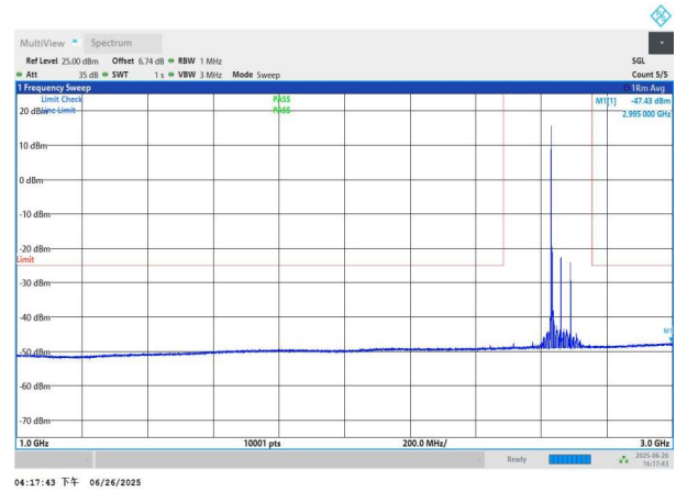
NTNV-n41-PC3-30-60-H-DFT-QPSK-Edge_1RB_Left-1000-3000-P PASS
