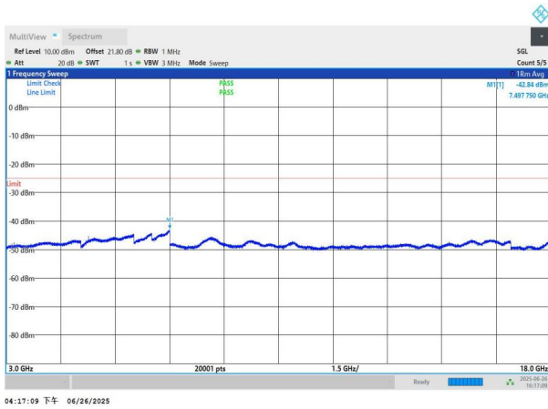
NTNV-n41-PC3-30-60-H-DFT-BPSK-Edge_1RB_Left-3000-1800 0-PASS
