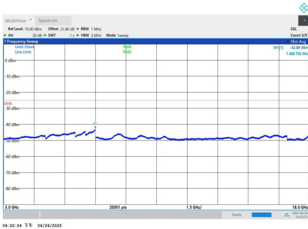
NTNV-n41-PC3-30-70-H-DFT-BPSK-Edge_1RB_Left-3000-1800 0-PASS
