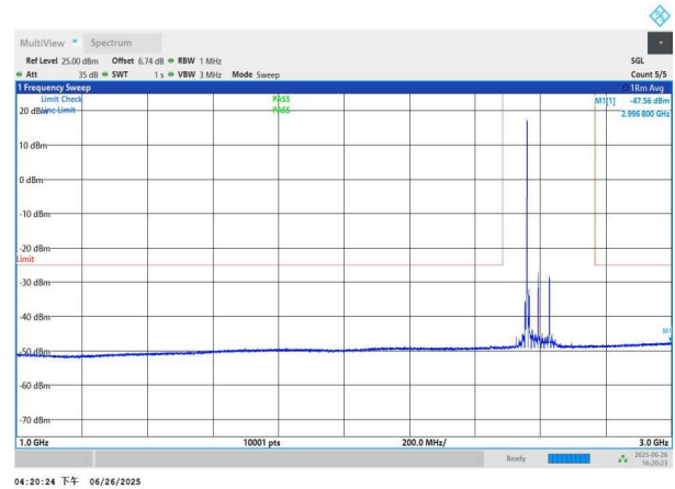
NTNV-n41-PC3-30-70-M-DFT-BPSK-Edge_1RB_Left-1000-3000-P PASS
