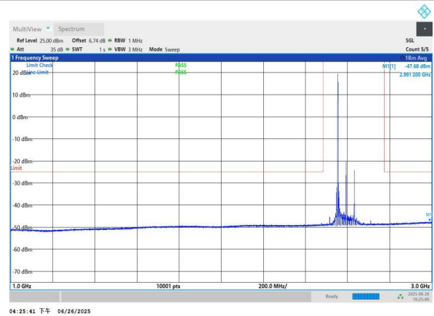
NTNV-n41-PC3-30-80-M-DFT-BPSK-Edge_1RB_Left-1000-3000-P PASS
