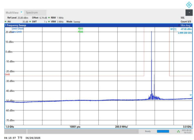
NTNV-n41-PC3-30-60-M-DFT-QPSK-Edge_1RB_Left-1000-3000- PASS
