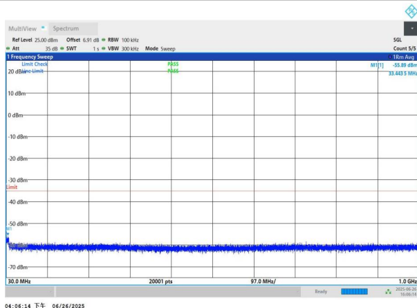
NTNV-n41-PC3-30-40-H-DFT-BPSK-Edge_1RB_Left-30-1000-P ASS
