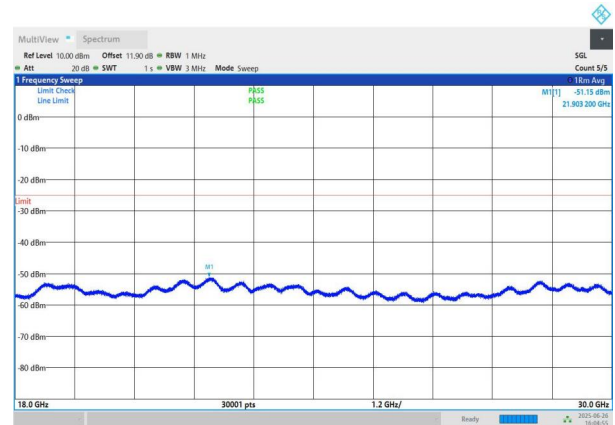
NTNV-n41-PC3-30-40-M-DFT-BPSK-Edge_1RB_Left-18000-3000 0-PASS
