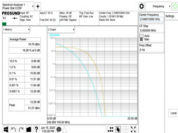
NTNV-n41-PC3-30-100-L-DFT-BPSK-Outter_Full-PASS
