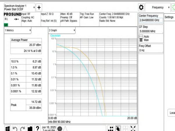
NTNV-n41-PC3-30-90-H-DFT-QPSK-Outer_Full-PASS
