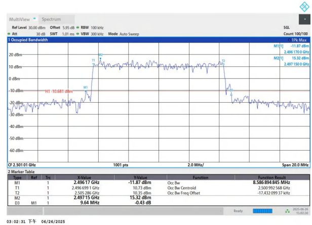
NTNV-n41-PC3-30-10-L-DFT-64QAM-Outer_Full-Ant1-PASS
