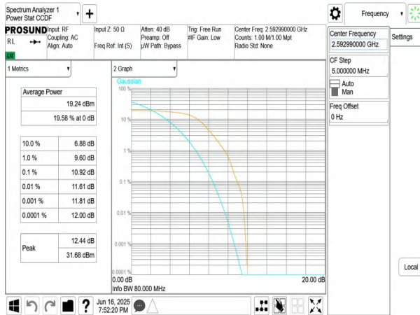
NTNV-n41-PC3-30-80-M-DFT-BPSK-Outer_Full-PASS
