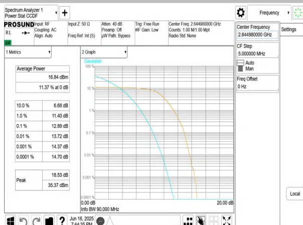
NTNV-n41-PC3-30-90-H-DFT-BPSK-Outer_Full-PASS
