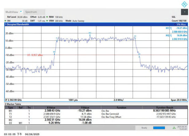
NTNV-n41-PC3-30-10-M-DFT-BPSK-Outer_Full-Ant1-PASS
