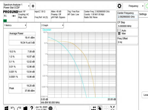
NTNV-n41-PC3-30-90-M-DFT-QPSK-Outer_Full-PASS
