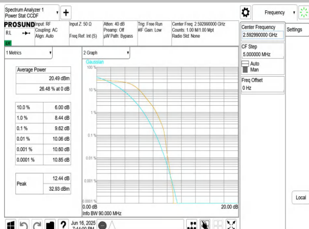
NTNV-n41-PC3-30-90-M-DFT-BPSK-Outer_Full-PASS
