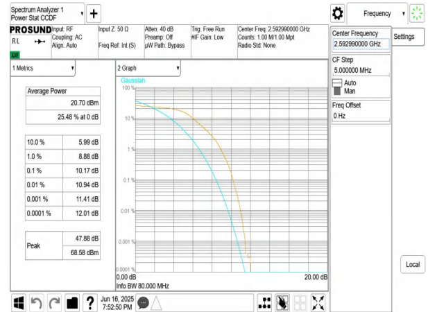
NTNV-n41-PC3-30-80-M-DFT-QPSK-Outer_Full-PASS
