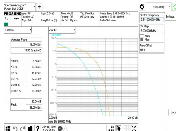
NTNV-n41-PC3-30-90-L-DFT-QPSK-Outer_Full-PASS
