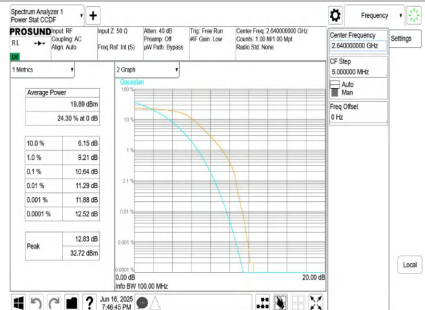
NTNV-n41-PC3-30-100-H-DFT-QPSK-Outter_Full-PASS
