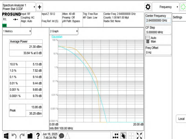
NTNV-n41-PC3-30-100-H-DFT-BPSK-Outter_Full-PASS
