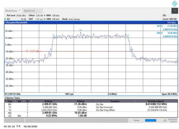
NTNV-n41-PC3-30-10-L-DFT-QPSK-Outer_Full-Ant1-PASS
