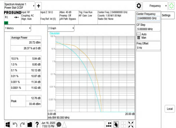
NTNV-n41-PC3-30-80-H-DFT-QPSK-Outer_Full-PASS
