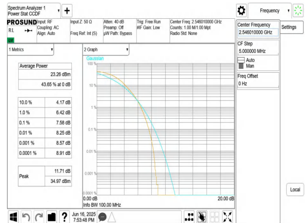
NTNV-n41-PC3-30-100-L-DFT-QPSK-Outter_Full-PASS
