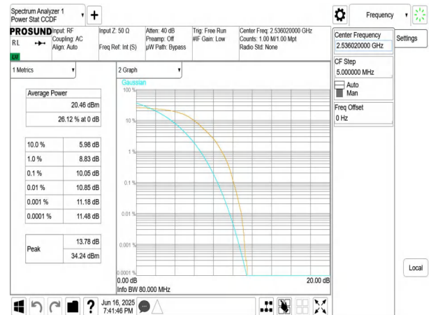
NTNV-n41-PC3-30-80-L-DFT-QPSK-Outer_Full-PASS
