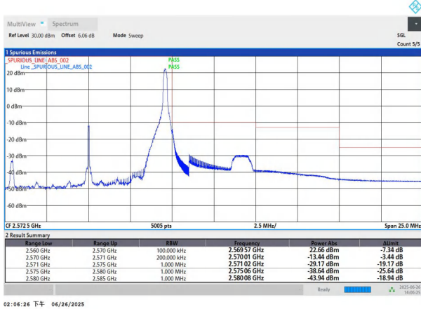
NTNV-n7-PC3-15-10-H-DFT-BPSK-Edge_1RB_Right-PASS
