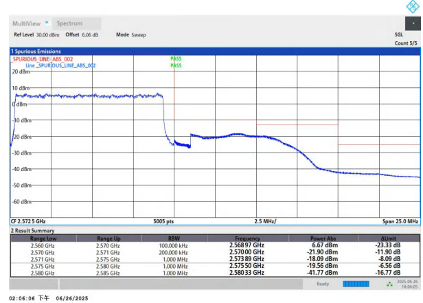
NTNV-n7-PC3-15-10-H-DFT-BPSK-Outer_Full-PASS
