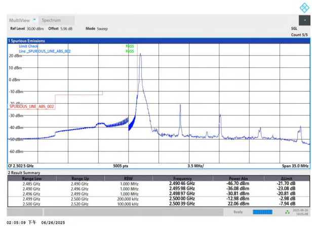
NTNV-n7-PC3-15-10-L-DFT-BPSK-Edge_1RB_Left-PASS
