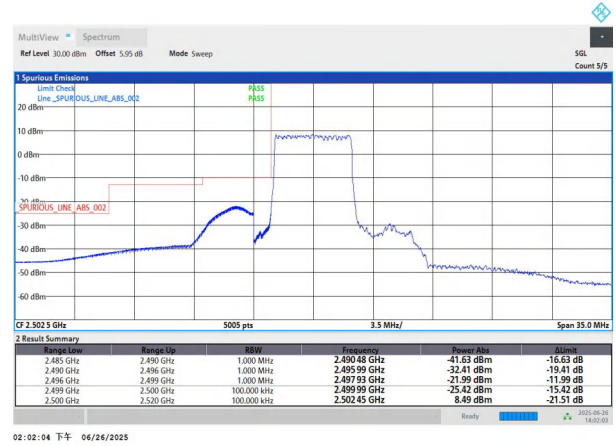
NTNV-n7-PC3-15-5-L-DFT-BPSK-Outer_Full-PASS
