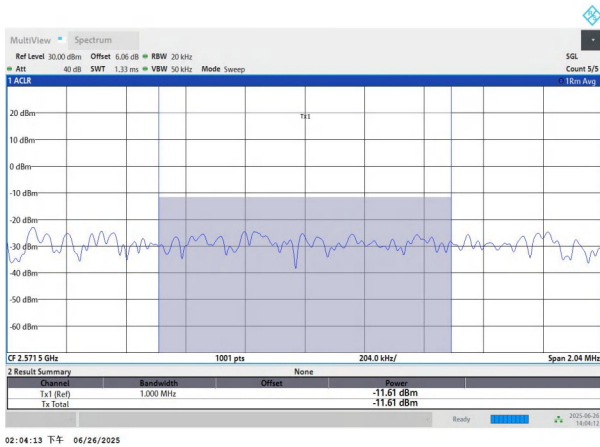
NTNV-n7-PC3-15-5-H-DFT-QPSK-Outer_Full-PASS_Final1
