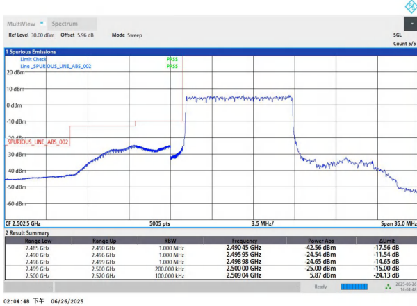
NTNV-n7-PC3-15-10-L-DFT-BPSK-Outer_Full-PASS
