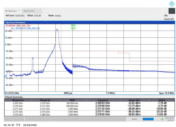
NTNV-n7-PC3-15-5-H-DFT-BPSK-Edge_1RB_Right-PASS
