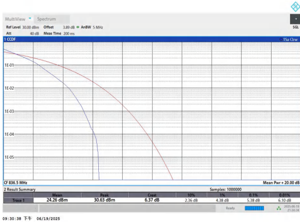
NTNV-n5-PC3-15-5-M-DFT-BPSK-Outer_Full-PASS
