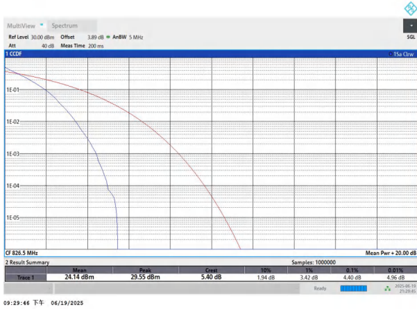
NTNV-n5-PC3-15-5-L-DFT-BPSK-Outer_Full-PASS
