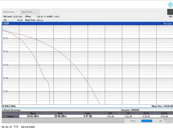
NTNV-n5-PC3-15-5-H-DFT-BPSK-Outer_Full-PASS
