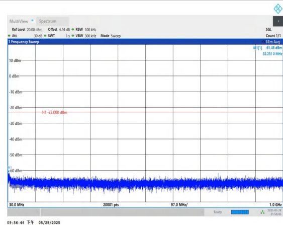
Band66-3MHz-QPSK-131987-1RB#0-30~1000-PASS
