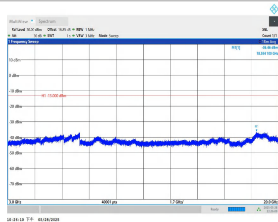
Band66-10MHz-QPSK-132022-1RB#0-3000~20000-PASS
