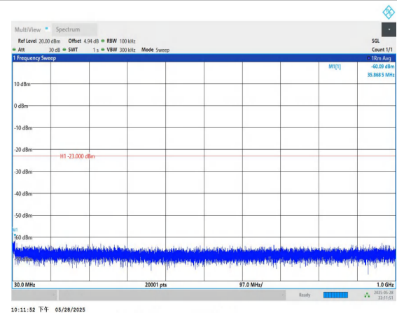
Band66-5MHz-QPSK-132322-1RB#0-30~1000-PASS
