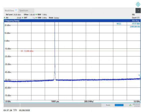
Band66-3MHz-QPSK-132322-1RB#0-1000~3000-PASS
