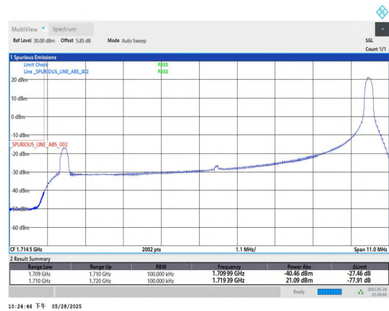
Band66-10MHz-QPSK-132022-1RB#49-PASS
