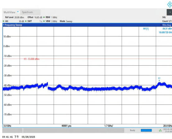
Band66-1.4MHz-QPSK-131979-1RB#0-3000~20000-PASS
