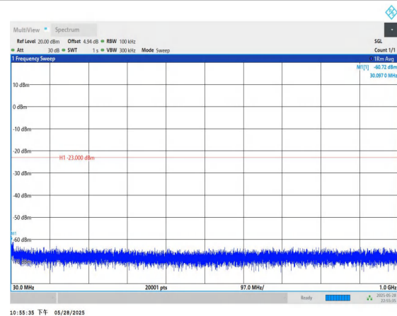
Band66-20MHz-QPSK-132072-1RB#0-30~1000-PASS
