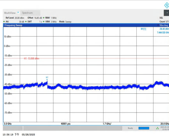
Band66-20MHz-QPSK-132322-1RB#0-3000~20000-PASS
