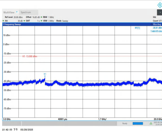
Band66-15MHz-QPSK-132597-1RB#0-3000~20000-PASS
