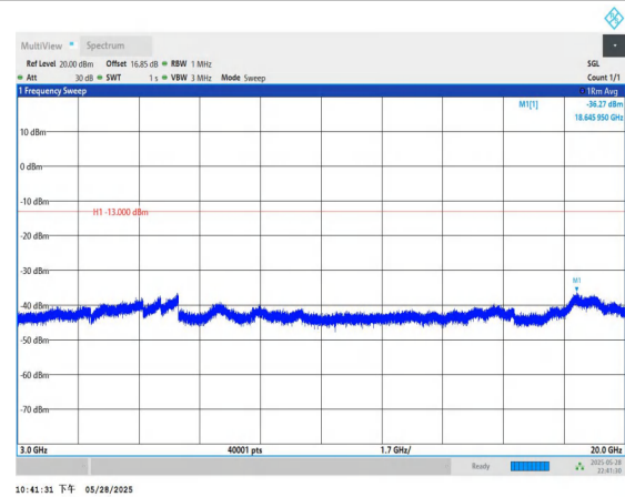
Band66-15MHz-QPSK-132322-1RB#0-3000~20000-PASS
