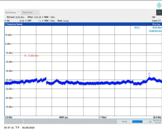
Band66-3MHz-QPSK-131987-1RB#0-3000~20000-PASS
