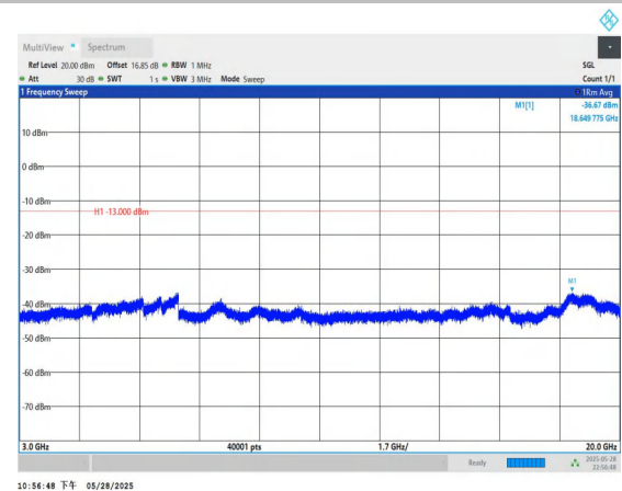
Band66-20MHz-QPSK-132572-1RB#0-3000~20000-PASS
