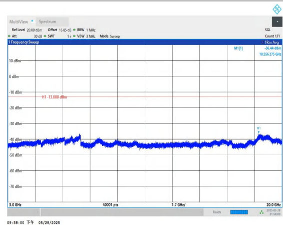
Band66-3MHz-QPSK-132657-1RB#0-3000~20000-PASS
