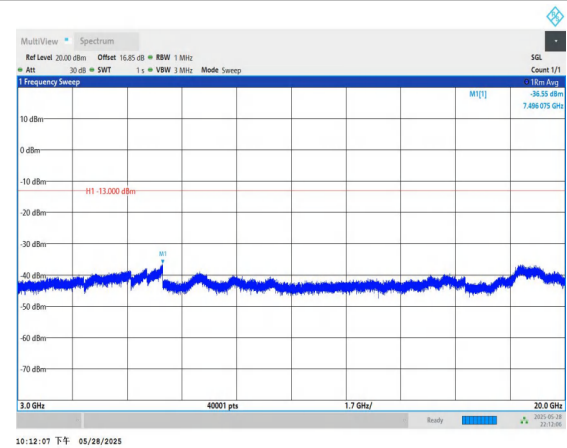
Band66-5MHz-QPSK-132322-1RB#0-3000~20000-PASS
