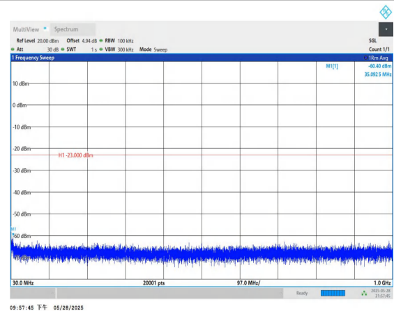
Band66-3MHz-QPSK-132657-1RB#0-30~1000-PASS
