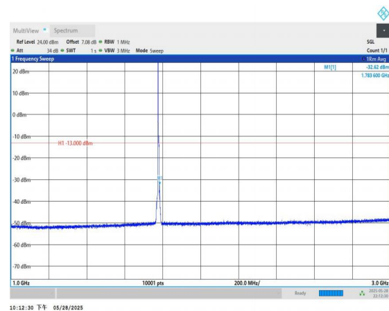
Band66-5MHz-QPSK-132647-1RB#0-1000~3000-PASS
