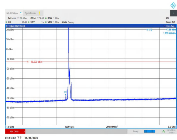
Band66-20MHz-QPSK-132322-1RB#0-1000~3000-PASS
