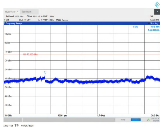
Band66-10MHz-QPSK-132622-1RB#0-3000~20000-PASS
