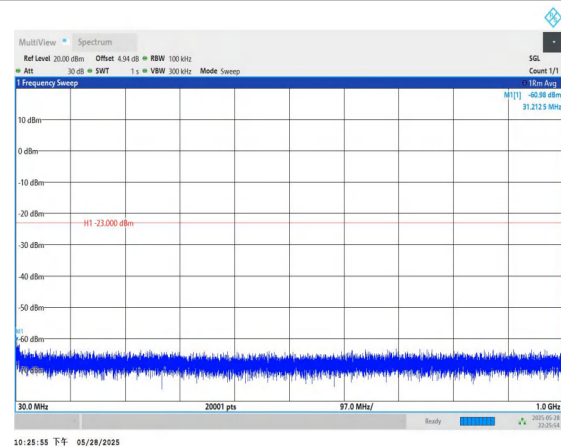
Band66-10MHz-QPSK-132022-1RB#0-30~1000-PASS
