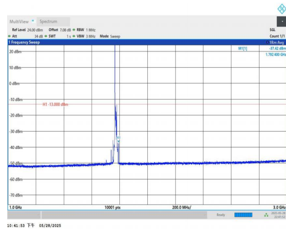
Band66-15MHz-QPSK-132597-1RB#0-1000~3000-PASS
