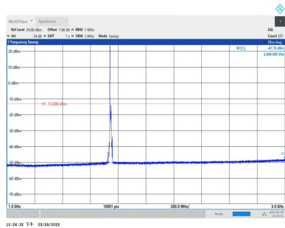
Band66-10MHz-QPSK-132322-1RB#0-1000~3000-PASS
