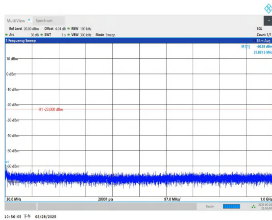
Band66-20MHz-QPSK-132322-1RB#0-30~1000-PASS
