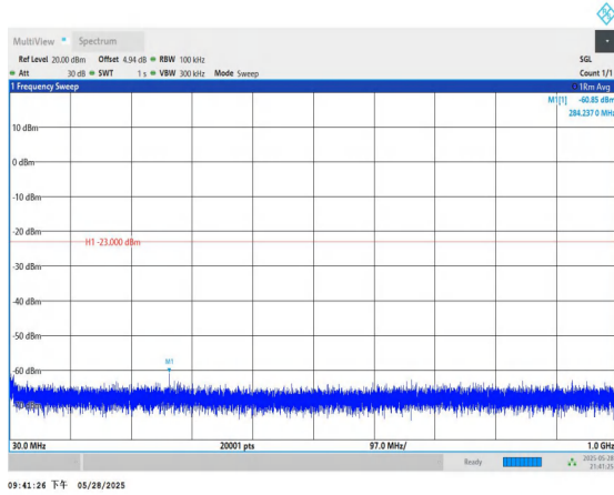
Band66-1.4MHz-QPSK-131979-1RB#0-30~1000-PASS
