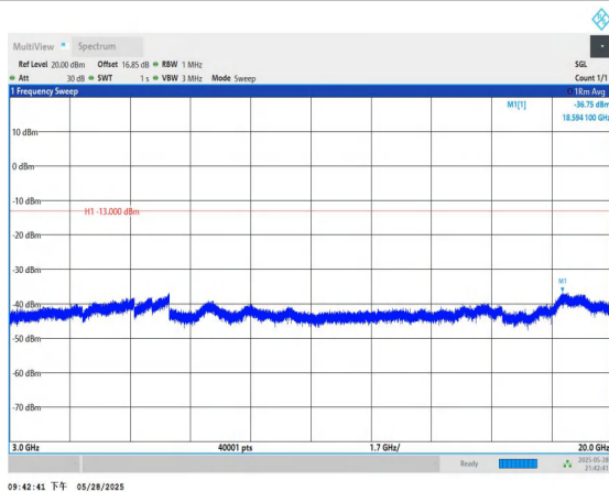
Band66-1.4MHz-QPSK-132665-1RB#0-3000~20000-PASS
