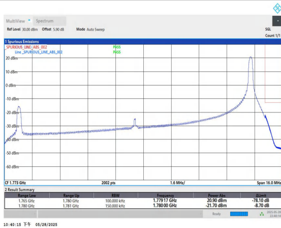
Band66-15MHz-QPSK-132597-1RB#74-PASS
