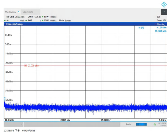
Band66-10MHz-QPSK-132622-1RB#0-30~1000-PASS
