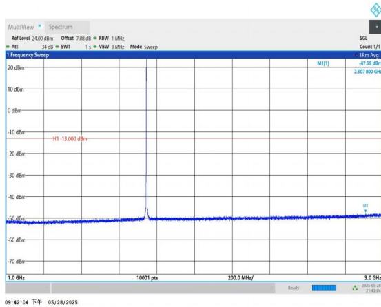
Band66-1.4MHz-QPSK-132322-1RB#0-1000~3000-PASS
