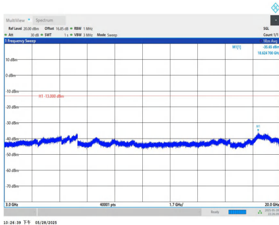
Band66-10MHz-QPSK-132322-1RB#0-3000~20000-PASS
