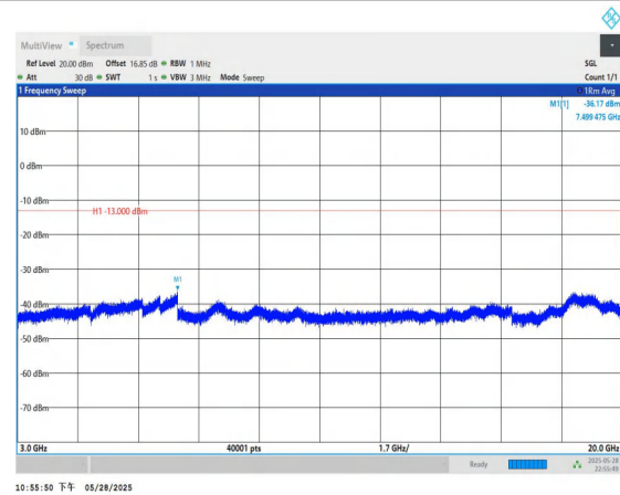
Band66-20MHz-QPSK-132072-1RB#0-3000~20000-PASS
