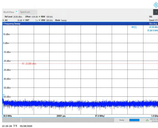
Band66-10MHz-QPSK-132322-1RB#0-30~1000-PASS
