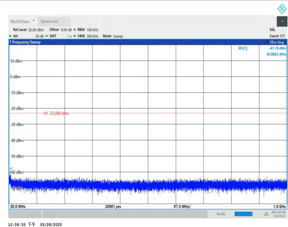
Band66-20MHz-QPSK-132572-1RB#0-30~1000-PASS
