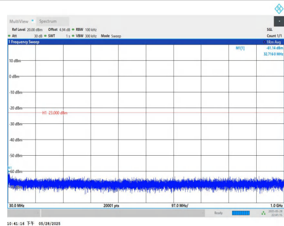
Band66-15MHz-QPSK-132322-1RB#0-30~1000-PASS
