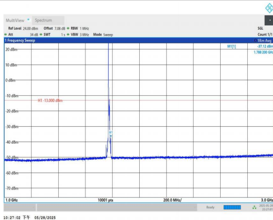
Band66-10MHz-QPSK-132622-1RB#0-1000~3000-PASS
