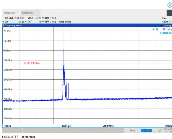
Band66-20MHz-QPSK-132072-1RB#0-1000~3000-PASS
