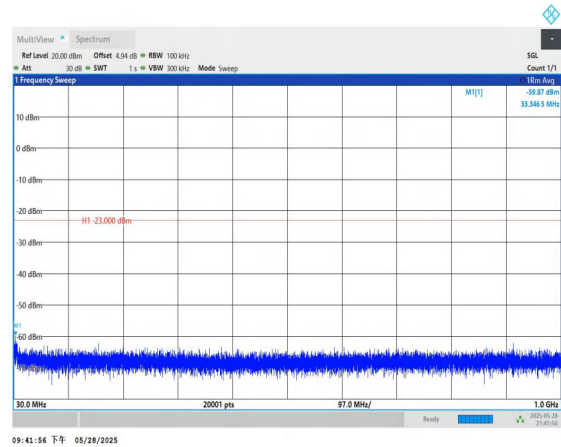
Band66-1.4MHz-QPSK-132322-1RB#0-30~1000-PASS
