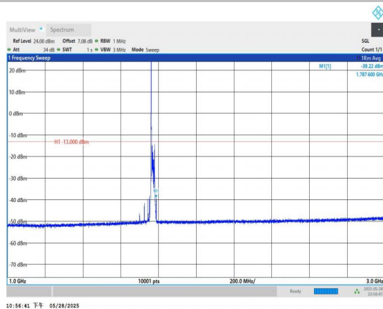
Band66-20MHz-QPSK-132572-1RB#0-1000~3000-PASS
