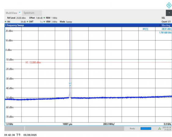
Band66-1.4MHz-QPSK-132665-1RB#0-1000~3000-PASS
