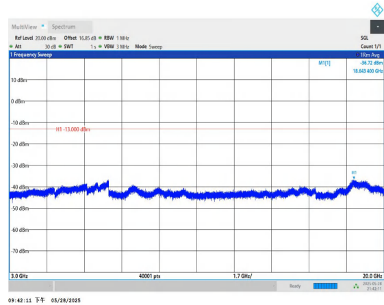
Band66-1.4MHz-QPSK-132322-1RB#0-3000~20000-PASS
