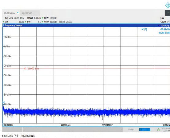
Band66-15MHz-QPSK-132597-1RB#0-30~1000-PASS
