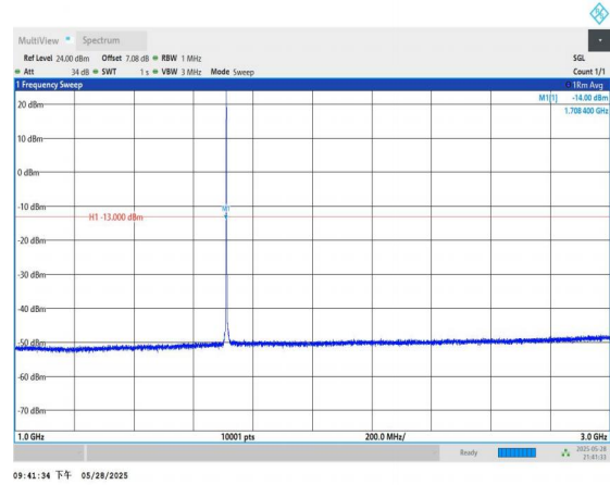
Band66-1.4MHz-QPSK-131979-1RB#0-1000~3000-PASS
