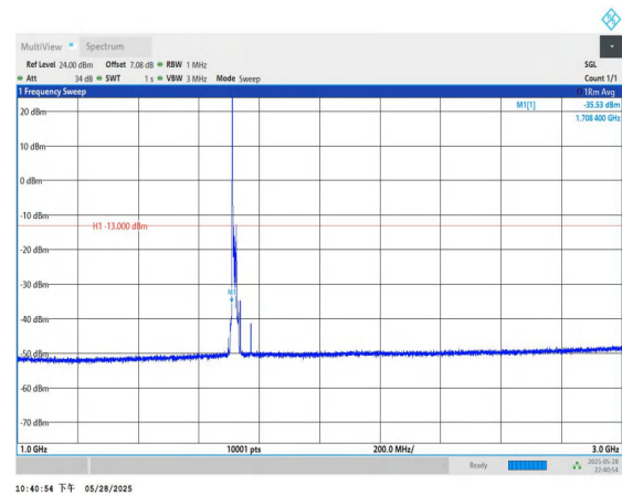
Band66-15MHz-QPSK-132047-1RB#0-1000~3000-PASS
