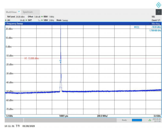
Band66-5MHz-QPSK-131997-1RB#0-1000~3000-PASS
