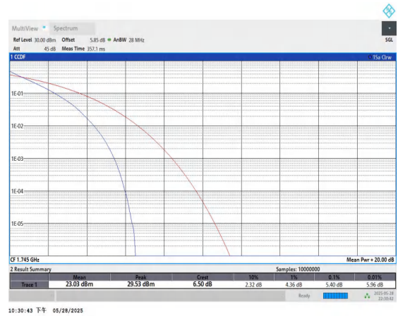
Band66-10MHz-QPSK-132322-50RB#0-PASS
