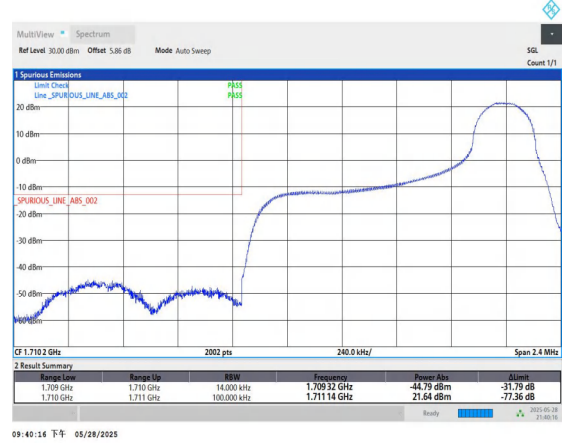
Band66-1.4MHz-QPSK-131979-1RB#5-PASS
