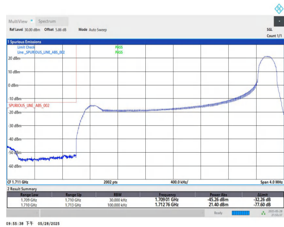
Band66-3MHz-QPSK-131987-1RB#14-PASS
