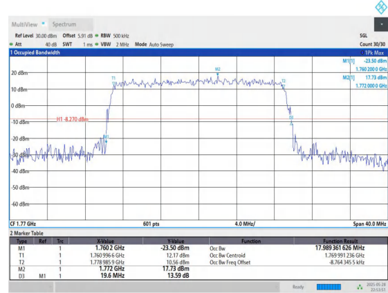
Band66-20MHz-16QAM-132572-100RB#0-PASS
