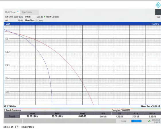
Band66-1.4MHz-QPSK-132322-6RB#0-PASS
