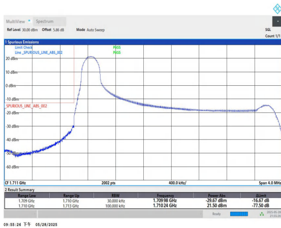
Band66-3MHz-QPSK-131987-1RB#0-PASS
