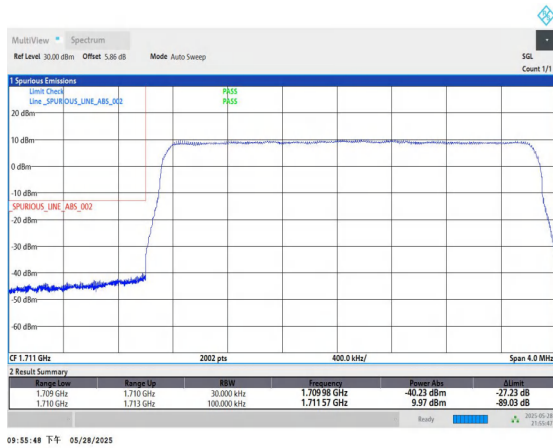
Band66-3MHz-QPSK-131987-15RB#0-PASS
