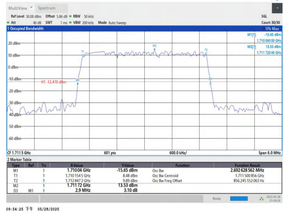
Band66-3MHz-16QAM-131987-15RB#0-PASS
