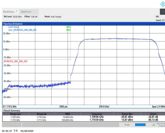
Band66-1.4MHz-QPSK-131979-6RB#0-PASS
