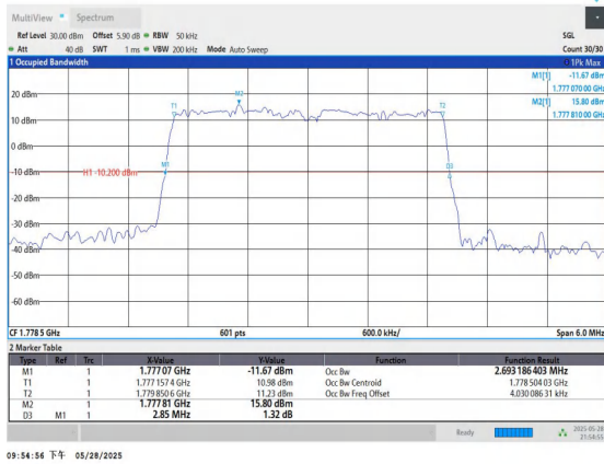
Band66-3MHz-QPSK-132657-15RB#0-PASS
