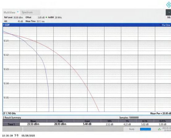
Band66-10MHz-QPSK-132322-1RB#0-PASS
