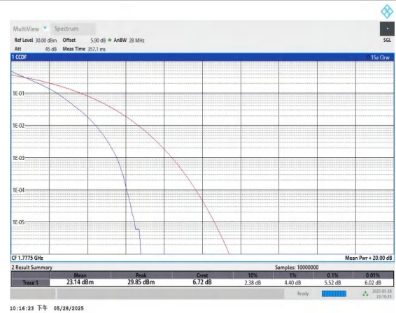
Band66-5MHz-QPSK-132647-25RB#0-PASS
