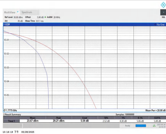
Band66-5MHz-QPSK-132647-1RB#0-PASS
