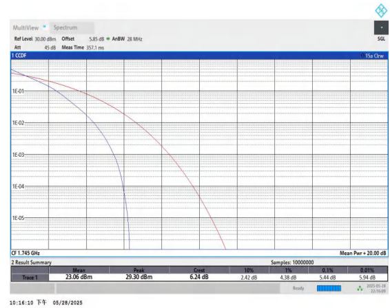
Band66-5MHz-QPSK-132322-25RB#0-PASS
