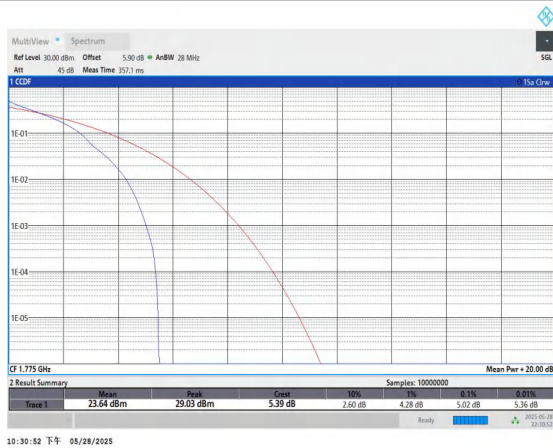
Band66-10MHz-QPSK-132622-1RB#0-PASS
