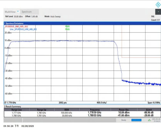
Band66-3MHz-QPSK-132657-15RB#0-PASS
