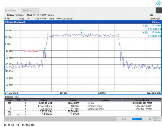
Band66-15MHz-16QAM-132597-75RB#0-PASS
