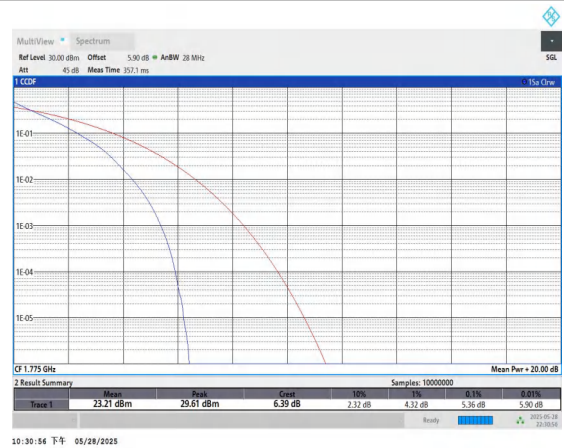
Band66-10MHz-QPSK-132622-50RB#0-PASS
