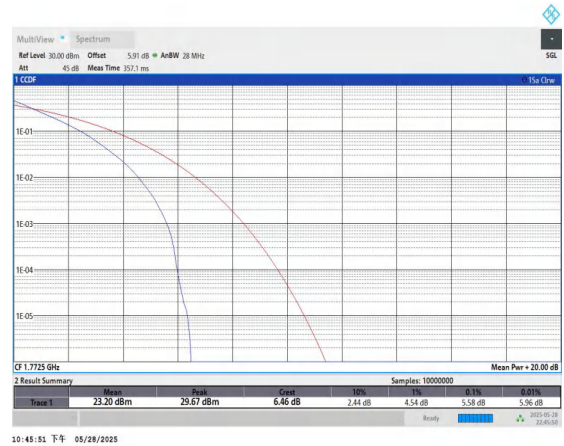
Band66-15MHz-QPSK-132597-75RB#0-PASS
