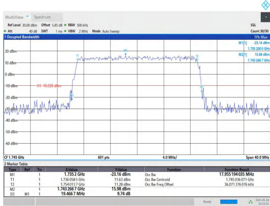
Band66-20MHz-16QAM-132322-100RB#0-PASS
