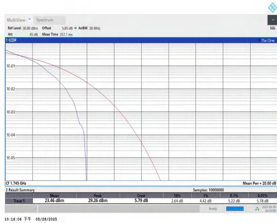
Band66-5MHz-QPSK-132322-1RB#0-PASS
