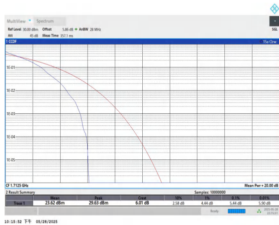
Band66-5MHz-QPSK-131997-1RB#0-PASS
