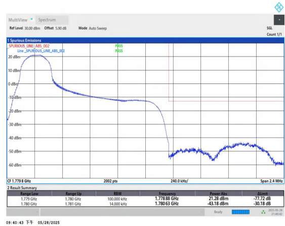
Band66-1.4MHz-QPSK-132665-1RB#0-PASS
