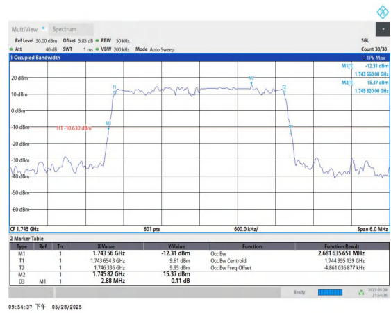
Band66-3MHz-QPSK-132322-15RB#0-PASS
