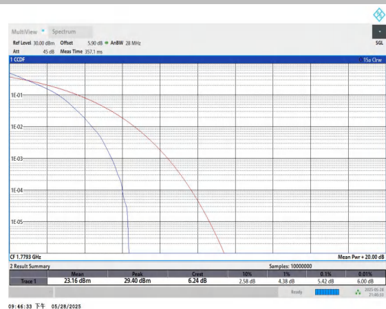
Band66-1.4MHz-QPSK-132665-6RB#0-PASS
