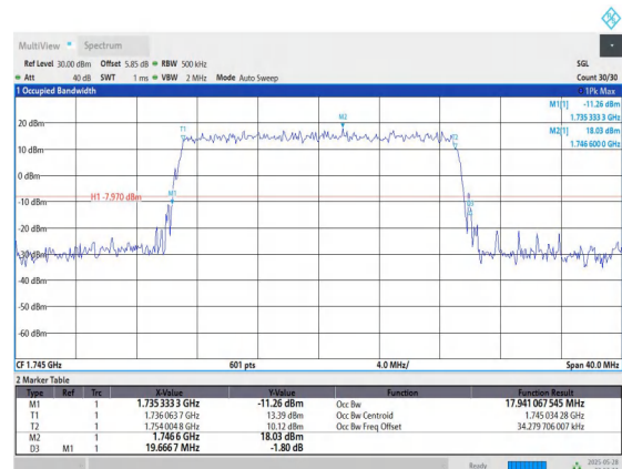
Band66-20MHz-QPSK-132322-100RB#0-PASS
