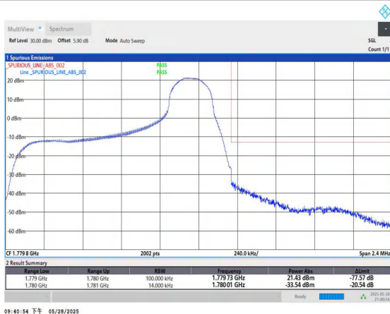
Band66-1.4MHz-QPSK-132665-1RB#5-PASS
