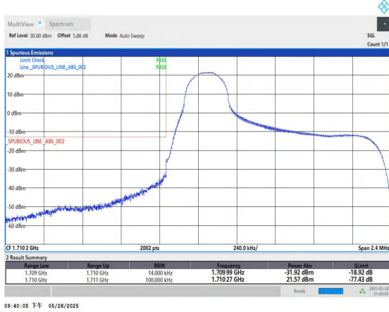
Band66-1.4MHz-QPSK-131979-1RB#0-PASS
