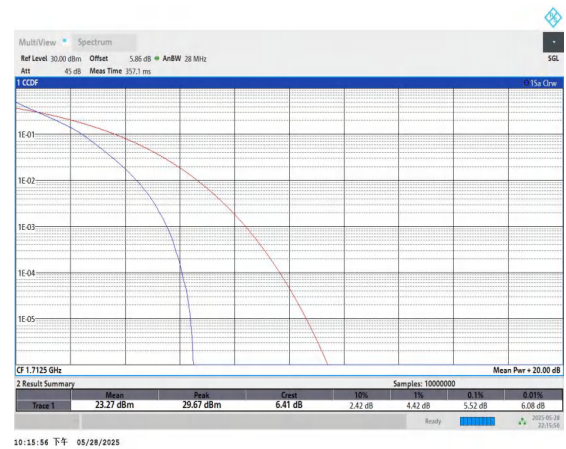
Band66-5MHz-QPSK-131997-25RB#0-PASS
