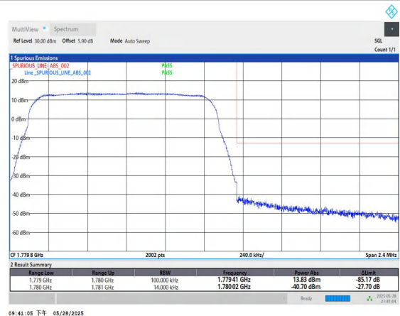
Band66-1.4MHz-QPSK-132665-6RB#0-PASS
