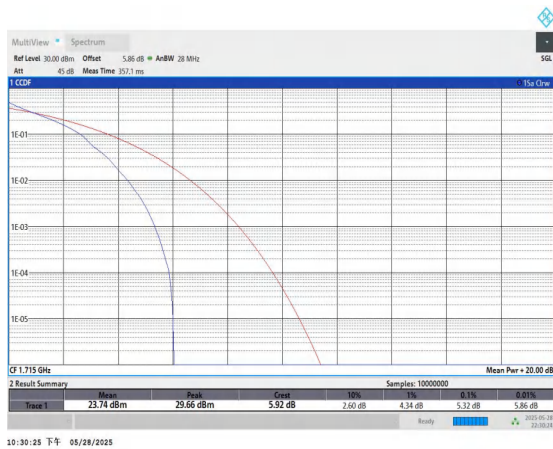
Band66-10MHz-QPSK-132022-1RB#0-PASS
