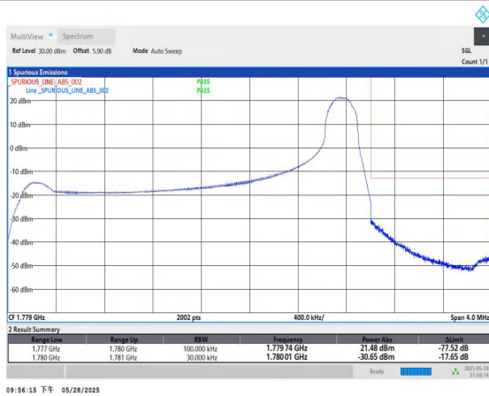
Band66-3MHz-QPSK-132657-1RB#14-PASS
