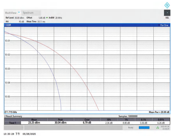
Band66-10MHz-QPSK-132022-50RB#0-PASS
