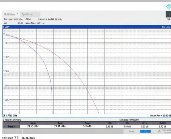
Band66-1.4MHz-QPSK-132665-1RB#0-PASS
