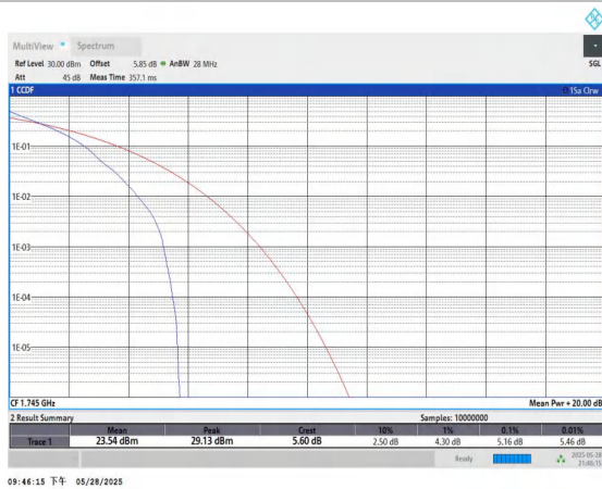
Band66-1.4MHz-QPSK-132322-1RB#0-PASS
