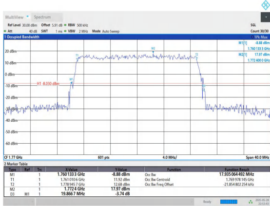
Band66-20MHz-QPSK-132572-100RB#0-PASS
