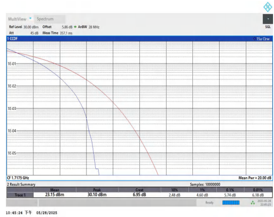
Band66-15MHz-QPSK-132047-75RB#0-PASS
