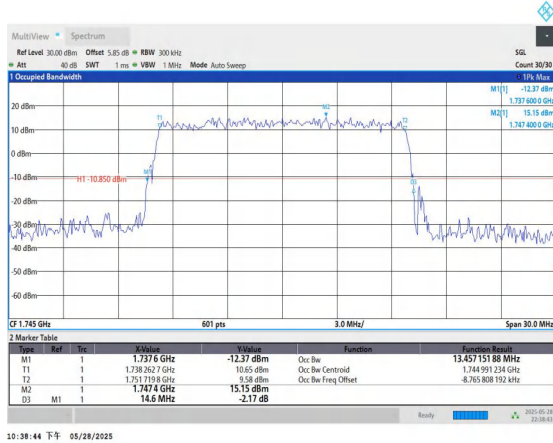
Band66-15MHz-16QAM-132322-75RB#0-PASS
