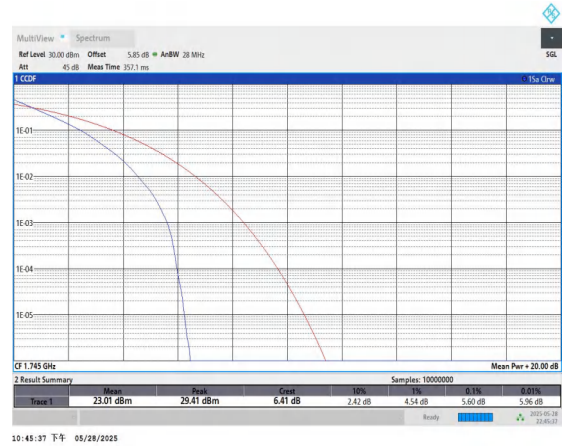
Band66-15MHz-QPSK-132322-75RB#0-PASS
