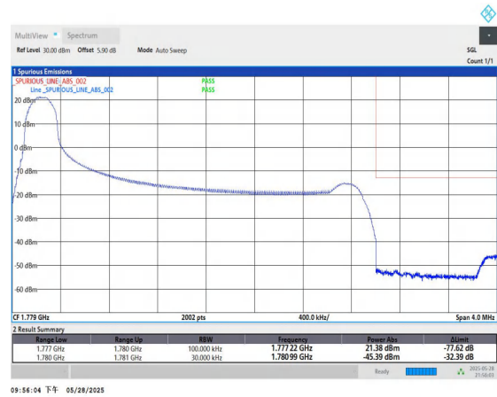
Band66-3MHz-QPSK-132657-1RB#0-PASS
