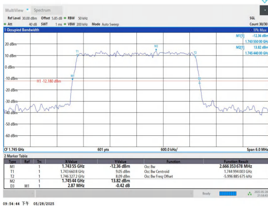
Band66-3MHz-16QAM-132322-15RB#0-PASS
