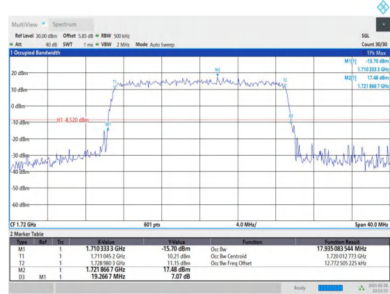
Band66-20MHz-16QAM-132072-100RB#0-PASS
