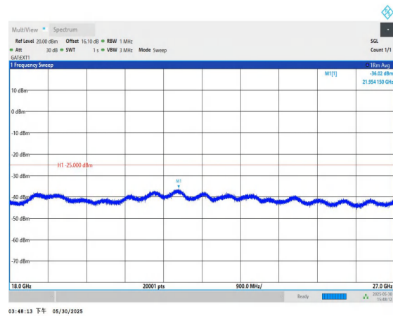
Band41-15MHz-QPSK-40620-1RB#0-18000~27000-PASS
