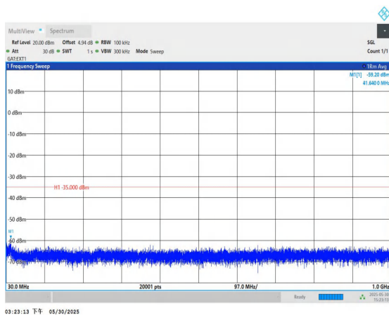
Band41-10MHz-QPSK-39700-1RB#0-30~1000-PASS
