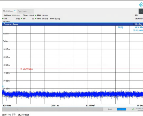
Band41-15MHz-QPSK-40620-1RB#0-30~1000-PASS
