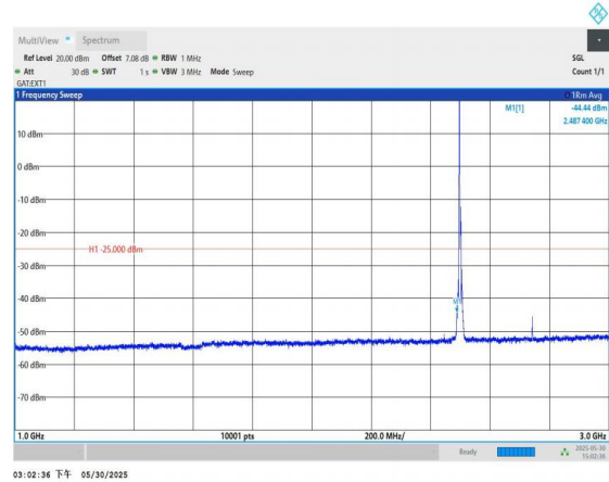
Band41-5MHz-QPSK-39675-1RB#0-1000~3000-PASS
