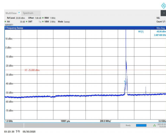
Band41-10MHz-QPSK-39700-1RB#0-1000~3000-PASS
