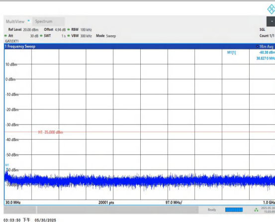
Band41-5MHz-QPSK-40620-1RB#0-30~1000-PASS
