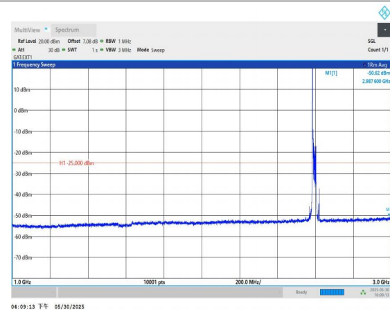
Band41-20MHz-QPSK-40620-1RB#0-1000~3000-PASS
