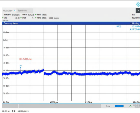
Band41-5MHz-QPSK-39675-1RB#0-3000~18000-PASS
