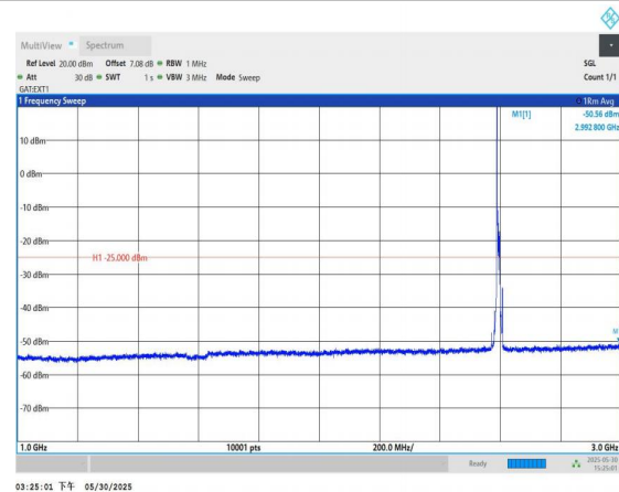
Band41-10MHz-QPSK-40620-1RB#0-1000~3000-PASS
