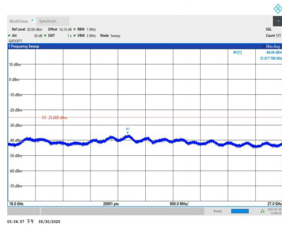
Band41-5MHz-QPSK-40620-1RB#0-18000~27000-PASS
