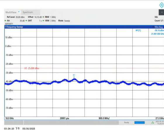
Band41-10MHz-QPSK-39700-1RB#0-18000~27000-PASS
