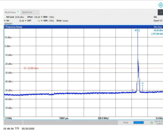
Band41-15MHz-QPSK-41515-1RB#0-1000~3000-PASS
