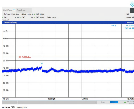
Band41-20MHz-QPSK-40620-1RB#0-3000~18000-PASS
