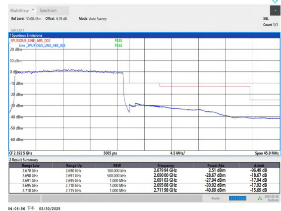
Band41-20MHz-QPSK-41490-100RB#0-PASS
