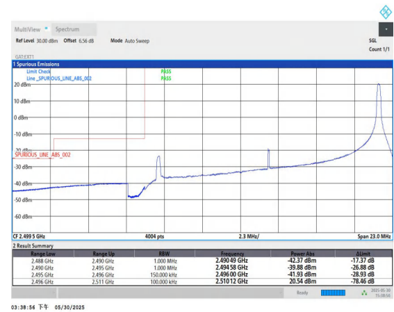
Band41-15MHz-QPSK-39725-1RB#74-PASS
