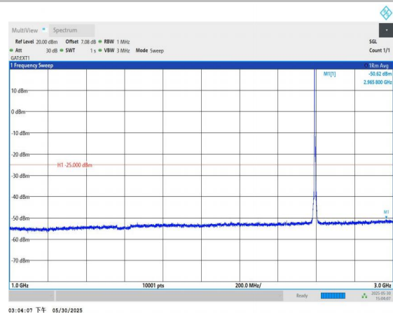
Band41-5MHz-QPSK-40620-1RB#0-1000~3000-PASS
