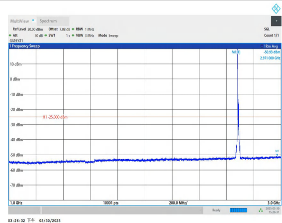
Band41-10MHz-QPSK-41540-1RB#0-1000~3000-PASS
