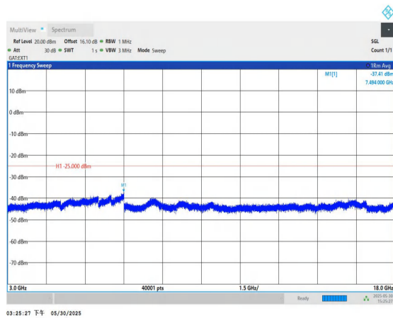
Band41-10MHz-QPSK-40620-1RB#0-3000~18000-PASS
