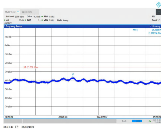
Band41-15MHz-QPSK-41515-1RB#0-18000~27000-PASS
