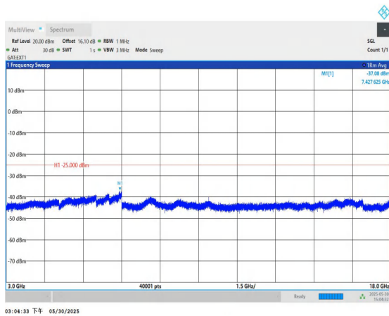
Band41-5MHz-QPSK-40620-1RB#0-3000~18000-PASS
