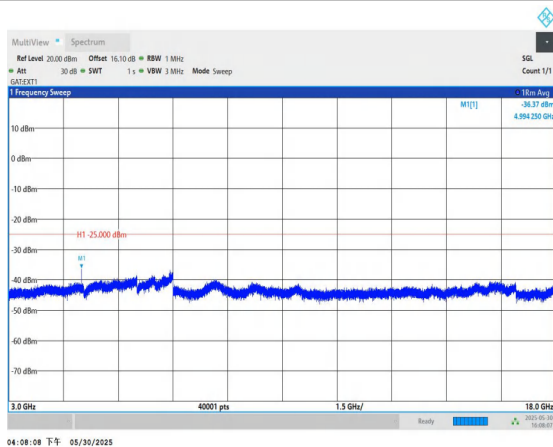
Band41-20MHz-QPSK-39750-1RB#0-3000~18000-PASS
