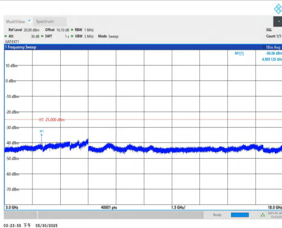
Band41-10MHz-QPSK-39700-1RB#0-3000~18000-PASS
