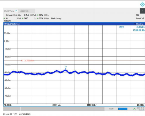
Band41-5MHz-QPSK-39675-1RB#0-18000~27000-PASS
