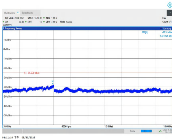
Band41-20MHz-QPSK-41490-1RB#0-3000~18000-PASS
