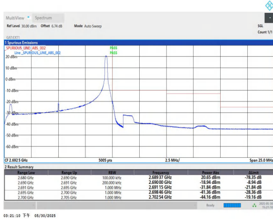
Band41-10MHz-QPSK-41540-1RB#49-PASS
