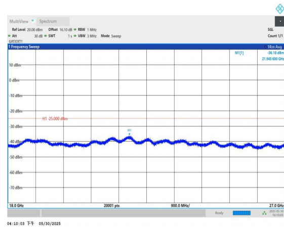
Band41-20MHz-QPSK-40620-1RB#0-18000~27000-PASS
