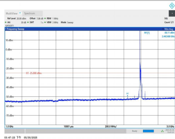
Band41-15MHz-QPSK-40620-1RB#0-1000~3000-PASS
