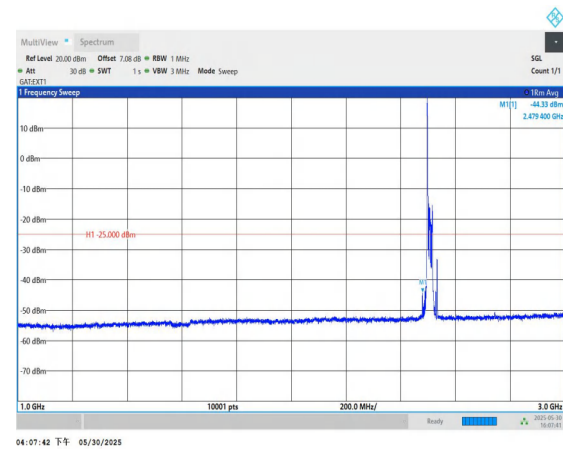
Band41-20MHz-QPSK-39750-1RB#0-1000~3000-PASS
