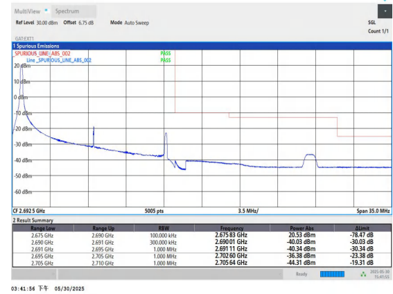
Band41-15MHz-QPSK-41515-1RB#0-PASS
