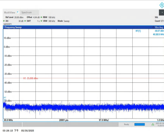
Band41-10MHz-QPSK-41540-1RB#0-30~1000-PASS
