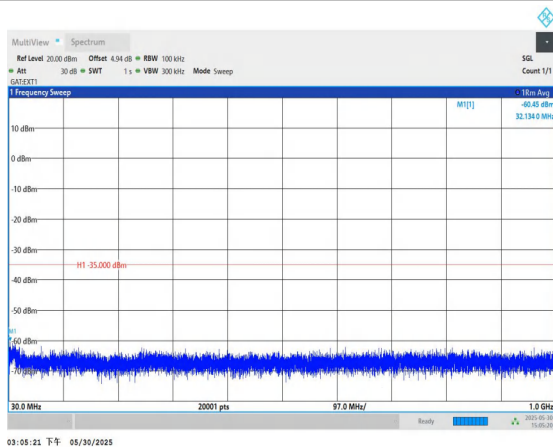
Band41-5MHz-QPSK-41565-1RB#0-30~1000-PASS
