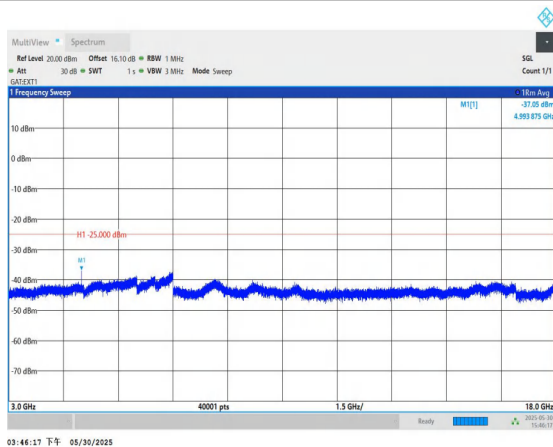
Band41-15MHz-QPSK-39725-1RB#0-3000~18000-PASS
