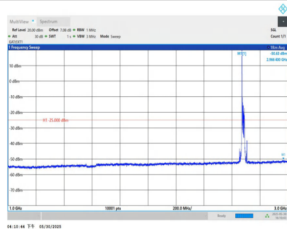
Band41-20MHz-QPSK-41490-1RB#0-1000~3000-PASS
