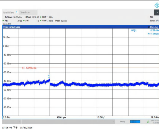
Band41-5MHz-QPSK-41565-1RB#0-3000~18000-PASS
