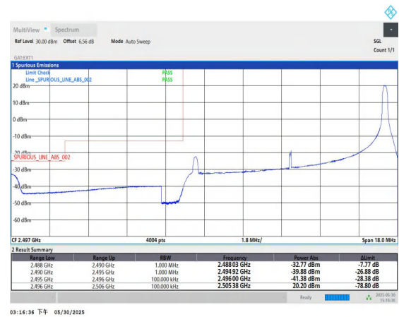
Band41-10MHz-QPSK-39700-1RB#49-PASS
