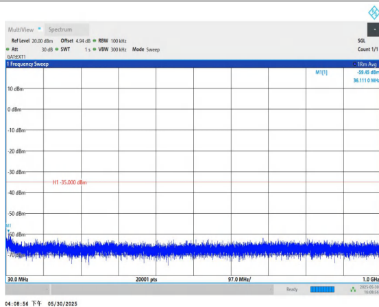
Band41-20MHz-QPSK-40620-1RB#0-30~1000-PASS
