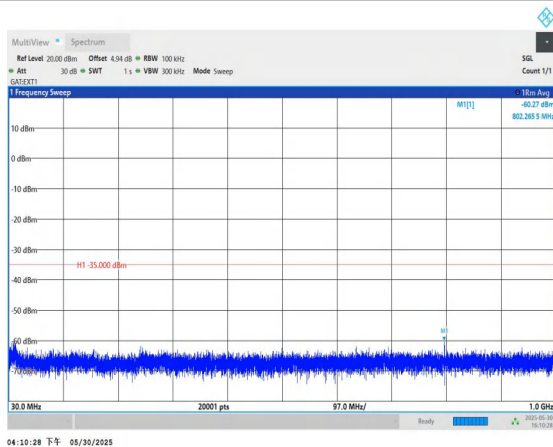
Band41-20MHz-QPSK-41490-1RB#0-30~1000-PASS
