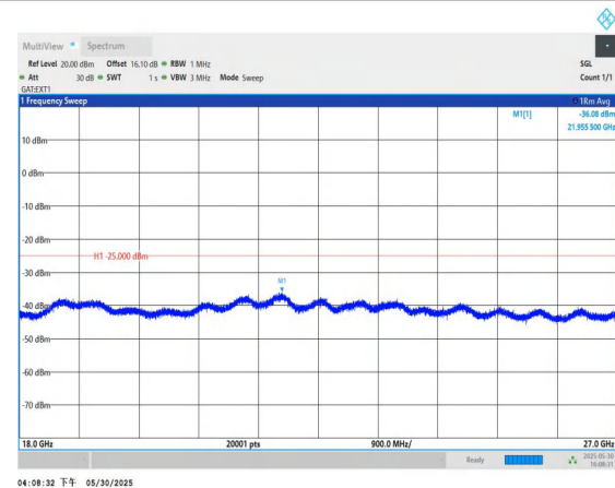
Band41-20MHz-QPSK-39750-1RB#0-18000~27000-PASS
