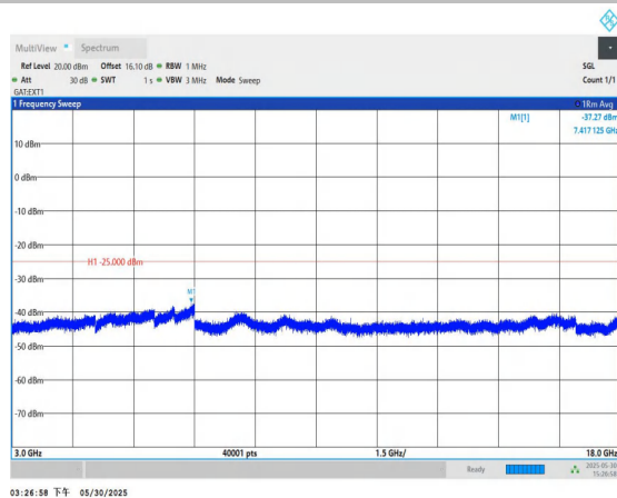
Band41-10MHz-QPSK-41540-1RB#0-3000~18000-PASS
