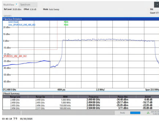
Band41-15MHz-QPSK-39725-75RB#0-PASS
