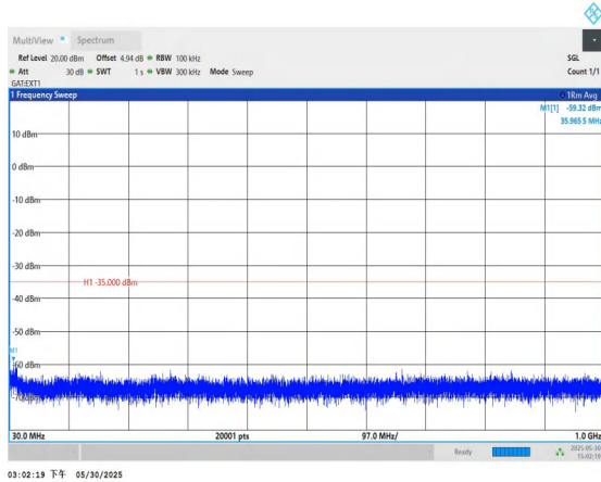
Band41-5MHz-QPSK-39675-1RB#0-30~1000-PASS
