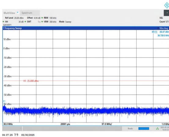
Band41-20MHz-QPSK-39750-1RB#0-30~1000-PASS
