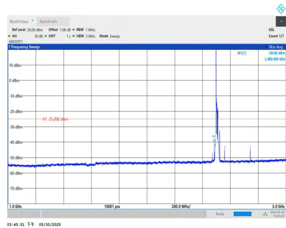
Band41-15MHz-QPSK-39725-1RB#0-1000~3000-PASS
