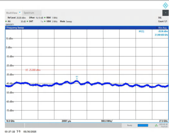
Band41-10MHz-QPSK-41540-1RB#0-18000~27000-PASS
