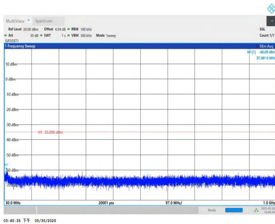
Band41-15MHz-QPSK-39725-1RB#0-30~1000-PASS
