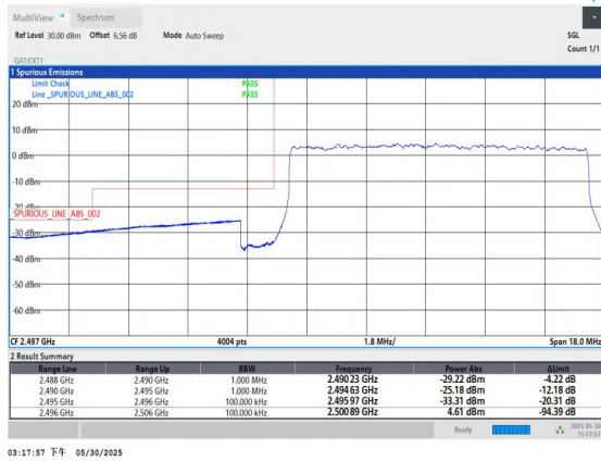
Band41-10MHz-QPSK-39700-50RB#0-PASS
