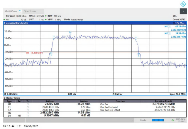
Band41-10MHz-16QAM-41540-50RB#0-PASS
