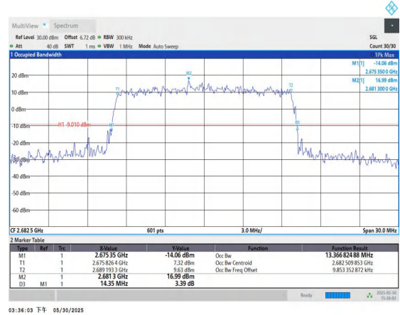
Band41-15MHz-16QAM-41515-75RB#0-PASS
