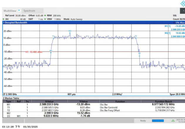
Band41-10MHz-16QAM-40620-50RB#0-PASS
