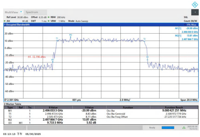
Band41-10MHz-16QAM-39700-50RB#0-PASS
