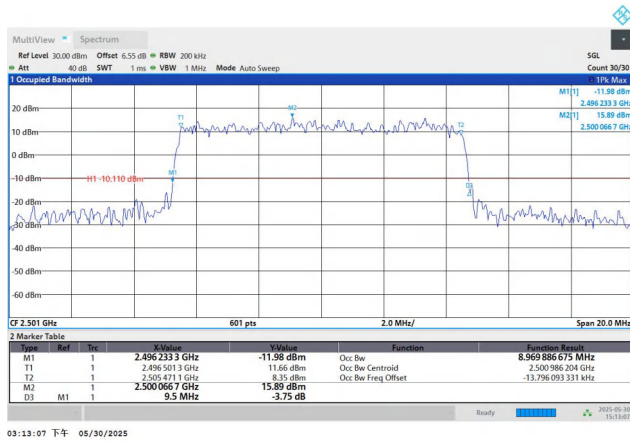
Band41-10MHz-QPSK-39700-50RB#0-PASS
