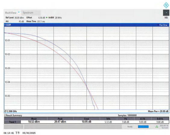
Band41-20MHz-QPSK-39750-100RB#0-PASS
