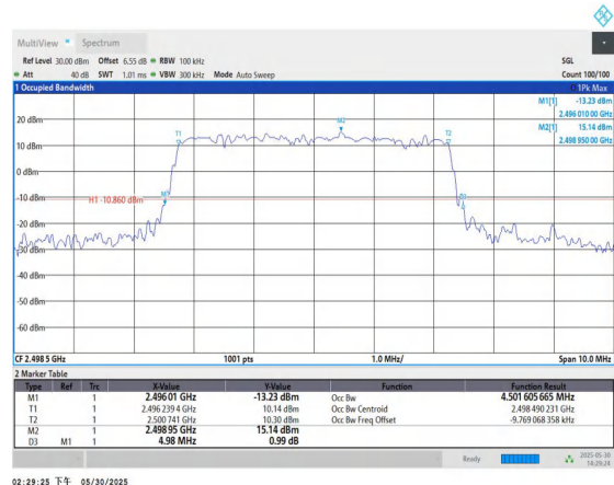
Band41-5MHz-16QAM-39675-25RB#0-PASS
