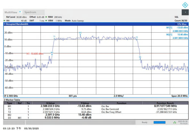
Band41-10MHz-QPSK-40620-50RB#0-PASS
