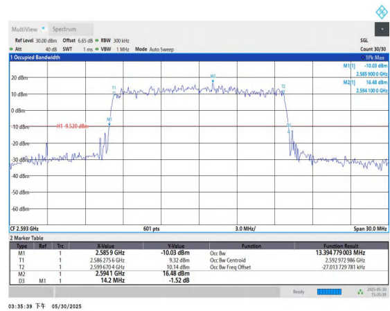
Band41-15MHz-QPSK-40620-75RB#0-PASS
