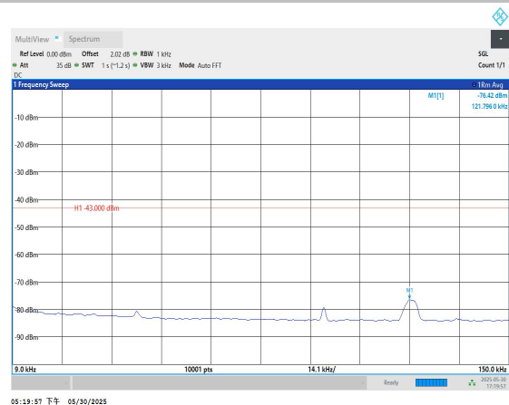
Band2-9400-0.009~0.15MHz-PASS
