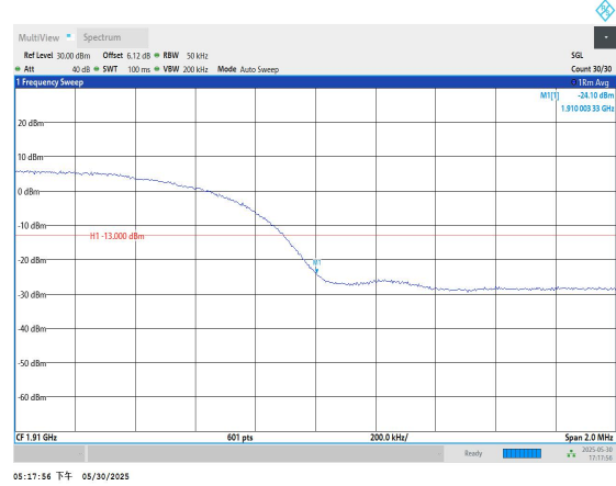
Band2-9538-PASS
