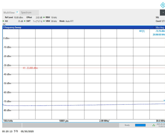
Band2-9400-0.15~30MHz-PASS
