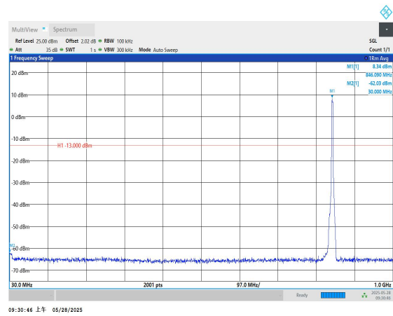
Band5-4233-30~1000MHz-PASS
