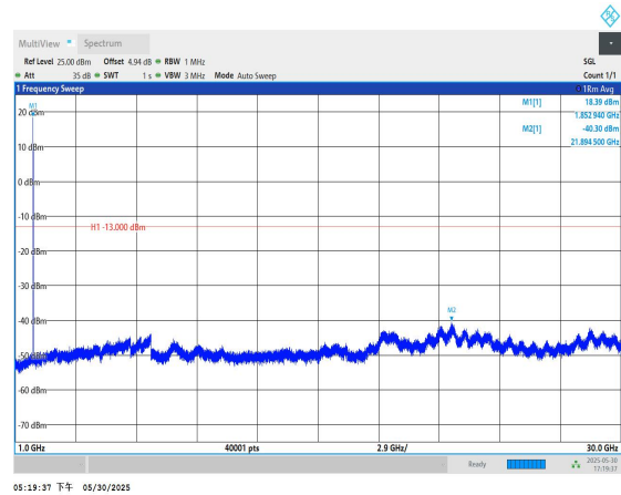
Band2-9262-1000~30000MHz-PASS
