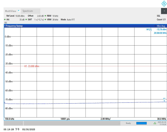
Band2-9262-0.15~30MHz-PASS
