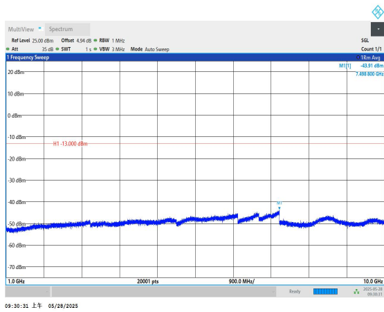
Band5-4182-1000~10000MHz-PASS
