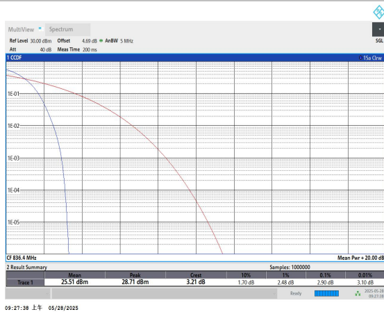
Band5-4182-PASS
