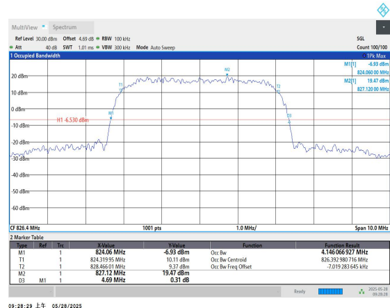
Band5-4132-PASS
