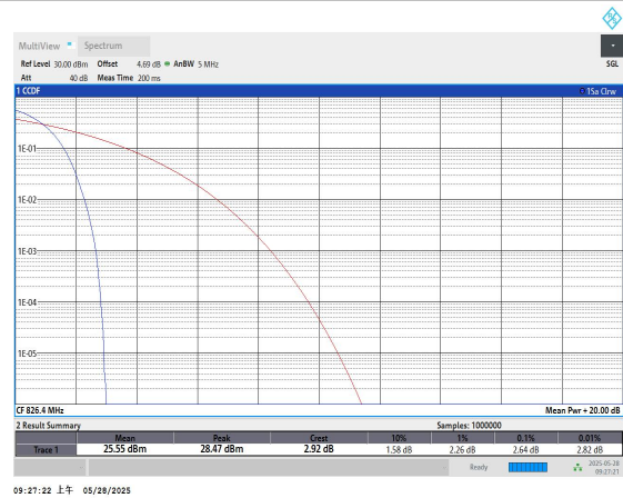
Band5-4132-PASS
