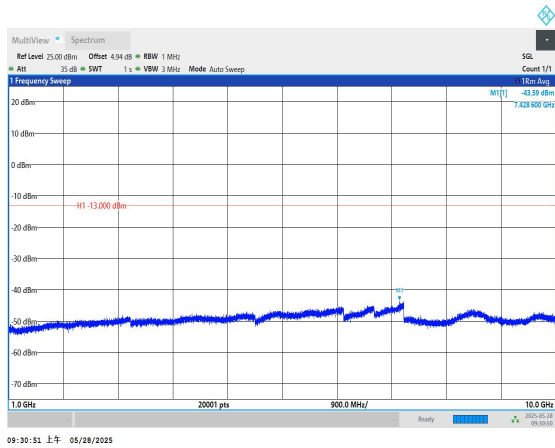
Band5-4233-1000~10000MHz-PASS
