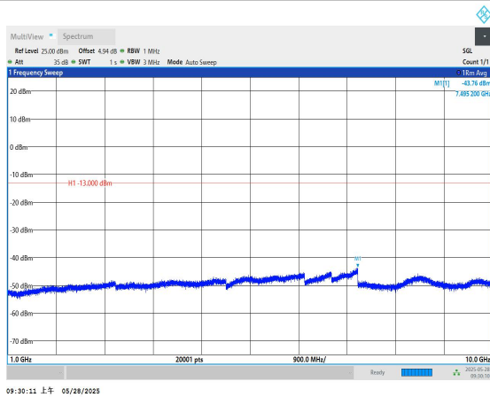
Band5-4132-1000~10000MHz-PASS
