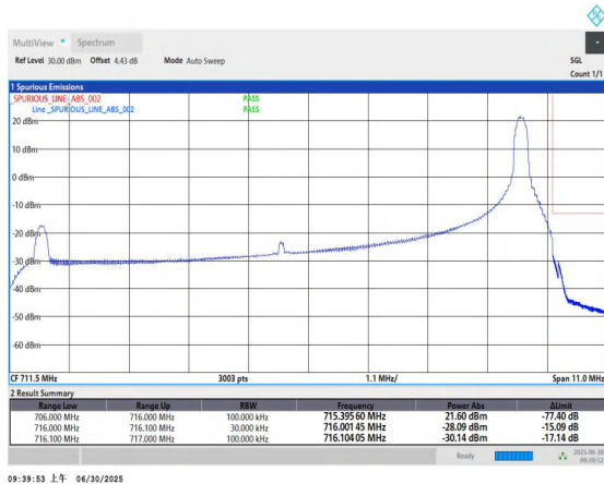
Band12-10MHz-QPSK-23130-1RB#49-PASS
