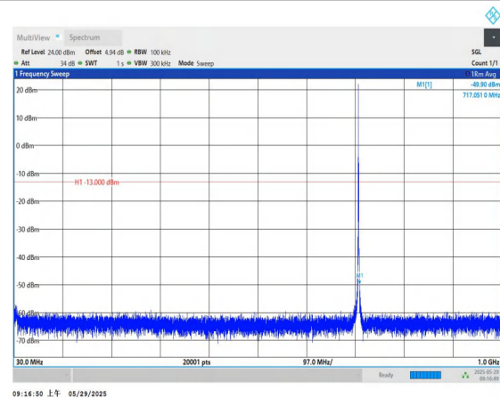
Band12-1.4MHz-16QAM-23173-1RB#0-30~1000-PASS
