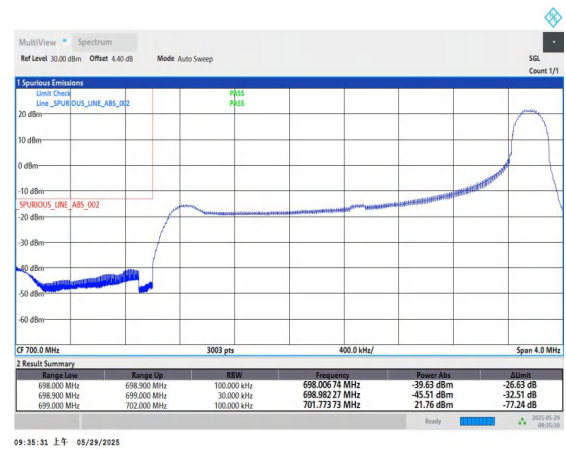
Band12-3MHz-16QAM-23025-1RB#14-PASS
