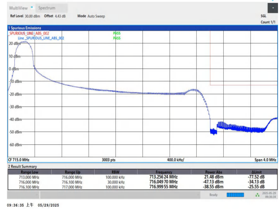
Band12-3MHz-16QAM-23165-1RB#0-PASS
