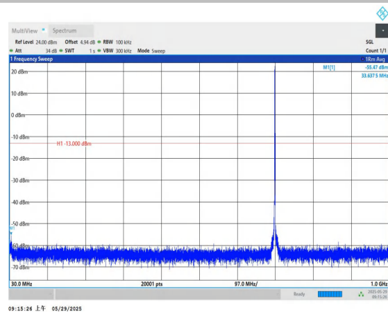
Band12.14MHz-QPSK-23095-1RB#0-30~1000-PASS
