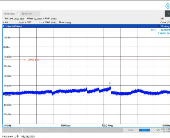
Band12.14MHz-QPSK-23017-1RB#0-3000~10000-PASS
