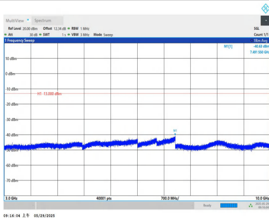
Band12-1.4MHz-16QAM-23095-1RB#0-3000~10000-PASS
