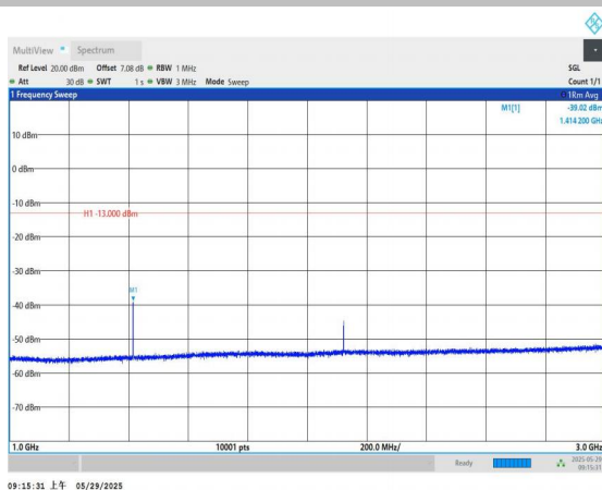
Band12.14MHz-QPSK-23095-1RB#0-1000~3000-PASS
