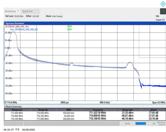
Band12-5MHz-QPSK-23155-1RB#0-PASS
