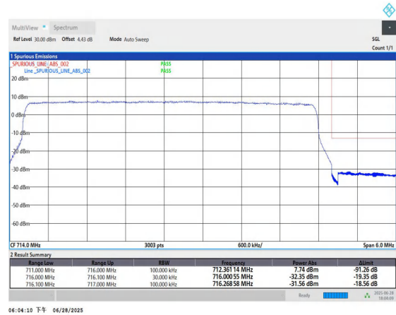
Band12-5MHz-QPSK-23155-25RB#0-PASS
