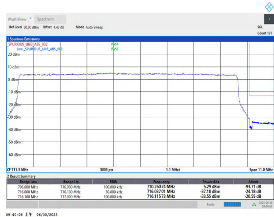
Band12-10MHz-QPSK-23130-50RB#0-PASS
