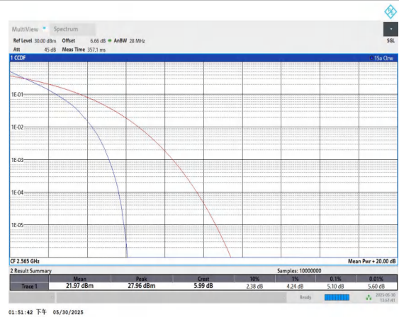
Band7-10MHz-QPSK-21400-50RB#0-PASS
