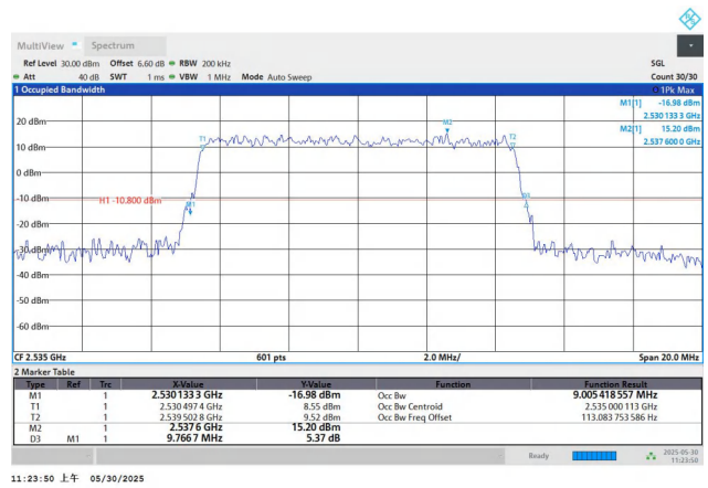
Band7-10MHz-QPSK-21100-50RB#0-PASS
