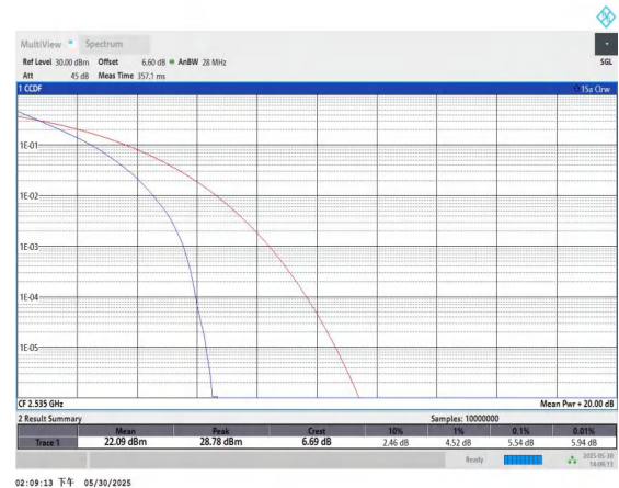
Band7-15MHz-QPSK-21100-75RB#0-PASS
