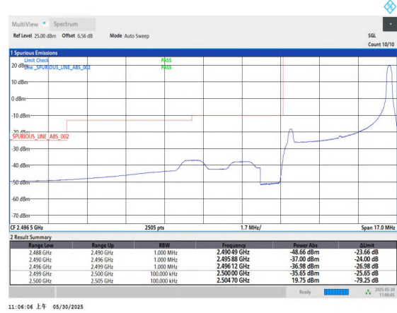
Band7-5MHz-QPSK-20775-1RB#24-PASS
