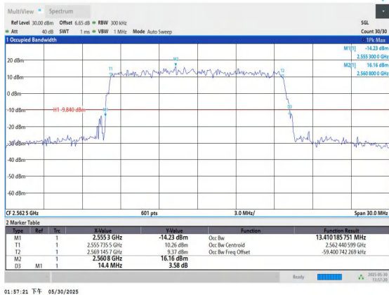
Band7-15MHz-QPSK-21375-75RB#0-PASS
