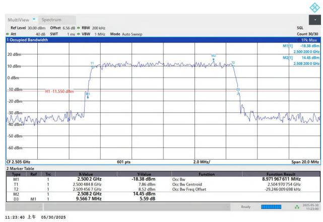
Band7-10MHz-16QAM-20800-50RB#0-PASS
