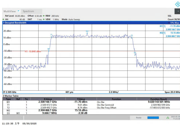
Band7-10MHz-QPSK-20800-50RB#0-PASS
