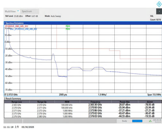
Band7-5MHz-QPSK-21425-1RB#0-PASS
