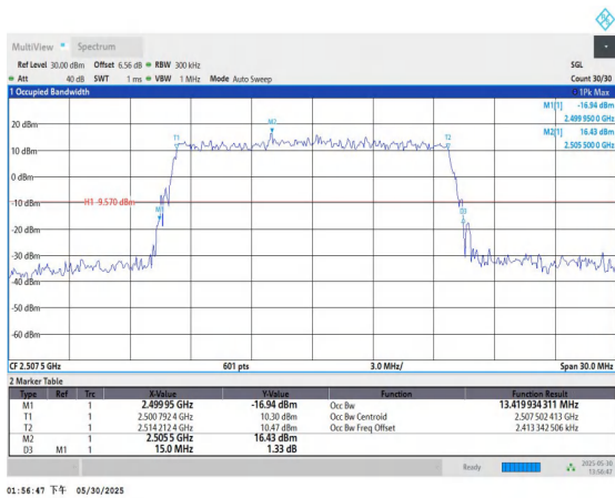
Band7-15MHz-QPSK-20825-75RB#0-PASS
