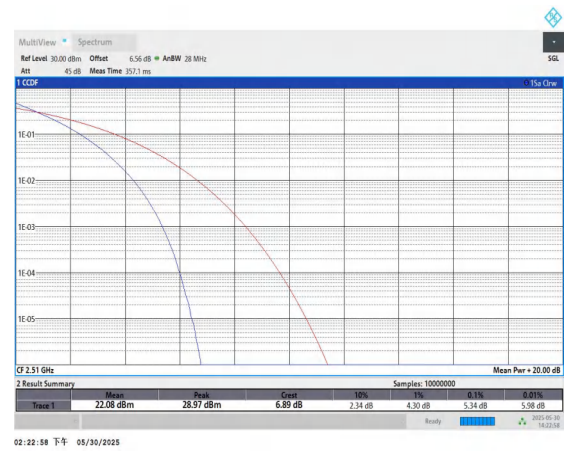
Band7-20MHz-QPSK-20850-100RB#0-PASS
