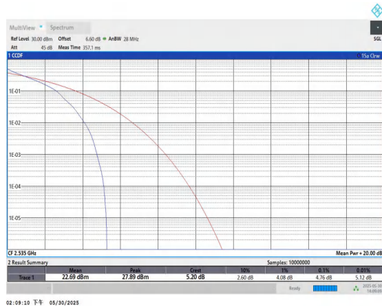
Band7-15MHz-QPSK-21100-1RB#0-PASS
