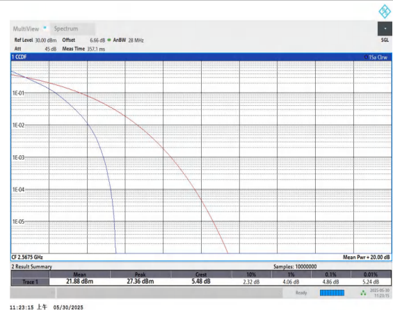
Band7-5MHz-QPSK-21425-25RB#0-PASS
