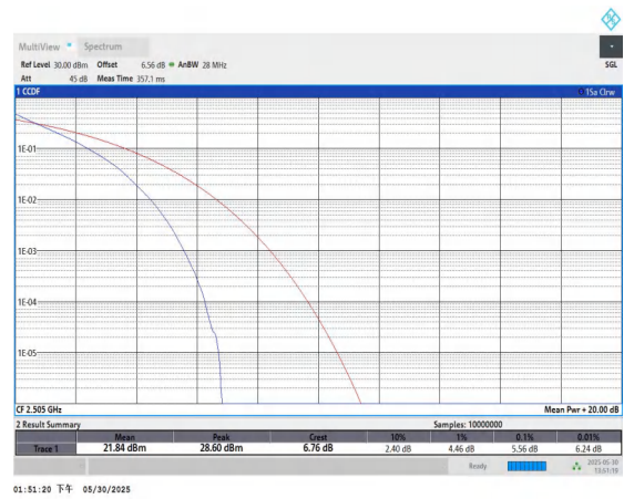
Band7-10MHz-QPSK-20800-50RB#0-PASS
