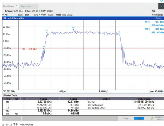
Band7-15MHz-16QAM-21100-75RB#0-PASS
