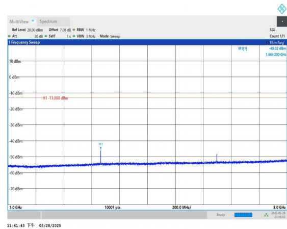
Band5-10MHz-QPSK-20525-1RB#0-1000~3000-PASS
