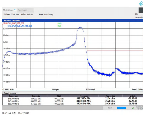
Band5-3MHz-QPSK-20635-1RB#14-PASS
