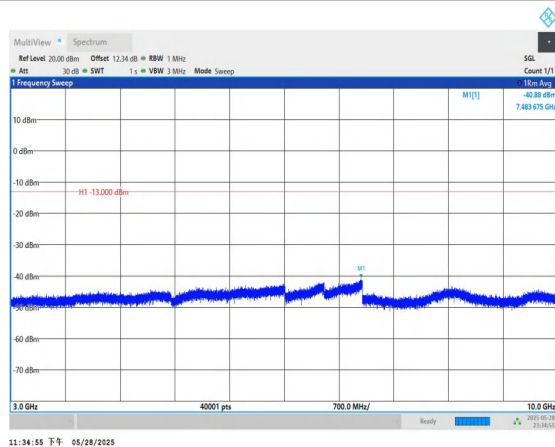
Band5-1.4MHz-QPSK-20643-1RB#0-3000~10000-PASS
