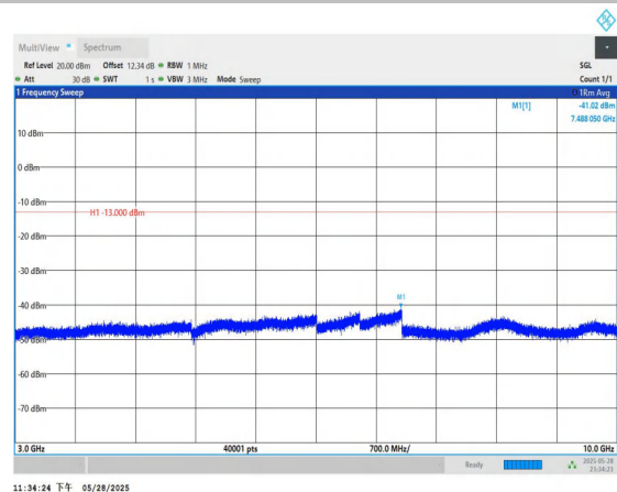
Band5-1.4MHz-QPSK-20525-1RB#0-3000~10000-PASS
