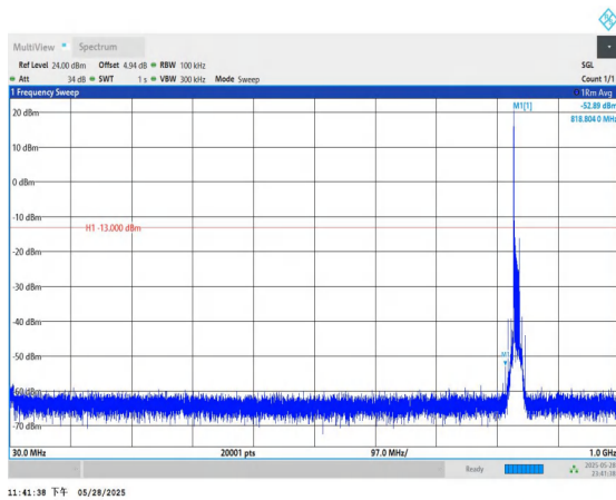
Band5-10MHz-QPSK-20525-1RB#0-30~1000-PASS
