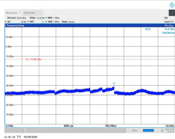
Band5-10MHz-QPSK-20450-1RB#0-3000~10000-PASS
