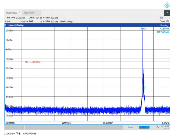
Band5-10MHz-QPSK-20600-1RB#0-30~1000-PASS
