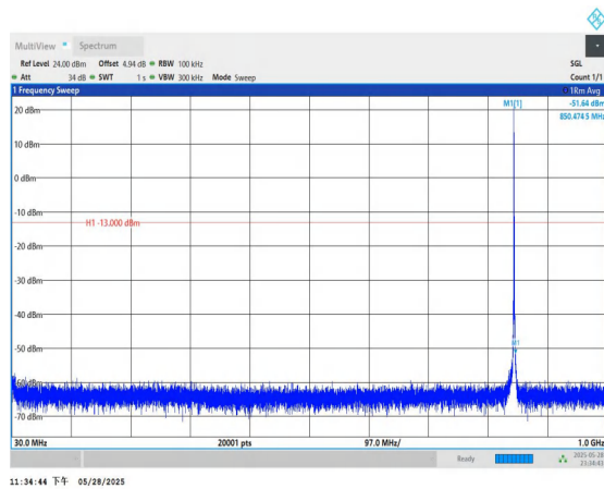
Band5-1.4MHz-QPSK-20643-1RB#0-30~1000-PASS
