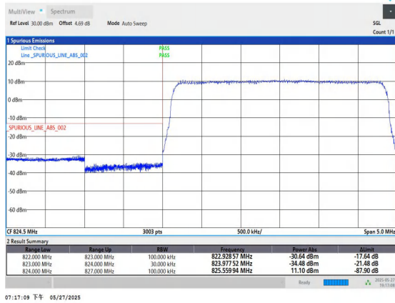
Band5-3MHz-QPSK-20415-15RB#0-PASS
