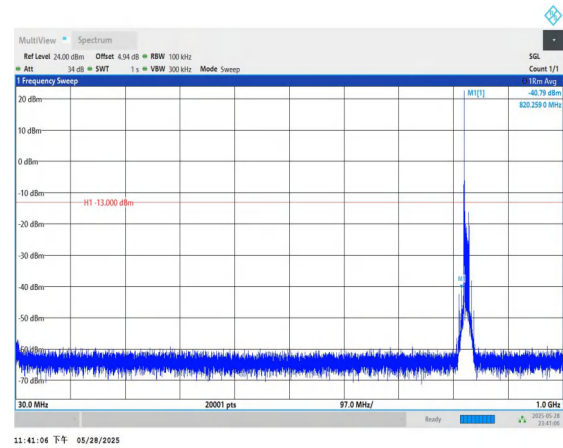
Band5-10MHz-QPSK-20450-1RB#0-30~1000-PASS
