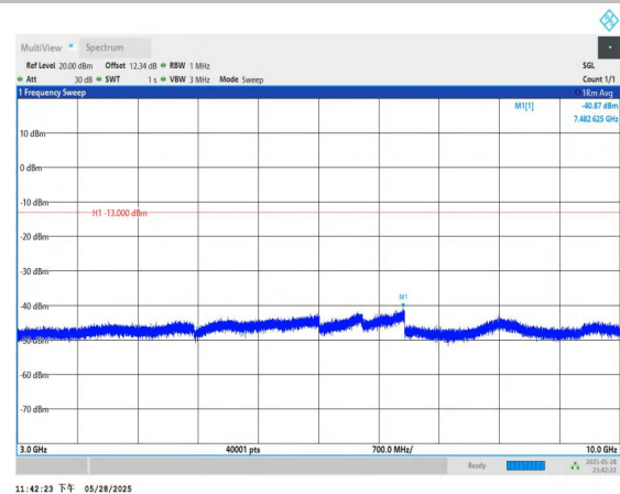
Band5-10MHz-QPSK-20600-1RB#0-3000~10000-PASS
