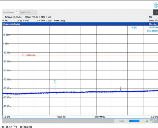
Band5-1.4MHz-QPSK-20525-1RB#0-1000~3000-PASS
