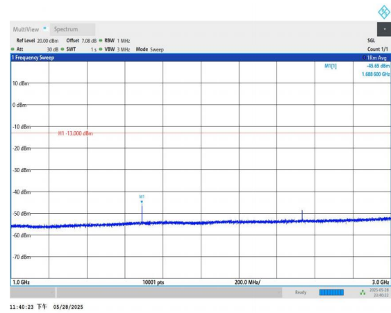
Band5-5MHz-QPSK-20625-1RB#0-1000~3000-PASS
