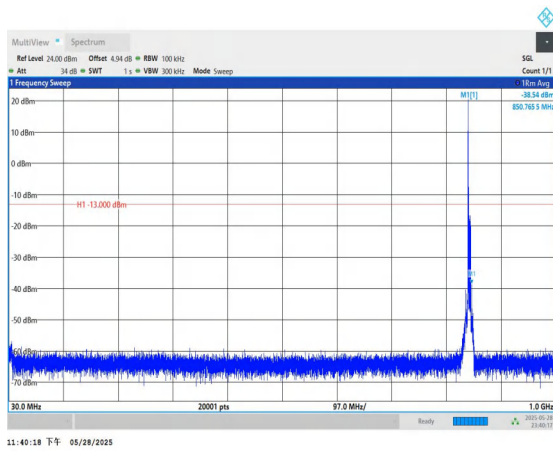
Band5-5MHz-QPSK-20625-1RB#0-30~1000-PASS
