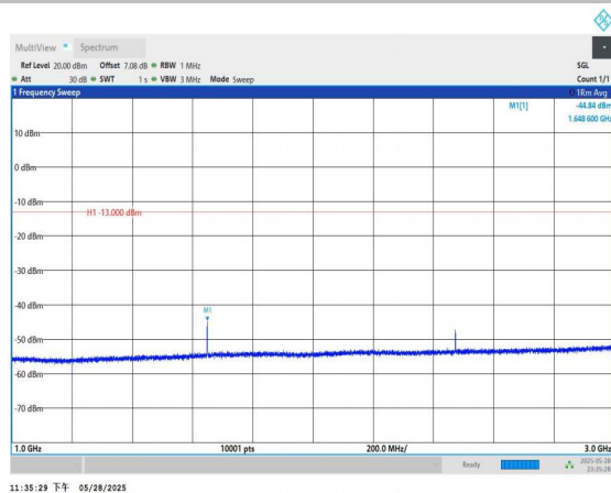
Band5-3MHz-QPSK-20415-1RB#0-1000~3000-PASS
