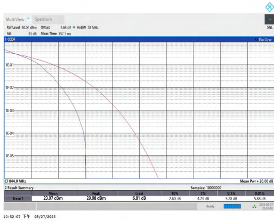
Band5-10MHz-QPSK-20600-1RB#0-PASS
