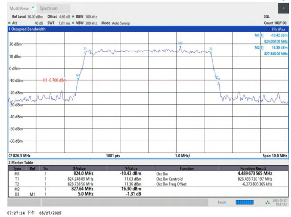
Band5-5MHz-16QAM-20425-25RB#0-PASS
