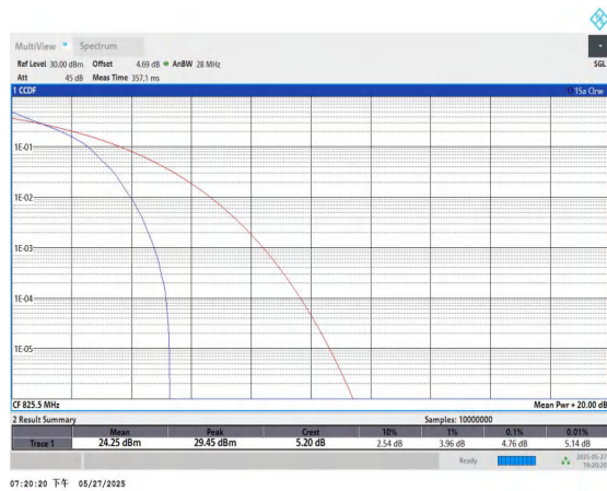
Band5-3MHz-QPSK-20415-1RB#0-PASS
