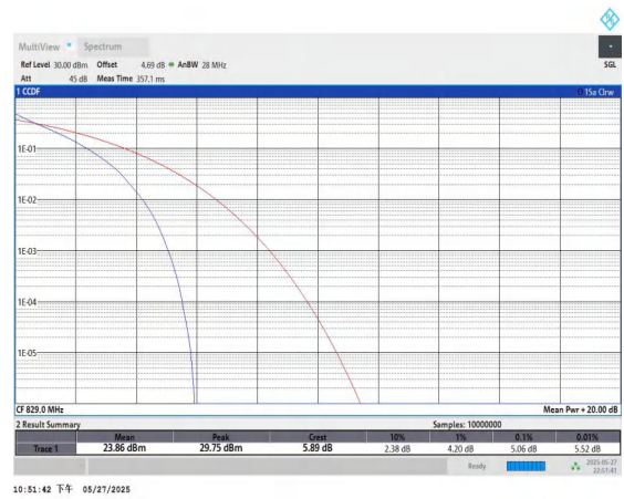
Band5-10MHz-QPSK-20450-50RB#0-PASS
