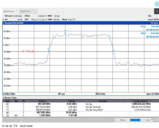
Band5-1.4MHz-QPSK-20643-6RB#0-PASS
