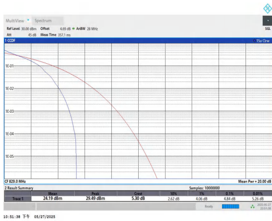
Band5-10MHz-QPSK-20450-1RB#0-PASS
