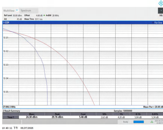
Band5-5MHz-QPSK-20625-1RB#0-PASS
