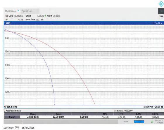
Band5-5MHz-QPSK-20525-25RB#0-PASS
