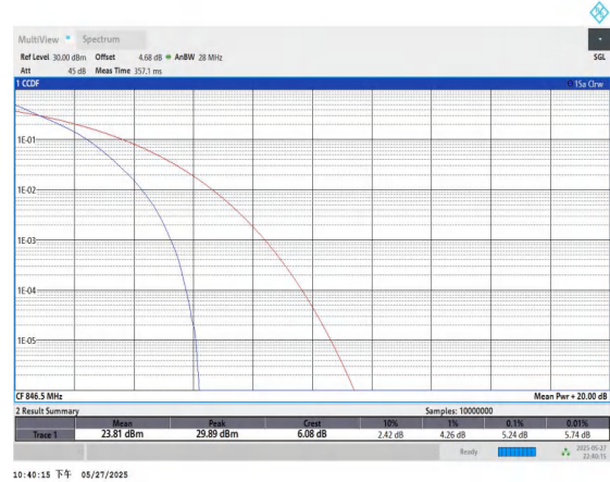
Band5-5MHz-QPSK-20625-25RB#0-PASS
