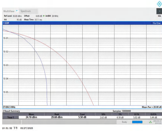
Band5-10MHz-QPSK-20525-1RB#0-PASS
