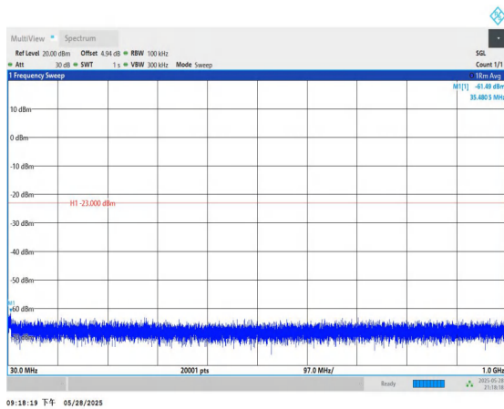
Band4-15MHz-QPSK-20025-1RB#0-30~1000-PASS
