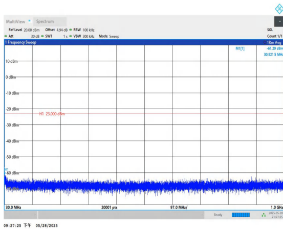
Band4-20MHz-QPSK-20175-1RB#0-30~1000-PASS
