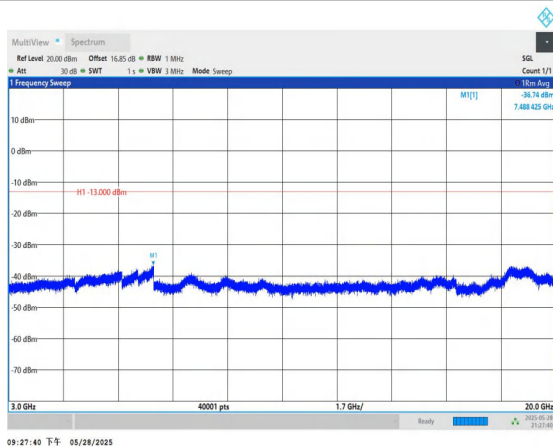
Band4-20MHz-QPSK-20175-1RB#0-3000~20000-PASS
