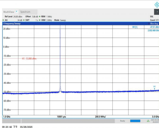
Band4-1.4MHz-QPSK-20175-1RB#0-1000~3000-PASS
