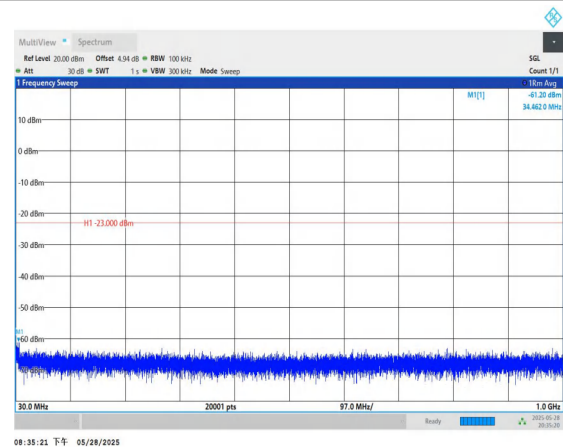
Band4-3MHz-QPSK-20385-1RB#0-30~1000-PASS
