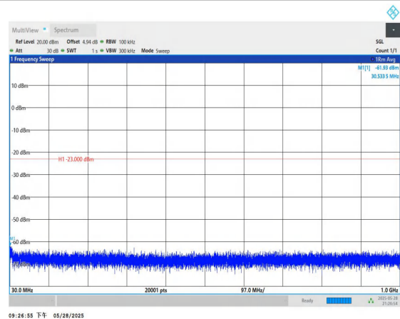
Band4-20MHz-QPSK-20050-1RB#0-30~1000-PASS
