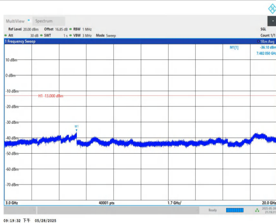
Band4-15MHz-QPSK-20325-1RB#0-3000~20000-PASS
