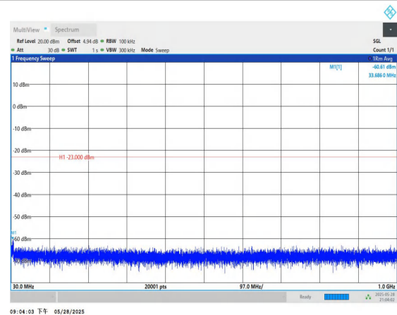
Band4-10MHz-QPSK-20350-1RB#0-30~1000-PASS
