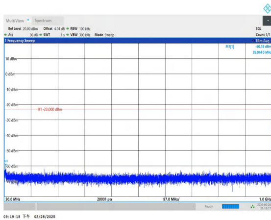
Band4-15MHz-QPSK-20325-1RB#0-30~1000-PASS
