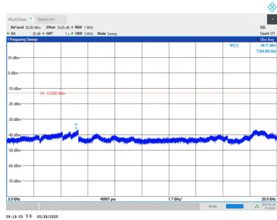
Band4-15MHz-QPSK-20175-1RB#0-3000~20000-PASS
