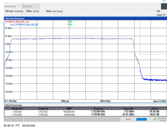
Band4-5MHz-QPSK-20375-25RB#0-PASS
