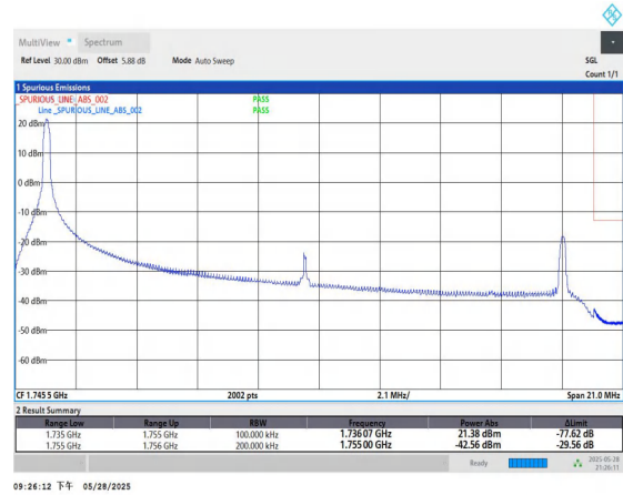
Band4-20MHz-QPSK-20300-1RB#0-PASS
