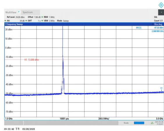
Band4-10MHz-QPSK-20175-1RB#0-1000~3000-PASS
