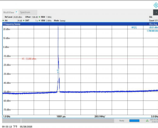
Band4-10MHz-QPSK-20000-1RB#0-1000~3000-PASS
