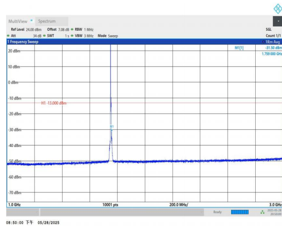
Band4-5MHz-QPSK-20375-1RB#0-1000~3000-PASS
