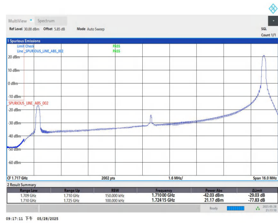
Band4-15MHz-QPSK-20025-1RB#74-PASS
