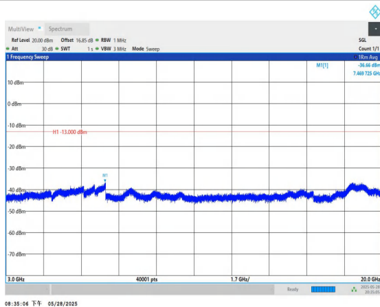
Band4-3MHz-QPSK-20175-1RB#0-3000~20000-PASS
