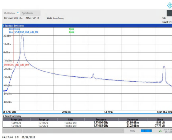
Band4-15MHz-QPSK-20025-1RB#0-PASS
