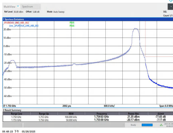
Band4-5MHz-QPSK-20375-1RB#24-PASS
