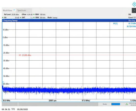
Band4-3MHz-QPSK-20175-1RB#0-30~1000-PASS
