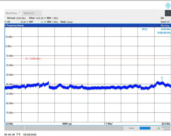
Band4-5MHz-QPSK-20175-1RB#0-3000~20000-PASS
