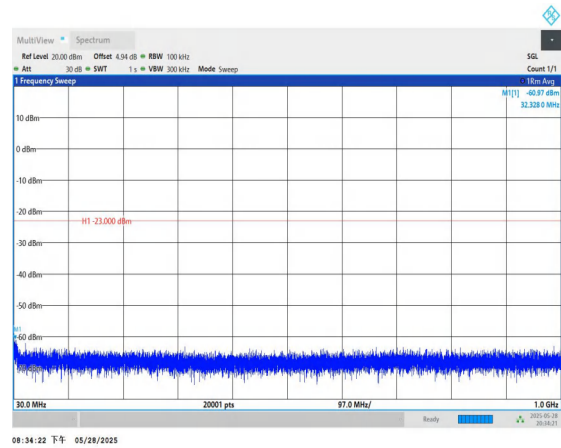
Band4-3MHz-QPSK-19965-1RB#0-30~1000-PASS
