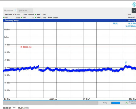
Band4-10MHz-QPSK-20000-1RB#0-3000~20000-PASS
