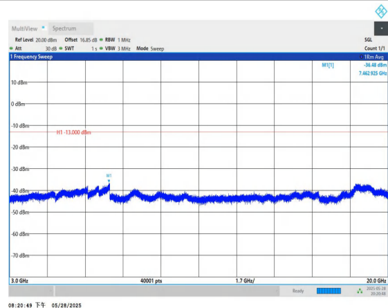
Band4-1.4MHz-QPSK-20175-1RB#0-3000~20000-PASS
