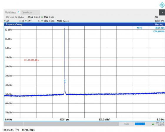
Band4-1.4MHz-QPSK-20393-1RB#0-1000~3000-PASS
