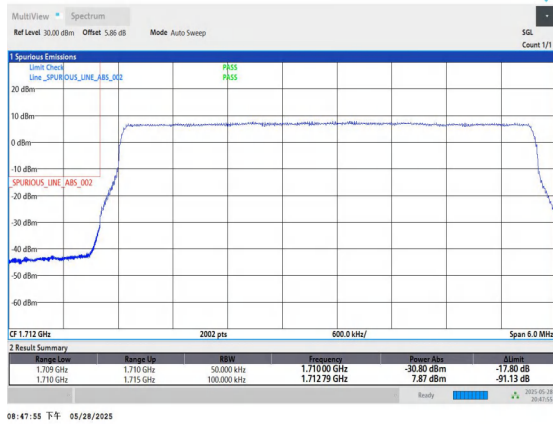
Band4-5MHz-QPSK-19975-25RB#0-PASS
