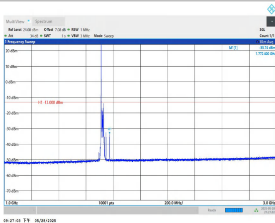
Band4-20MHz-QPSK-20050-1RB#0-1000~3000-PASS
