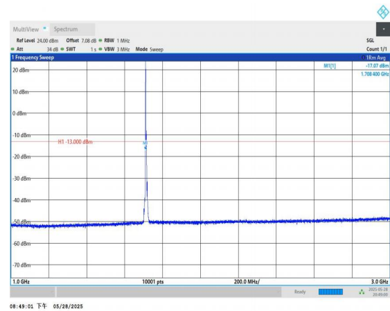
Band4-5MHz-QPSK-19975-1RB#0-1000~3000-PASS
