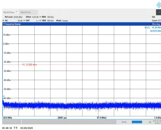
Band4-5MHz-QPSK-19975-1RB#0-30~1000-PASS
