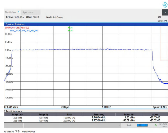
Band4-20MHz-QPSK-20300-100RB#0-PASS
