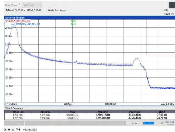
Band4-5MHz-QPSK-20375-1RB#0-PASS
