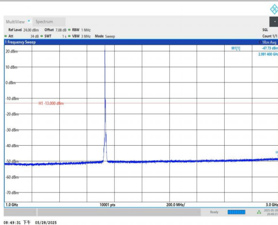
Band4-5MHz-QPSK-20175-1RB#0-1000~3000-PASS
