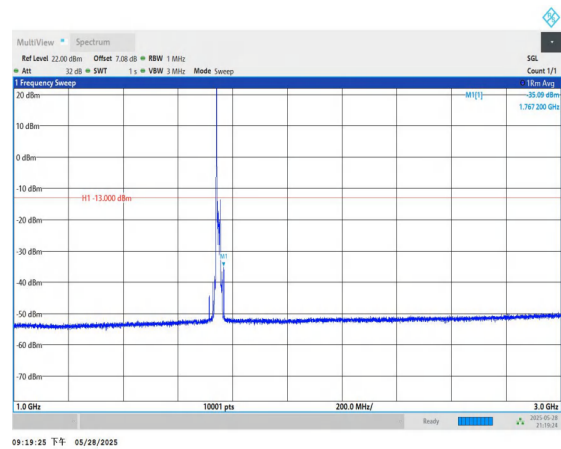
Band4-15MHz-QPSK-20325-1RB#0-1000~3000-PASS
