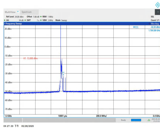
Band4-20MHz-QPSK-20175-1RB#0-1000~3000-PASS
