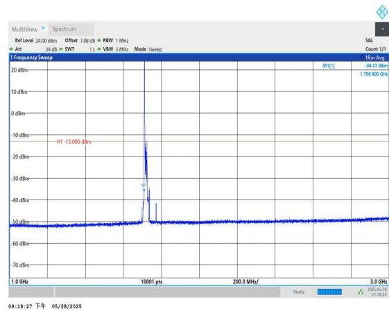
Band4-15MHz-QPSK-20025-1RB#0-1000~3000-PASS
