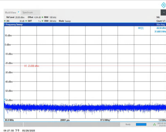
Band4-20MHz-QPSK-20300-1RB#0-30~1000-PASS
