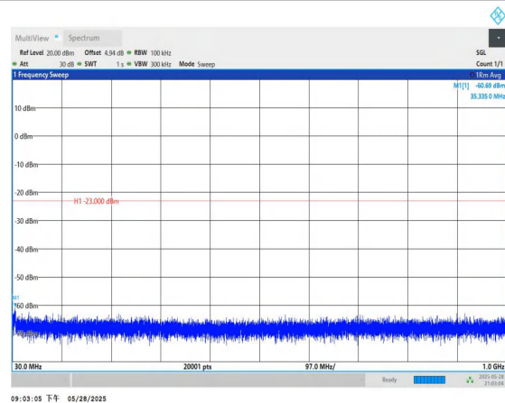
Band4-10MHz-QPSK-20000-1RB#0-30~1000-PASS
