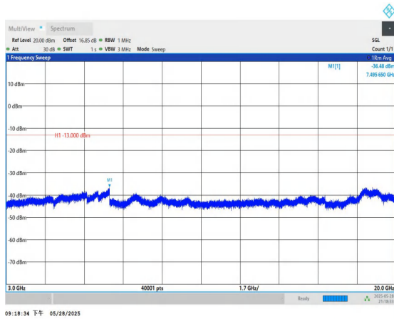
Band4-15MHz-QPSK-20025-1RB#0-3000~20000-PASS
