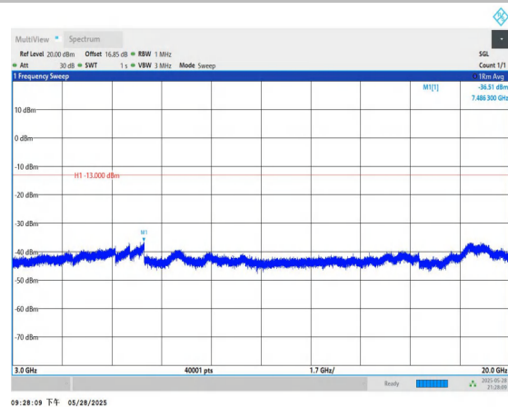
Band4-20MHz-QPSK-20300-1RB#0-3000~20000-PASS
