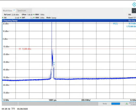
Band4-20MHz-QPSK-20300-1RB#0-1000~3000-PASS
