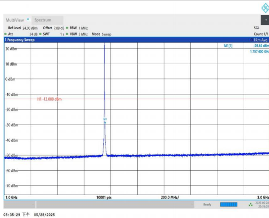
Band4-3MHz-QPSK-20385-1RB#0-1000~3000-PASS
