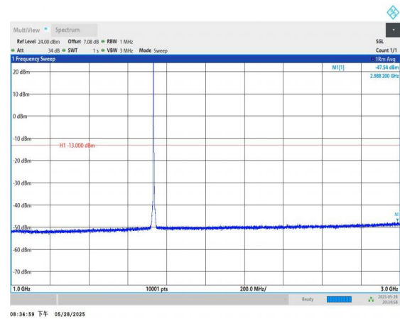
Band4-3MHz-QPSK-20175-1RB#0-1000~3000-PASS
