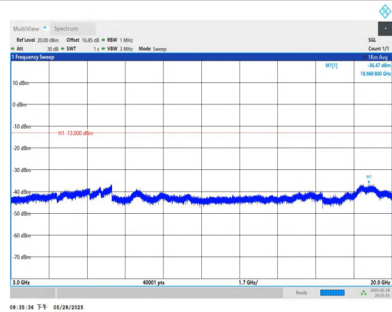
Band4-3MHz-QPSK-20385-1RB#0-3000~20000-PASS
