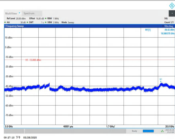
Band4-20MHz-QPSK-20050-1RB#0-3000~20000-PASS
