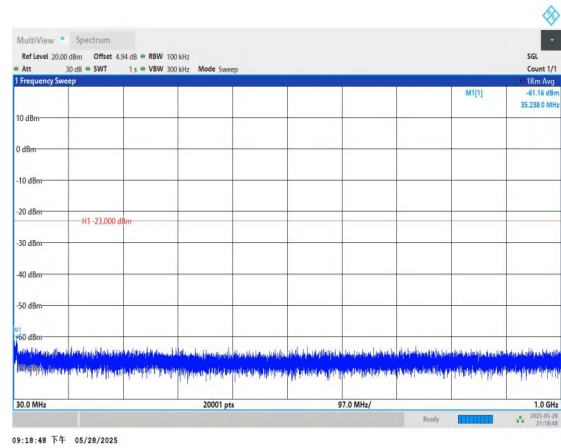
Band4-15MHz-QPSK-20175-1RB#0-30~1000-PASS
