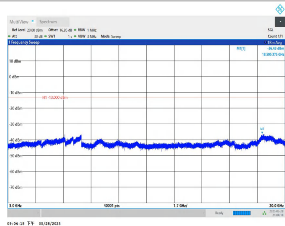
Band4-10MHz-QPSK-20350-1RB#0-3000~20000-PASS
