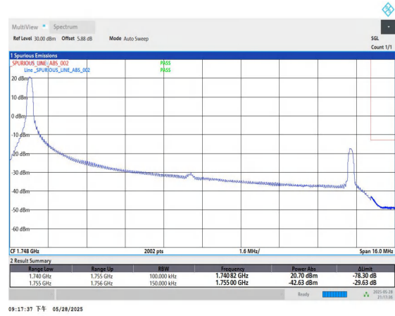
Band4-15MHz-QPSK-20325-1RB#0-PASS
