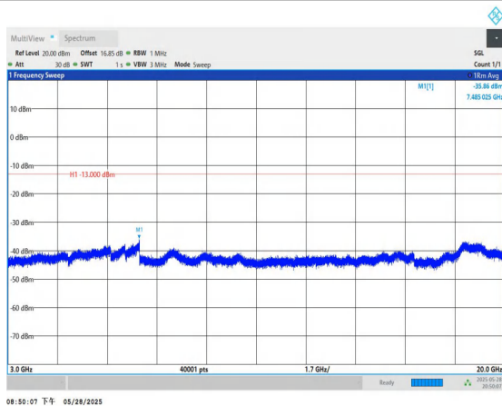
Band4-5MHz-QPSK-20375-1RB#0-3000~20000-PASS
