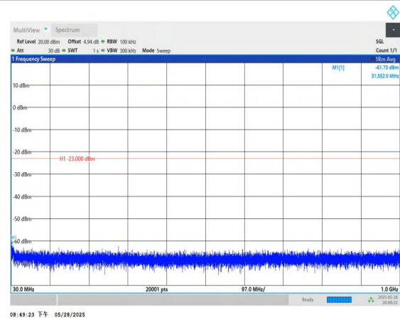
Band4-5MHz-QPSK-20175-1RB#0-30~1000-PASS
