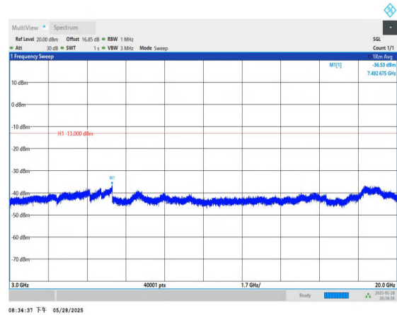
Band4-3MHz-QPSK-19965-1RB#0-3000~20000-PASS
