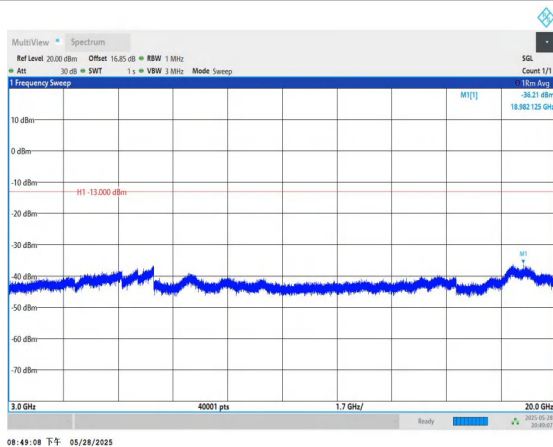
Band4-5MHz-QPSK-19975-1RB#0-3000~20000-PASS
