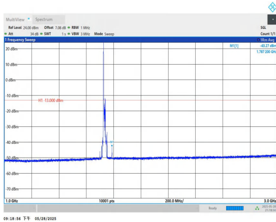
Band4-15MHz-QPSK-20175-1RB#0-1000~3000-PASS
