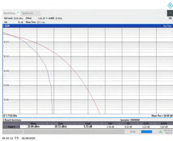
Band4-5MHz-QPSK-19975-1RB#0-PASS
