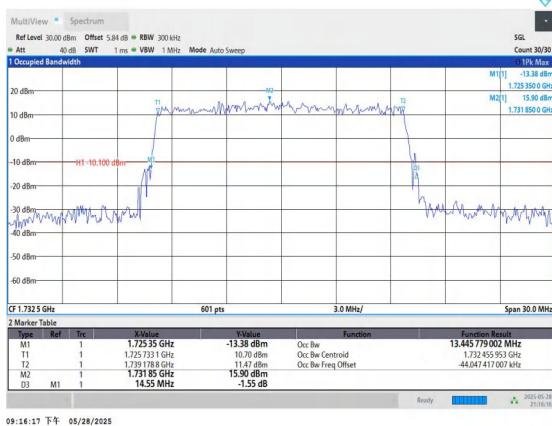
Band4-15MHz-16QAM-20175-75RB#0-PASS
