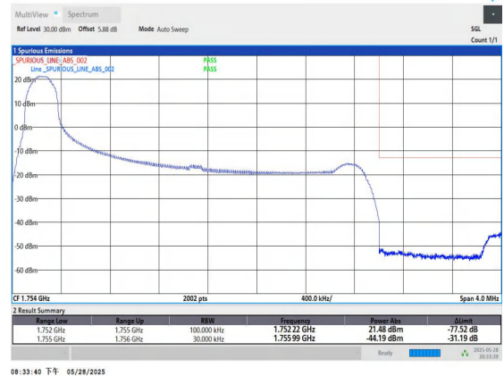
Band4-3MHz-QPSK-20385-1RB#0-PASS
