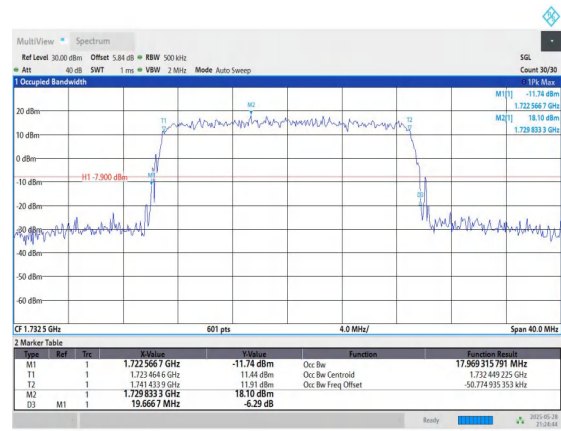
Band4-20MHz-QPSK-20175-100RB#0-PASS
