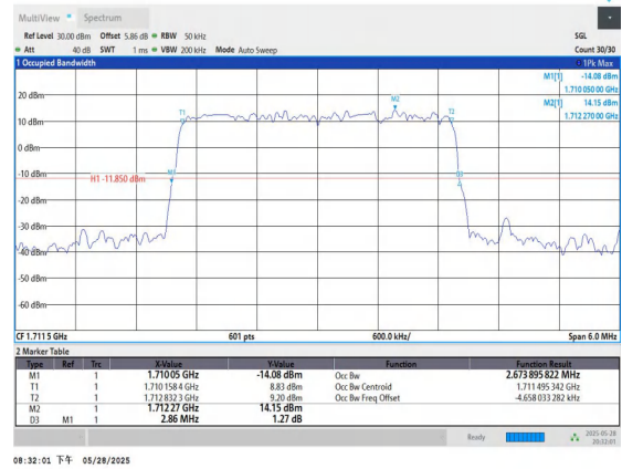
Band4-3MHz-16QAM-19965-15RB#0-PASS
