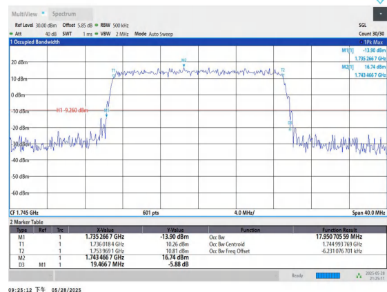
Band4-20MHz-16QAM-20300-100RB#0-PASS
