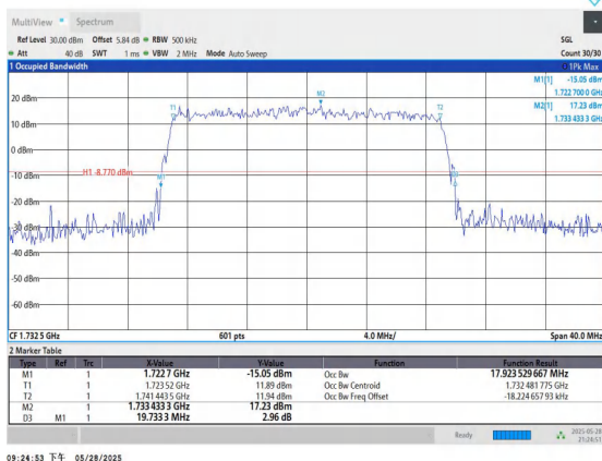
Band4-20MHz-16QAM-20175-100RB#0-PASS
