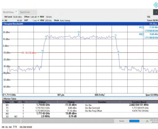
Band4-3MHz-QPSK-19965-15RB#0-PASS
