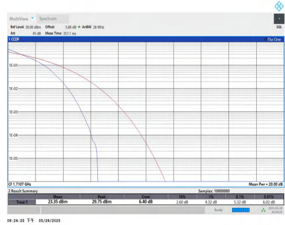
Band4-1.4MHz-QPSK-19957-6RB#0-PASS
