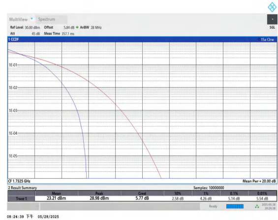
Band4-1.4MHz-QPSK-20175-6RB#0-PASS
