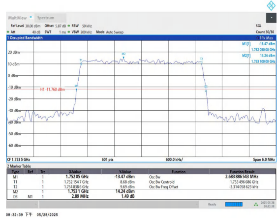
Band4-3MHz-16QAM-20385-15RB#0-PASS
