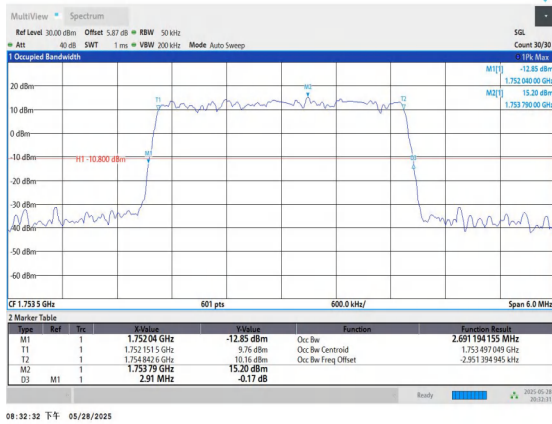
Band4-3MHz-QPSK-20385-15RB#0-PASS
