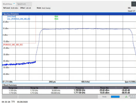
Band4-3MHz-QPSK-19965-15RB#0-PASS
