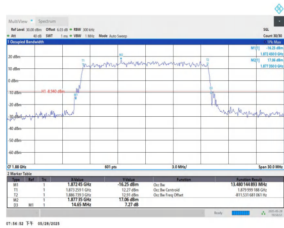
Band2-15MHz-QPSK-18900-75RB#0-PASS
