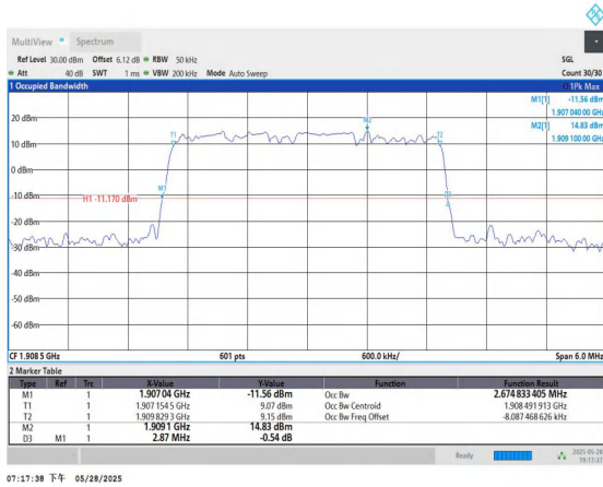
Band2-3MHz-QPSK-19185-15RB#0-PASS
