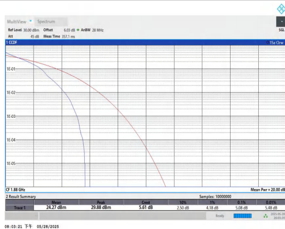
Band2-15MHz-QPSK-18900-1RB#0-PASS
