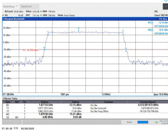
Band2-5MHz-16QAM-18900-25RB#0-PASS
