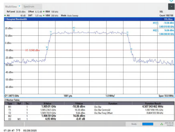
Band2-5MHz-16QAM-19175-25RB#0-PASS
