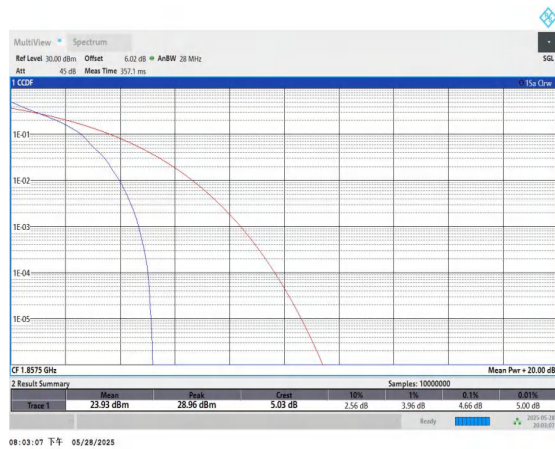
Band2-15MHz-QPSK-18675-1RB#0-PASS
