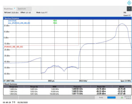
Band2-1.4MHz-QPSK-18607-1RB#5-PASS
