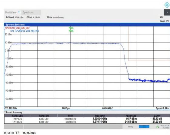
Band2-3MHz-QPSK-19185-15RB#0-PASS
