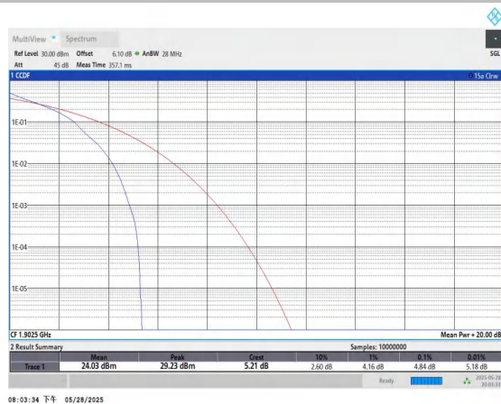
Band2-15MHz-QPSK-19125-1RB#0-PASS
