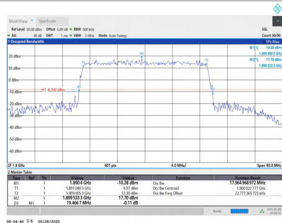
Band2-20MHz-16QAM-19100-100RB#0-PASS
