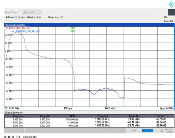
Band2-1.4MHz-QPSK-19193-1RB#0-PASS
