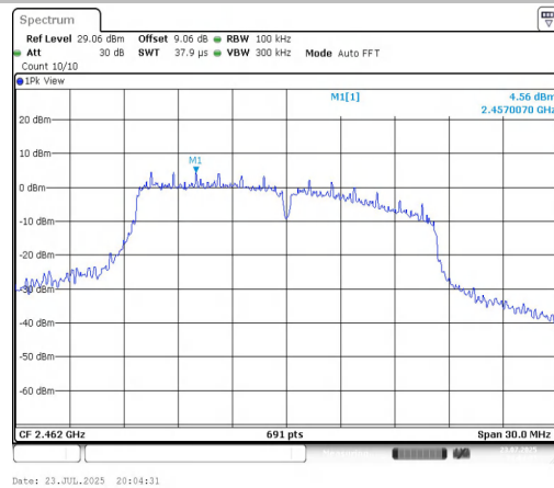
11G-Ant1-2462-0~Reference-PASS
