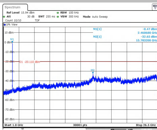
11N20SISO-Ant1-2462-0~Reference-PASS
