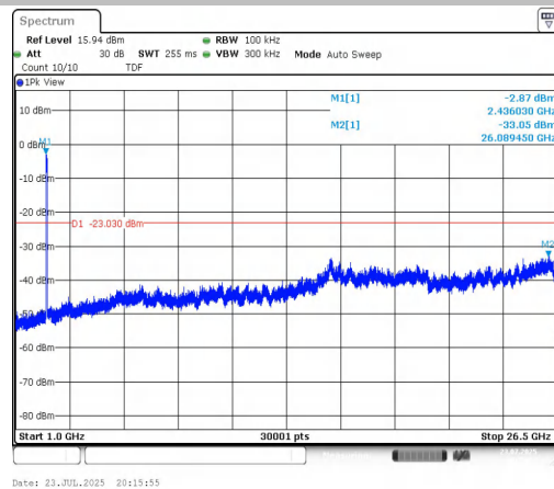
11N40SISO-Ant1-2452-1000~26500-PASS
