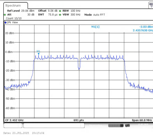
11N40SISO-Ant1-2452-0~Reference-PASS
