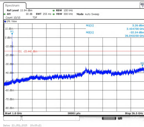
11G-Ant1-2462-1000~26500-PASS
