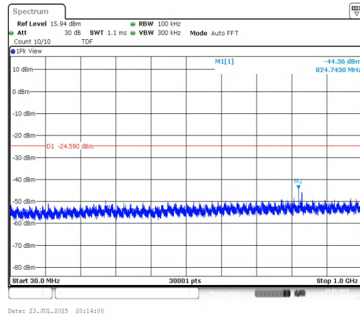
11N40SISO-Ant1-2437-30~1000-PASS
