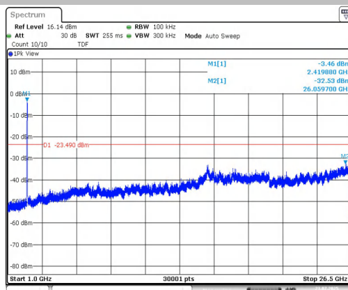
11N40SISO-Ant1-2422-0~Reference-PASS
