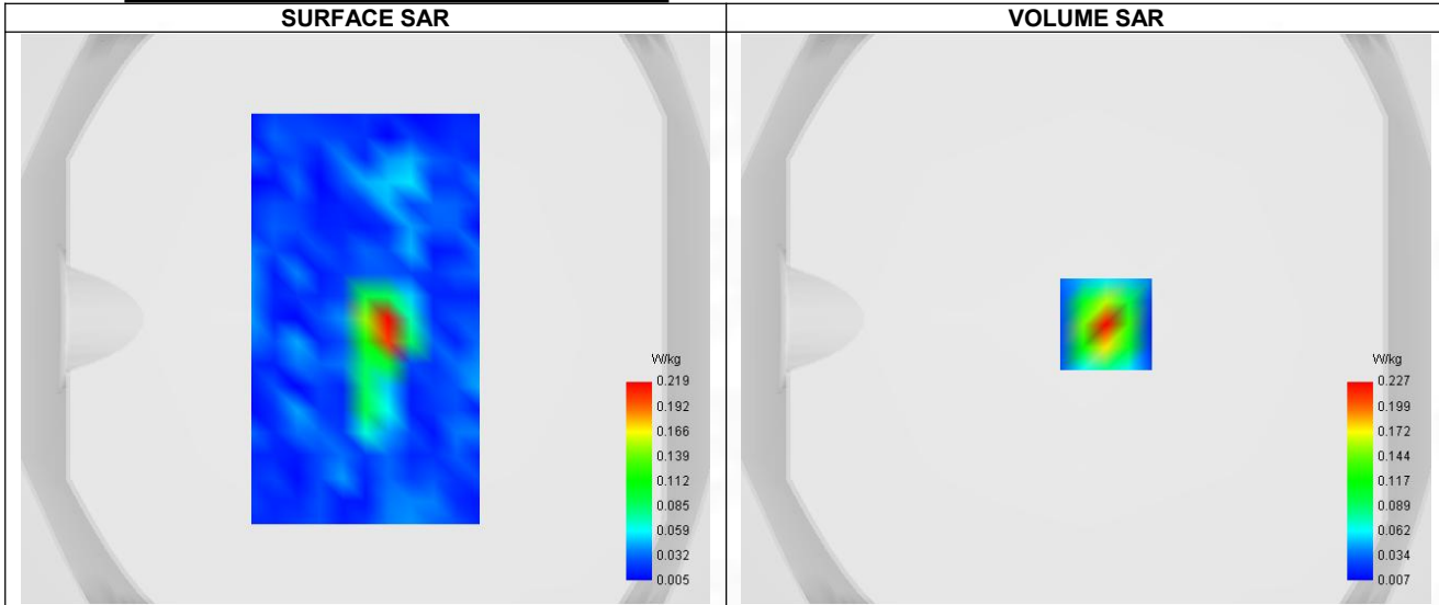
Maximum location: X=7.00, Y=-2.00 ; SAR Peak: 0.35 W/kg
