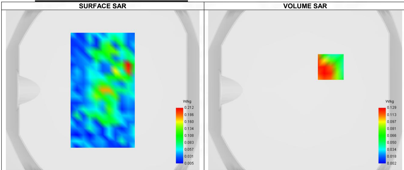
Maximum location: X=32.00, Y=29.00 ; SAR Peak: 0.18 W/kg
