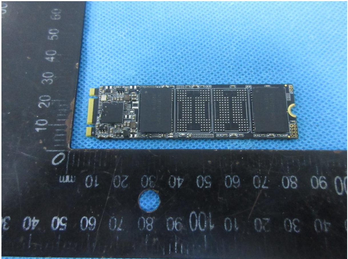
Photo 24 SSD#2
