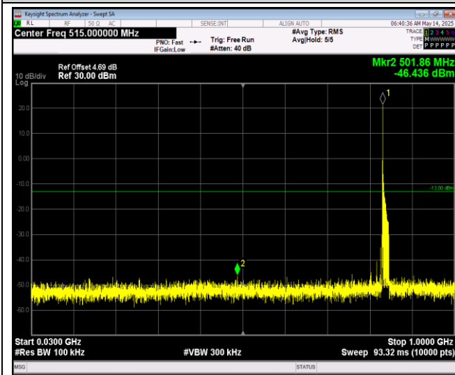
Band26-15MHz-64QAM-26965-1RB#0-Range1:30~1000MHz
