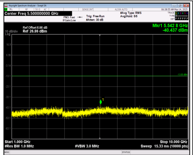
Band26-15MHz-64QAM-26915-1RB#0-Range2:1000~10000MHz
