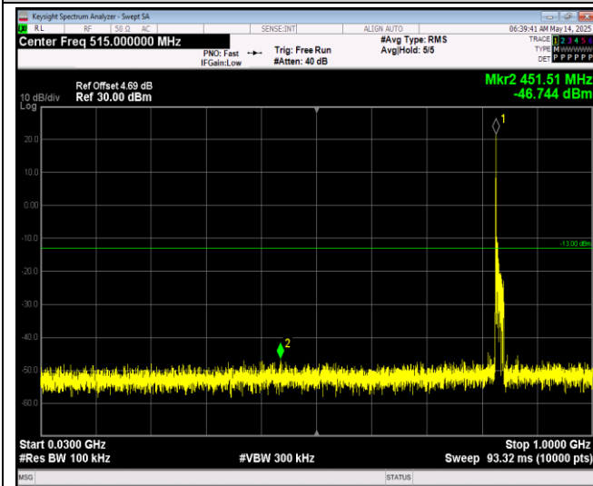
Band26-15MHz-64QAM-26965-1RB#0-Range1:30~1000MHz
