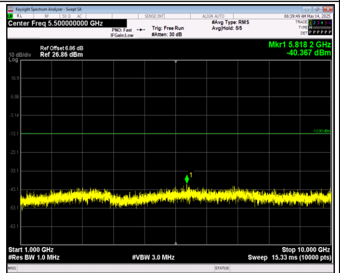
Band26-15MHz-64QAM-26965-1RB#0-Range2:1000~10000MHz
