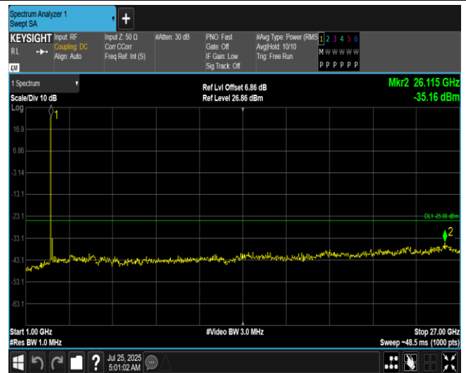
Band41-5MHz-QPSK-40620-1RB#0-Range2:1000~27000 MHz
