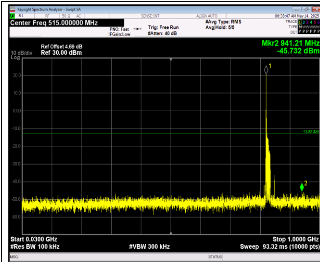
Band26-15MHz-64QAM-26915-1RB#0-Range1:30~1000MHz
