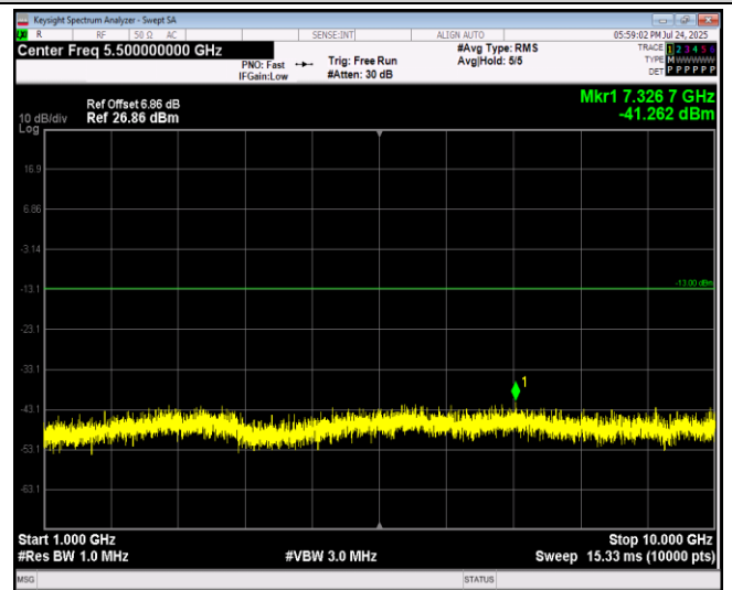
Band17-10MHz-64QAM-23800-1RB#0-Range2:1000~10000MHz
