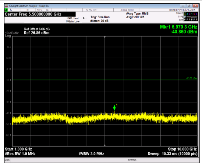
Band17-10MHz-64QAM-23790-1RB#0-Range2:1000~10000MHz
