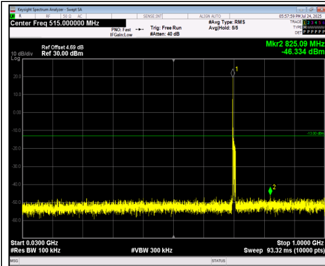
Band17-10MHz-64QAM-23790-1RB#0-Range1:30~1000MHz
