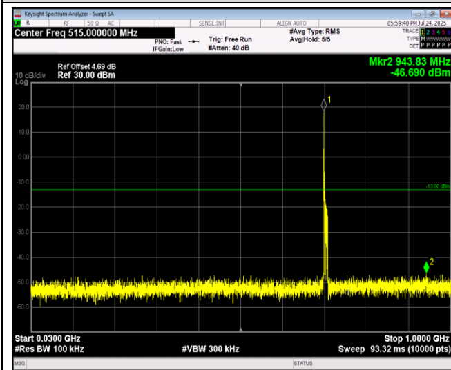
Band17-10MHz-64QAM-23800-1RB#0-Range1:30~1000MHz
