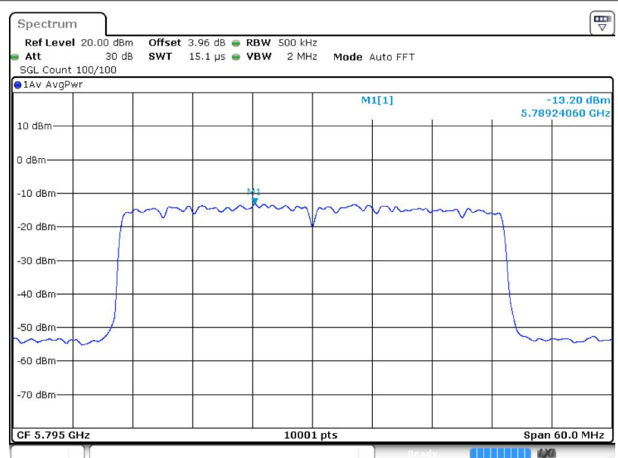
PSD ax40 5795MHz Ant2
