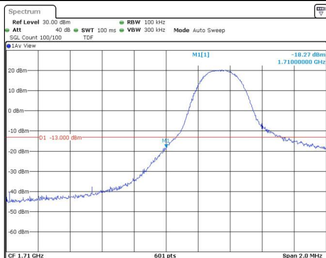
Band66-5MHz-QPSK-131997-1RB#24
