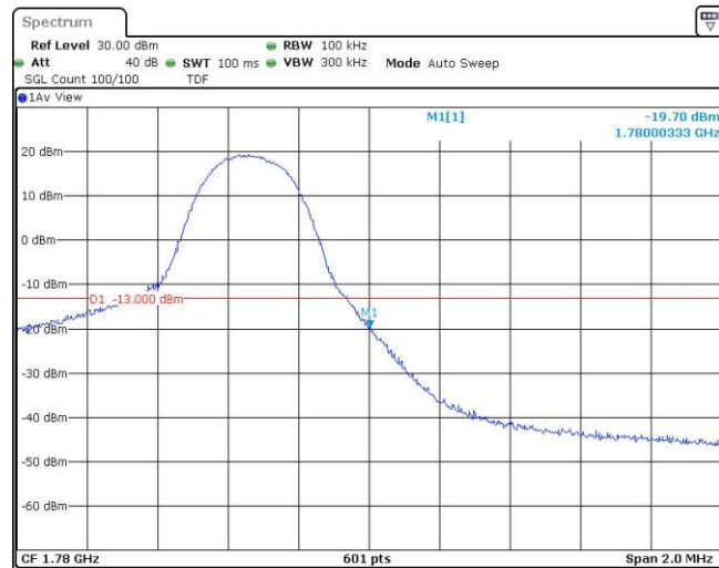
Band66-5MHz-16QAM-132647-25RB#0
