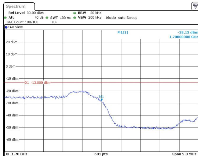
Band66-3MHz-QPSK-132657-1RB#14
