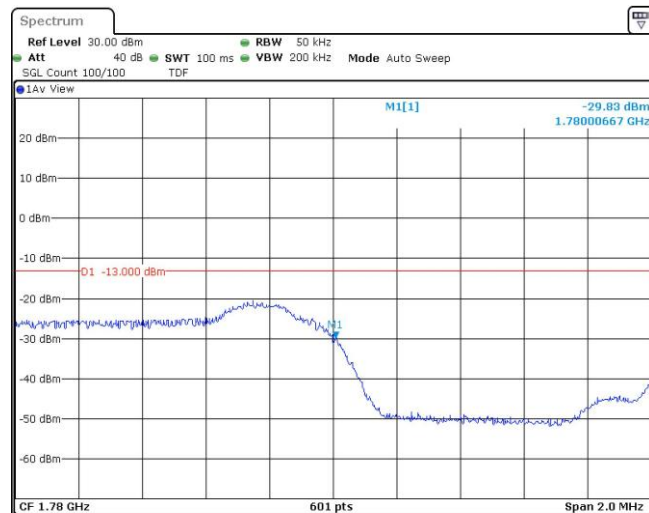
Band66-3MHz-16QAM-132657-1RB#14
