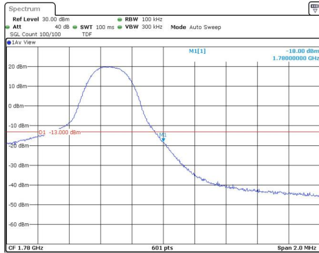
Band66-5MHz-QPSK-132647-25RB#0
