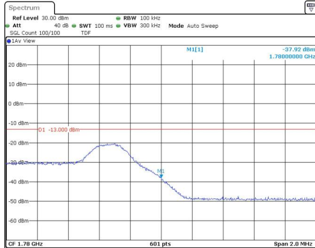
Band66-5MHz-QPSK-132647-1RB#24
