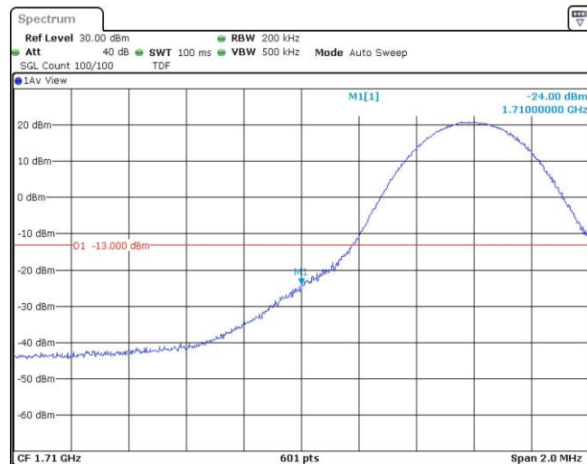
Band66-10MHz-16QAM-132022-1RB#49
