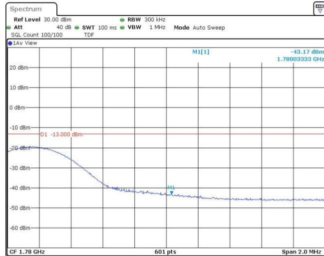
Band66-15MHz-16QAM-132597-1RB#74
