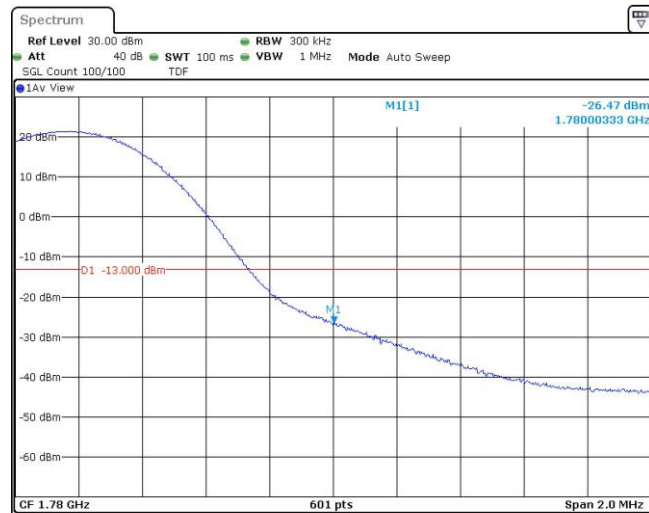
Band66-15MHz-QPSK-132597-75RB#0
