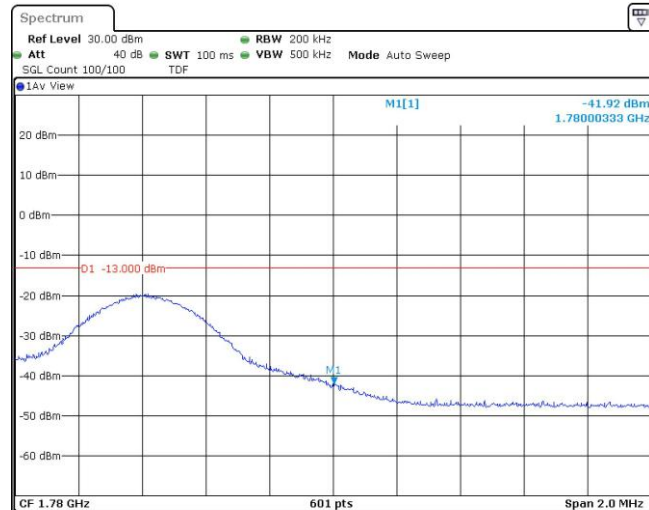
Band66-10MHz-16QAM-132622-1RB#49
