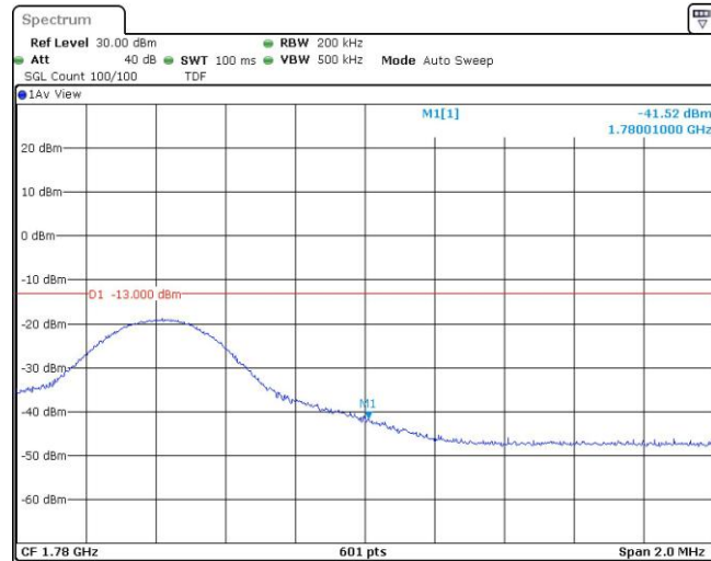
Band66-10MHz-QPSK-132622-1RB#49
