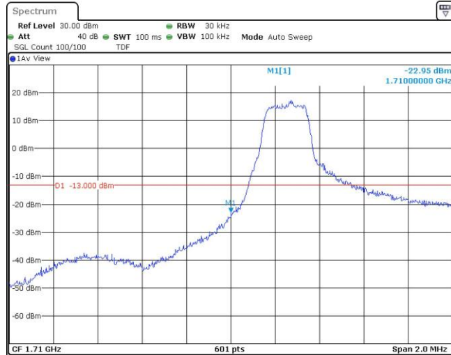
Band66-1.4MHz-16QAM-131979-1RB#5
