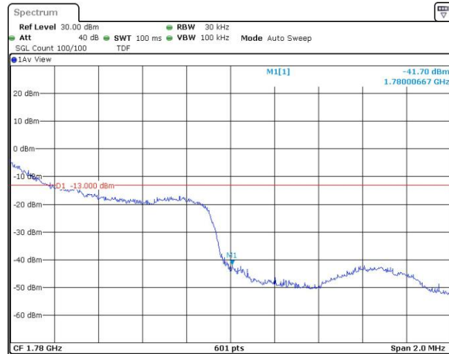
Band66-1.4MHz-QPSK-132665-1RB#5
