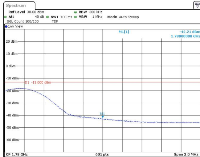
Band66-15MHz-QPSK-132597-1RB#74
