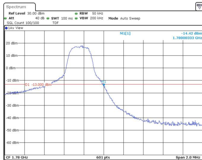
Band66-3MHz-16QAM-132657-15RB#0
