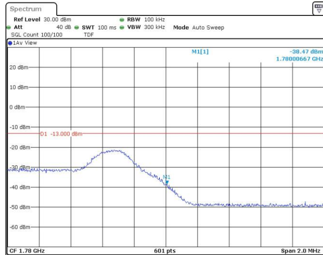
Band66-5MHz-16QAM-132647-1RB#24
