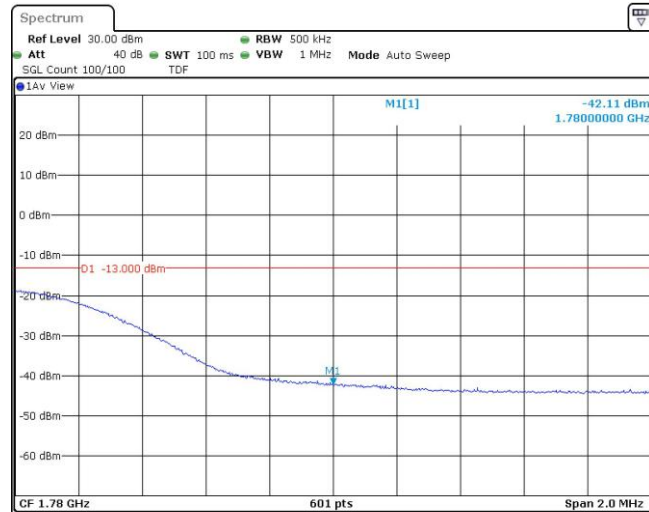
Band66-20MHz-16QAM-132572-1RB#99
