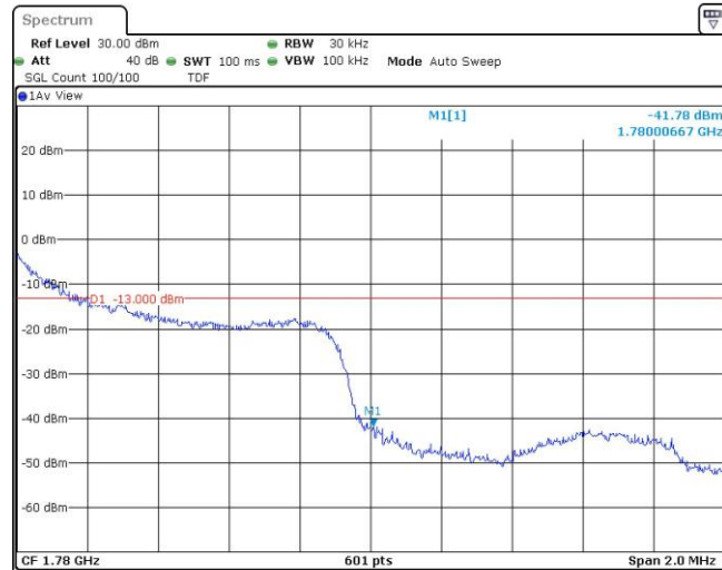
Band66-1.4MHz-16QAM-132665-1RB#5
