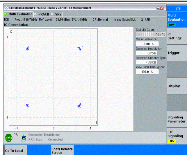
Band66-1.4MHz-QPSK-132322-6RB#0
