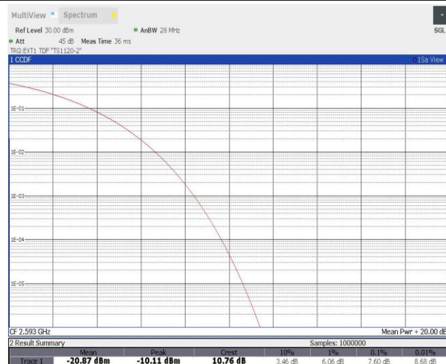
Band41-20MHz-QPSK-40620-100RB#0
