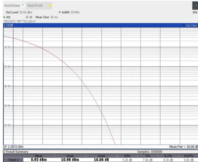
Band41-15MHz-16QAM-39765-75RB#0
