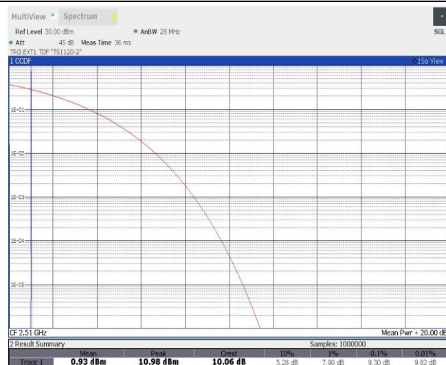
Band41-20MHz-16QAM-39790-100RB#0
