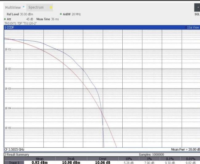
Band41-5MHz-16QAM-39715-25RB#0
