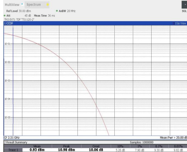
Band41-20MHz-QPSK-39790-100RB#0
