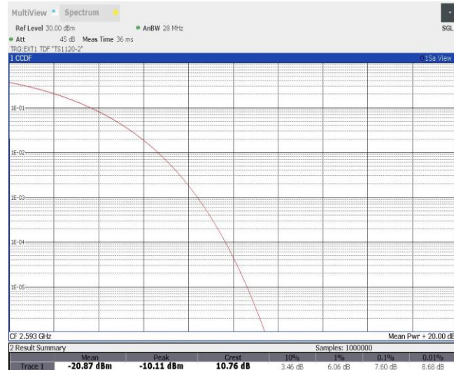
Band41-10MHz-QPSK-40620-50RB#0
