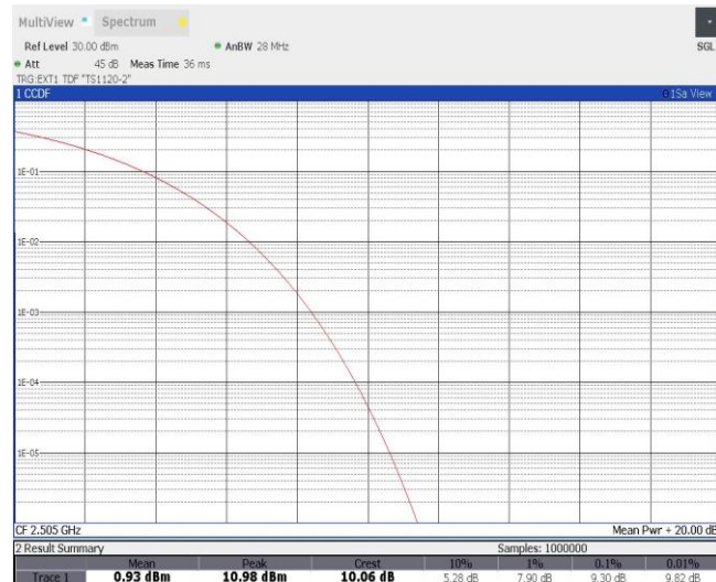
Band41-10MHz-16QAM-40620-1RB#0
