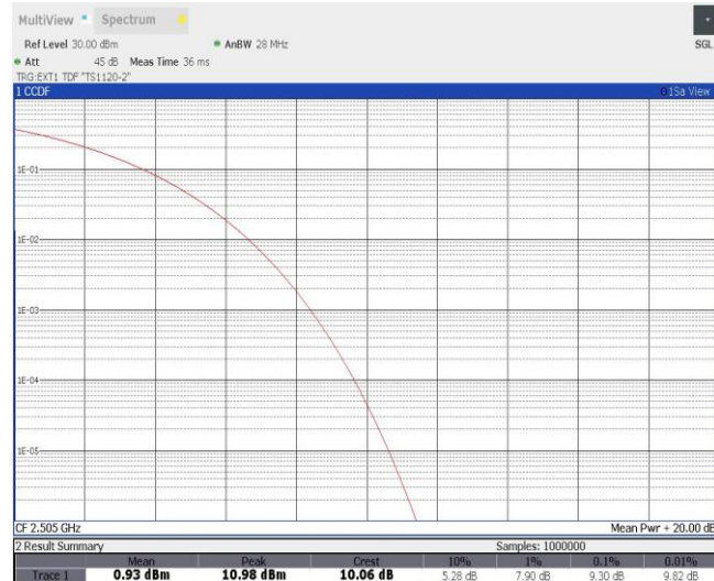
Band41-10MHz-16QAM-39740-50RB#0
