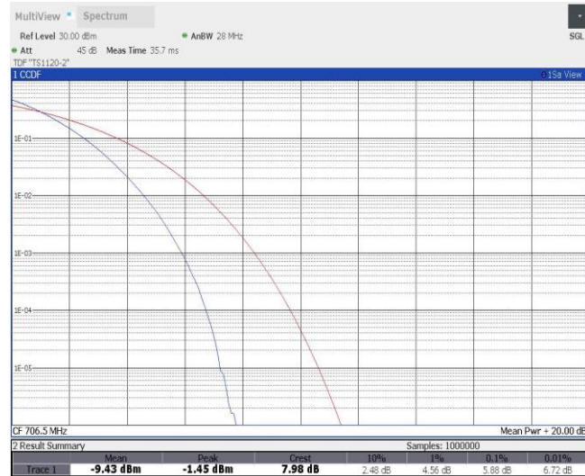
Band17-5MHz-QPSK-23755-25RB#0
