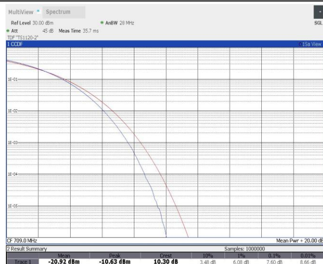
Band17-10MHz-16QAM-23790-1RB#0
