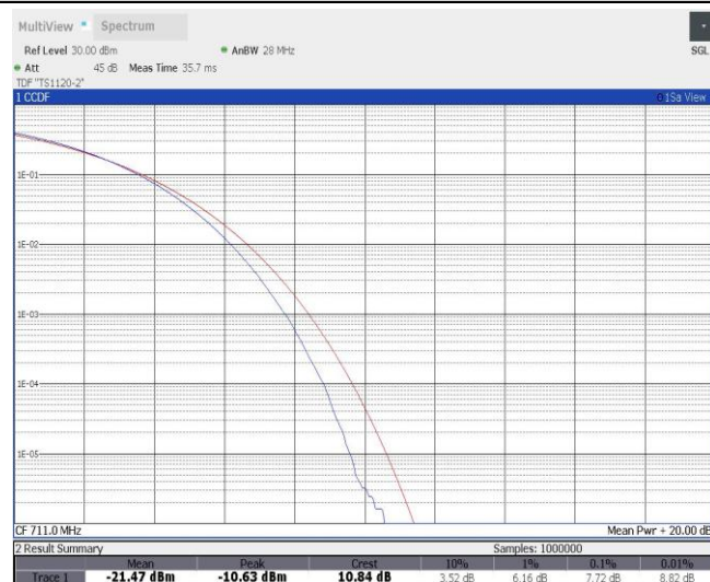
Band17-10MHz-16QAM-23800-50RB#0
