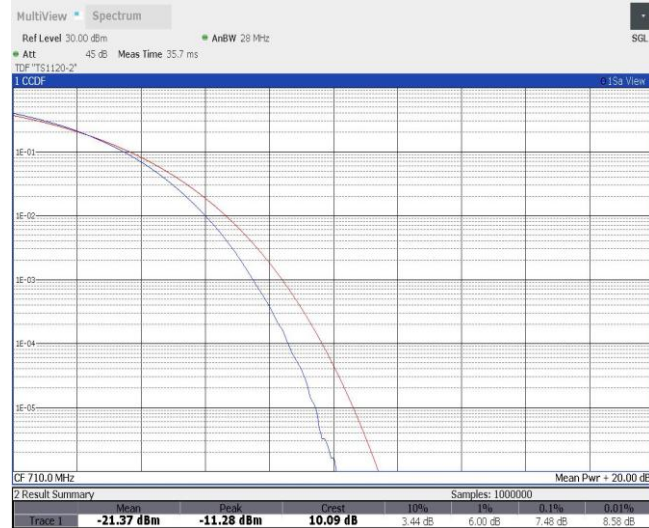
Band17-5MHz-QPSK-23790-25RB#0
