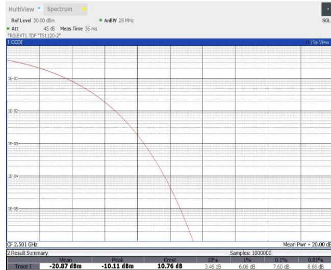
Band41-10MHz-QPSK-39740-1RB#0
