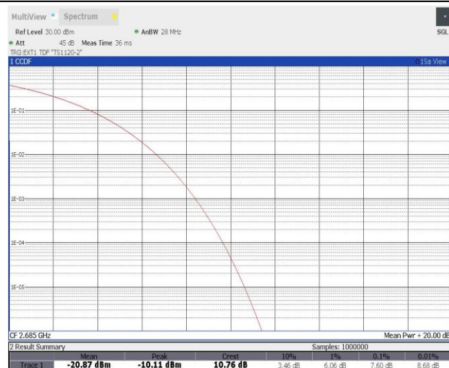
Band41-10MHz-QPSK-41540-50RB#0
