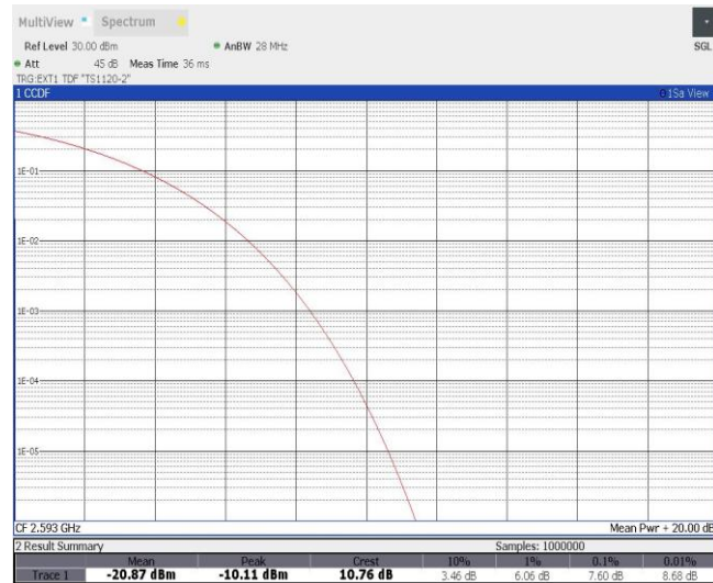
Band41-15MHz-QPSK-40620-75RB#0
