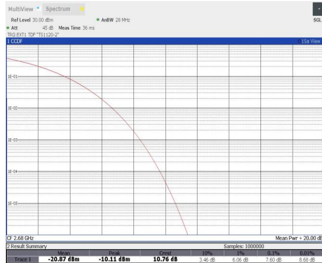
Band41-20MHz-16QAM-41490-100RB#0
