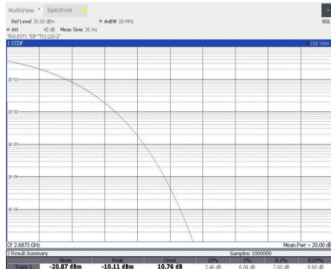
Band41-5MHz-QPSK-41565-25RB#0
