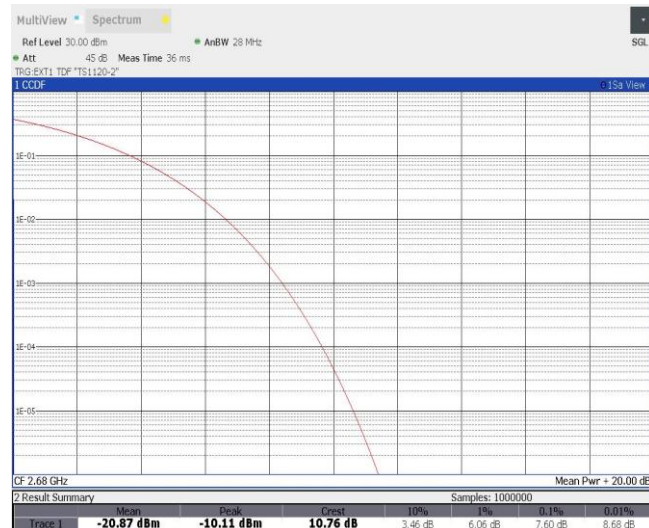
Band41-20MHz-QPSK-41490-100RB#0
