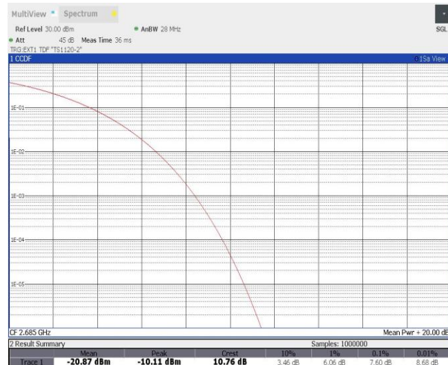
Band41-10MHz-16QAM-41540-50RB#0
