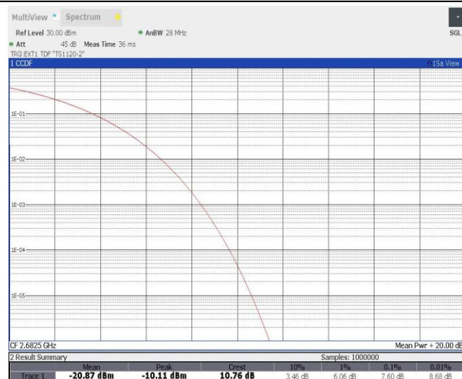
Band41-15MHz-16QAM-41515-75RB#0
