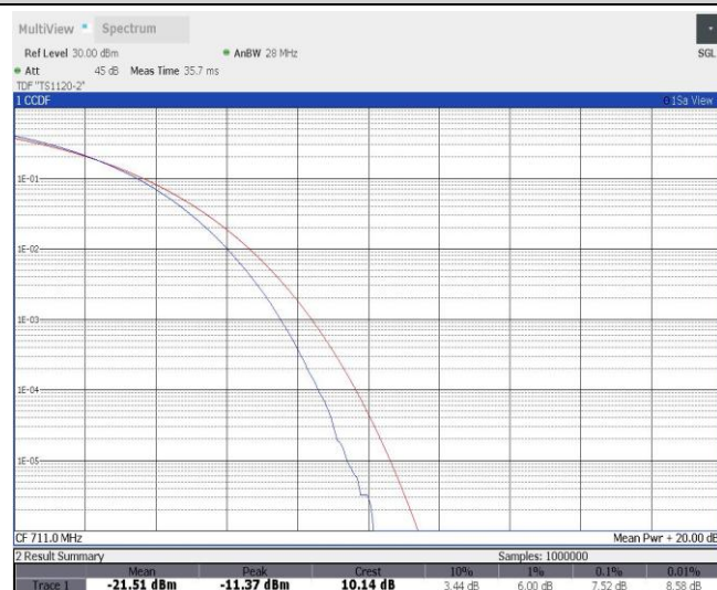
Band12-10MHz-QPSK-23130-50RB#0
