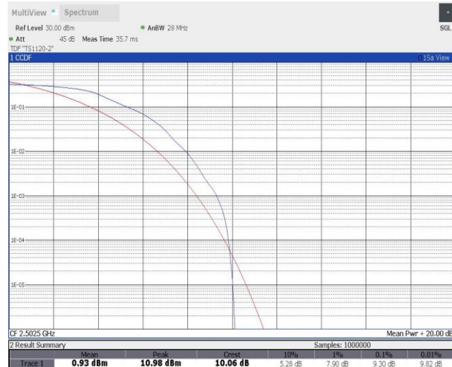
Band41-5MHz-QPSK-39715-25RB#0
