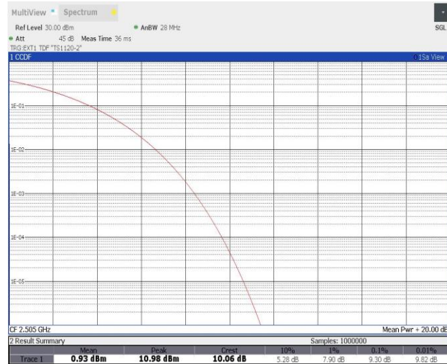
Band41-10MHz-QPSK-39740-50RB#0
