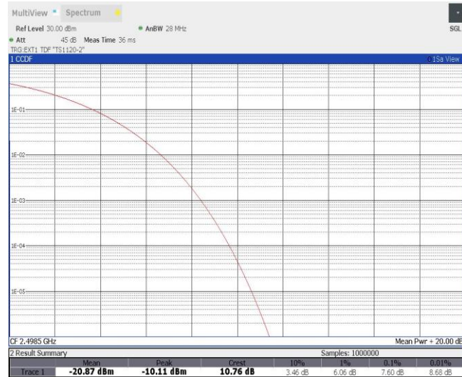
Band41-5MHz-16QAM-39675-25RB#0
