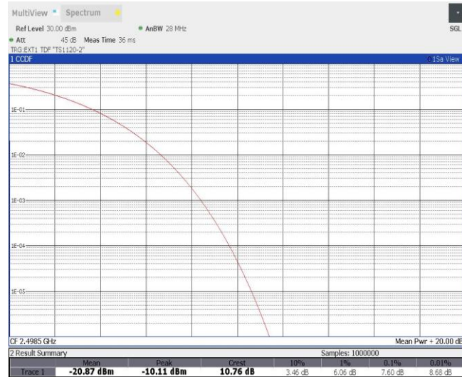
Band41-5MHz-QPSK-39675-25RB#0
