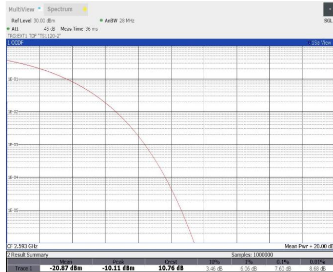
Band41-15MHz-16QAM-40620-75RB#0
