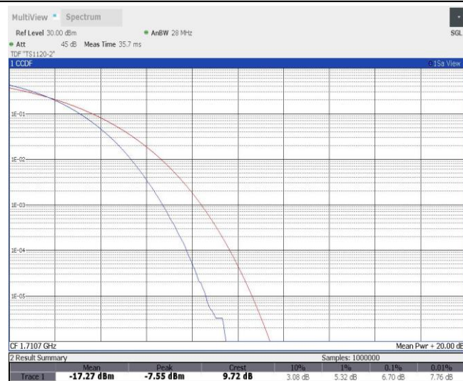
Band66-1.4MHz-QPSK-131979-6RB#0
