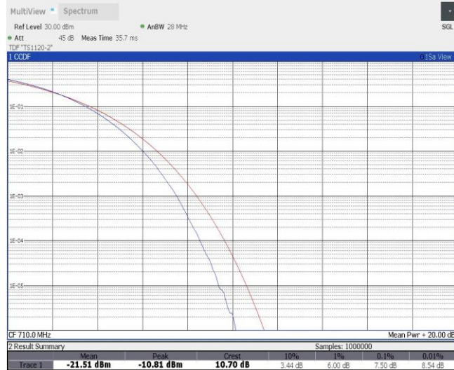
Band17-10MHz-QPSK-23790-50RB#0
