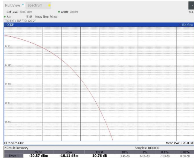
Band41-5MHz-16QAM-41565-25RB#0
