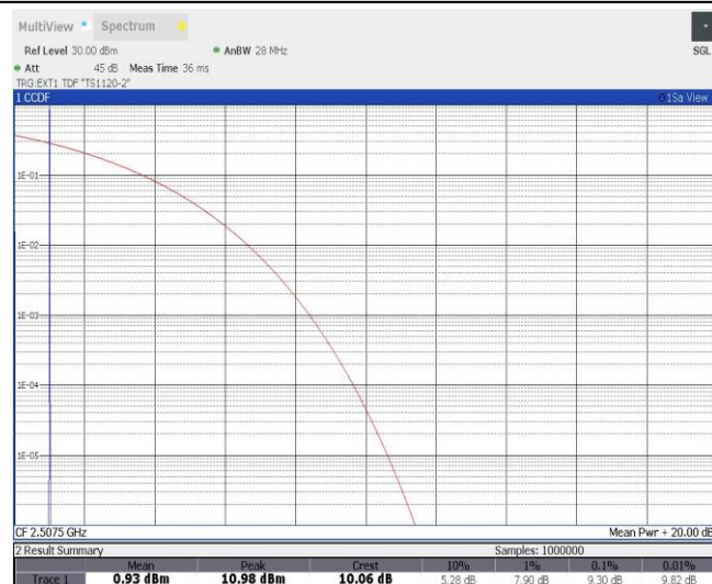
Band41-15MHz-QPSK-39765-75RB#0
