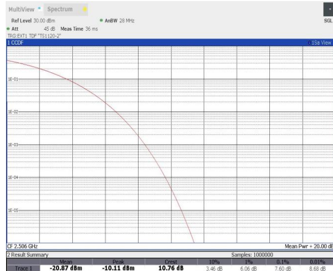
Band41-20MHz-16QAM-39750-100RB#0
