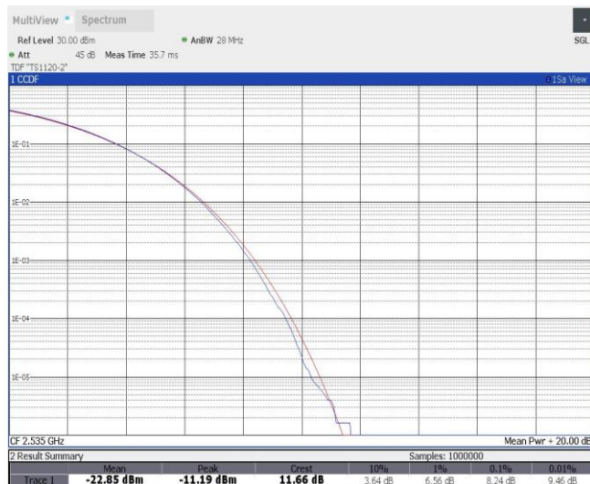
Band7-15MHz-16QAM-21375-1RB#0
