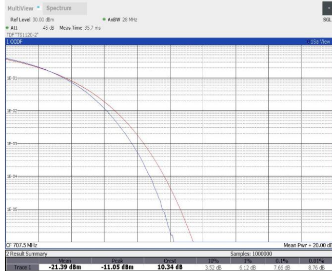
Band12-3MHz-16QAM-23095-15RB#0
