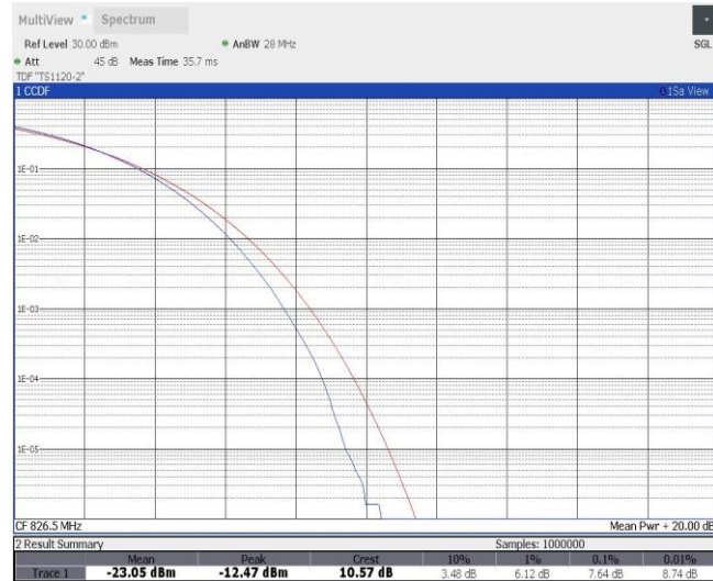
Band5-5MHz-QPSK-20425-25RB#0
