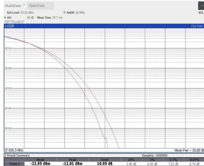
Band5-5MHz-QPSK-20525-25RB#0
