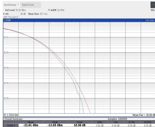
Band4-20MHz-16QAM-20300-1RB#0
