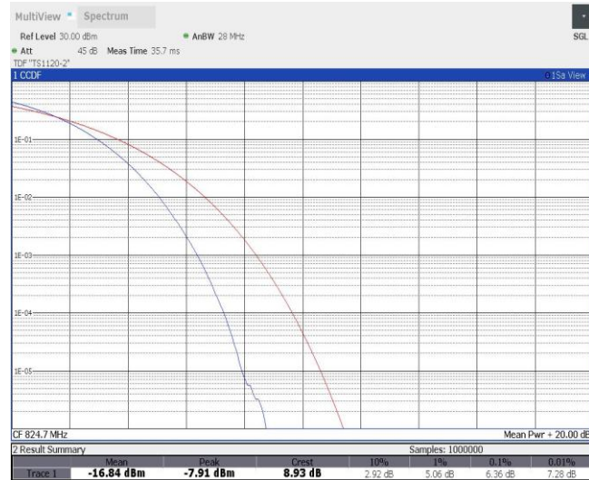
Band5-1.4MHz-QPSK-20407-6RB#0
