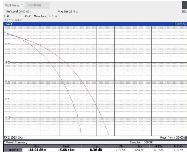
Band7-5MHz-QPSK-20775-25RB#0
