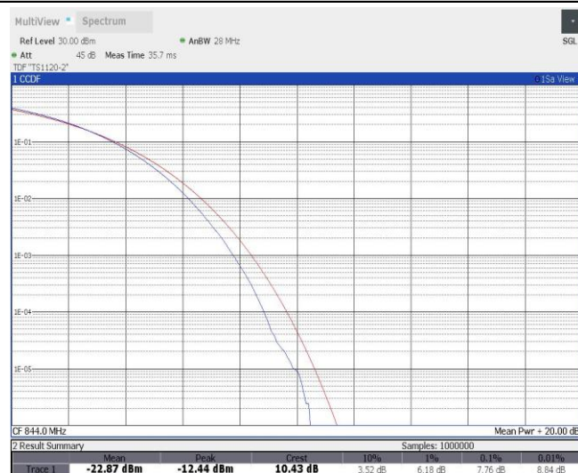
Band5-10MHz-16QAM-20600-50RB#0
