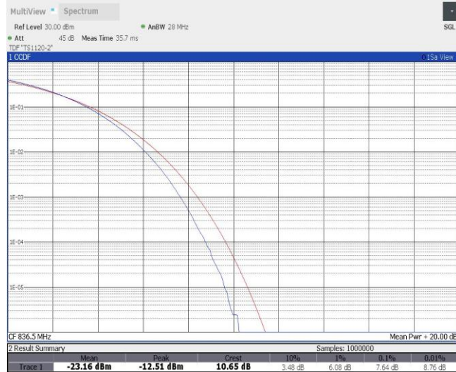
Band5-10MHz-QPSK-20525-50RB#0
