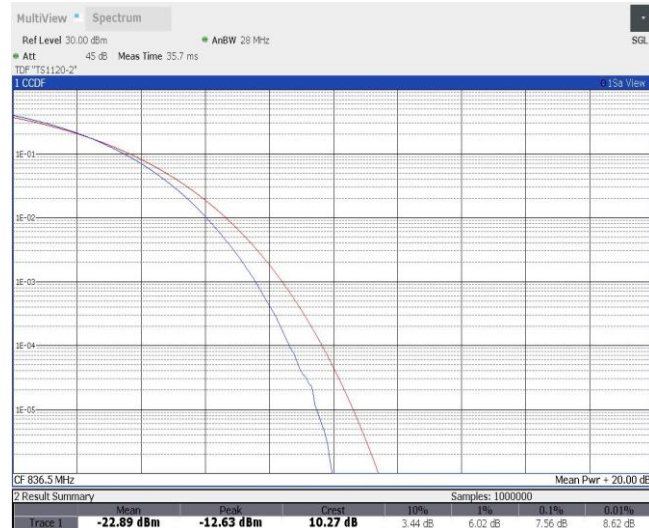
Band5-3MHz-QPSK-20525-15RB#0
