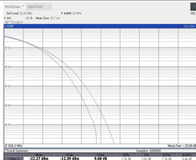
Band5-5MHz-QPSK-20525-1RB#0
