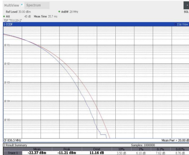
Band5-5MHz-16QAM-20625-1RB#0
