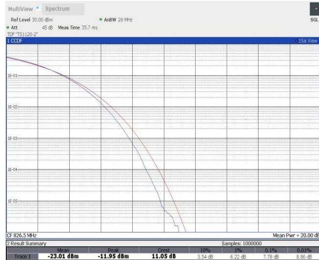
Band5-5MHz-16QAM-20425-25RB#0
