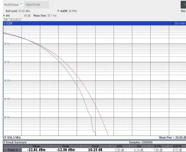
Band5-5MHz-16QAM-20525-25RB#0
