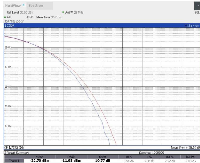
Band4-20MHz-QPSK-20175-100RB#0
