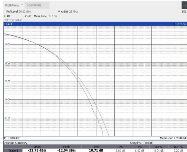
Band2-15MHz-16QAM-18900-75RB#0
