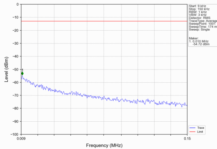
Band5_10MHz_16QAM_HCH_844MHz_RB_1_0_NTNV
