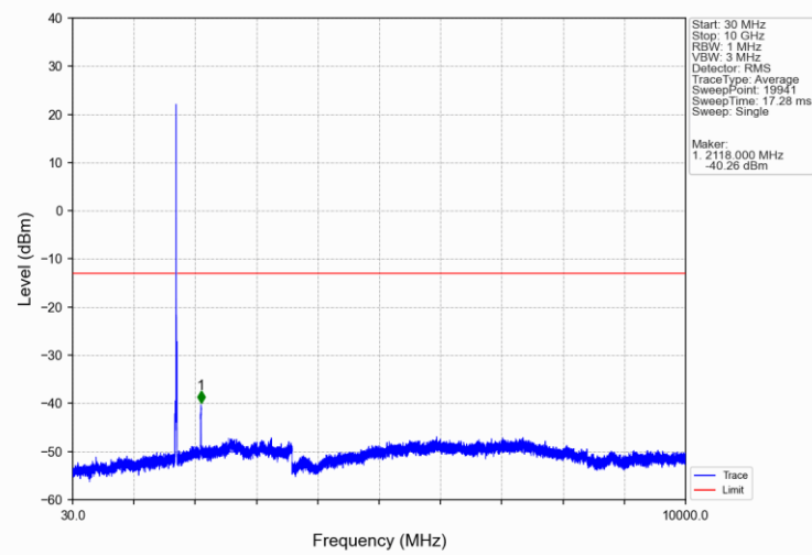
Band4_10MHz_16QAM_LCH_1715MHz_RB_1_0_NTNV
