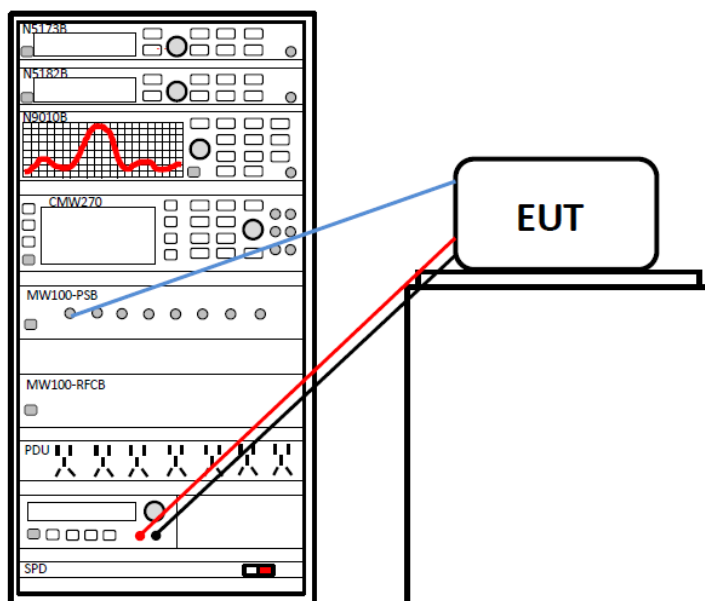
Conduction test items set diagram
