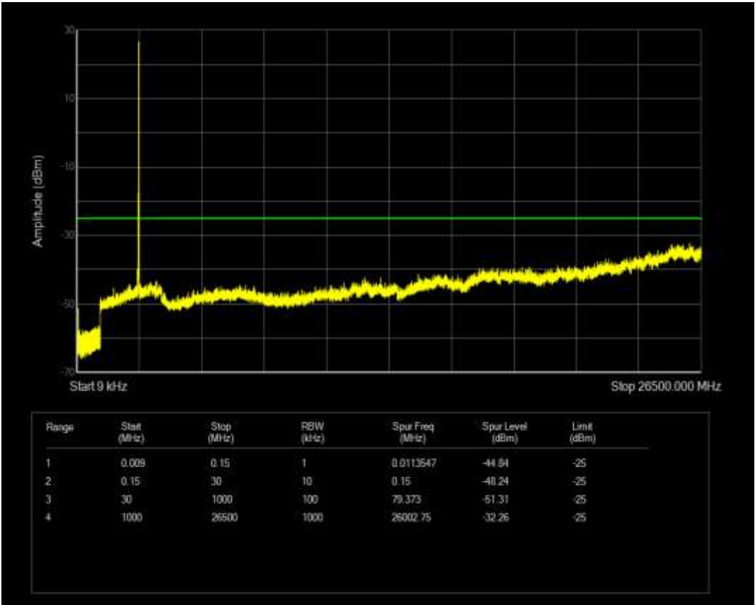
Band41 QPSK BW=10MHz Channel=41140 RB Size=50 Position=#0
