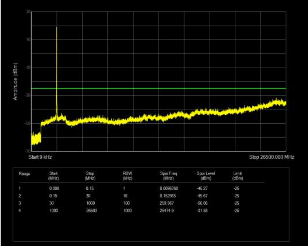
Band41 16QAM BW=10MHz Channel=41140 RB Size=1 Position=#0
