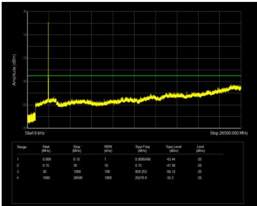
Band41 QPSK BW=5MHz Channel=41165 RB Size=1 Position=#0
