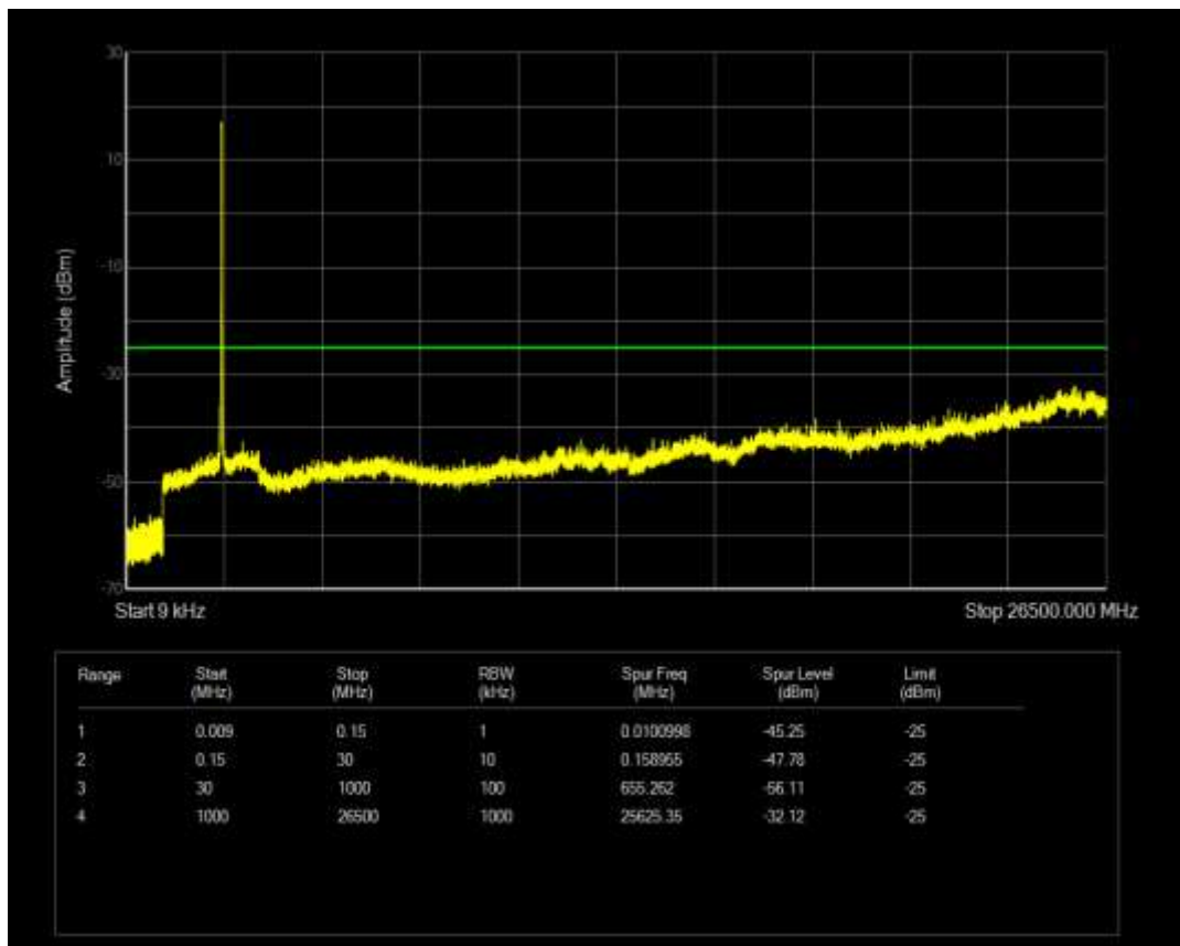
Band41 QPSK BW=15MHz Channel=41115 RB Size=1 Position=#0
