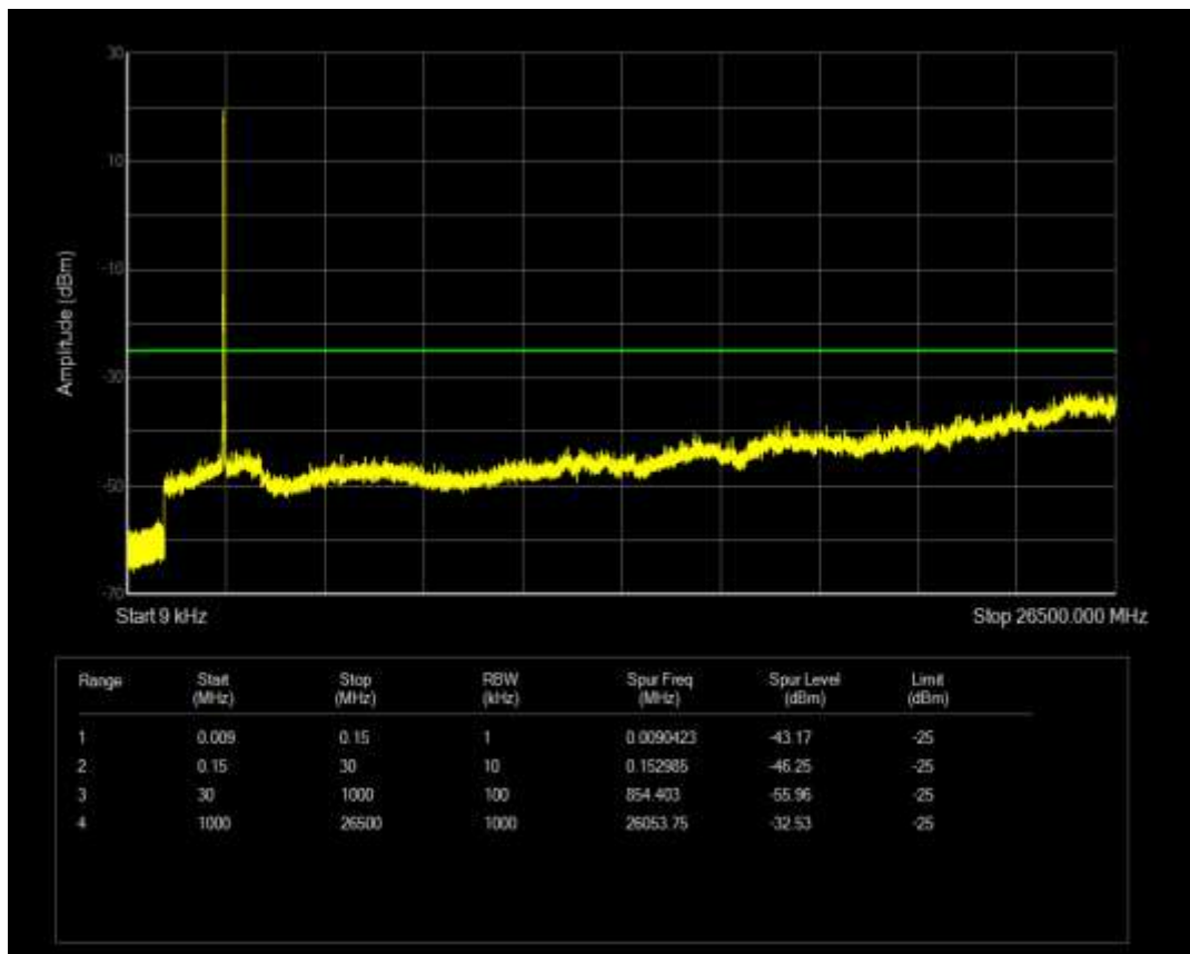
Band41 QPSK BW=10MHz Channel=41140 RB Size=1 Position=#0
