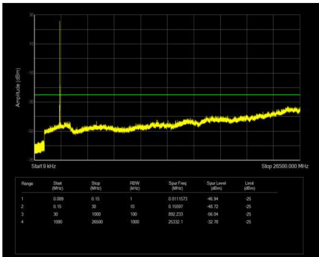
Band41 16QAM BW=10MHz Channel=40140 RB Size=50 Position=#0
