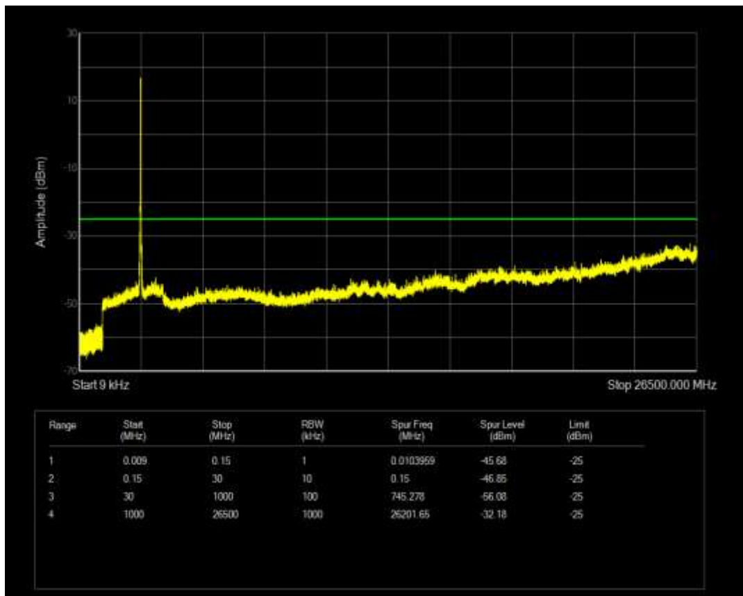
Band41 16QAM BW=20MHz Channel=41090 RB Size=1 Position=#0
