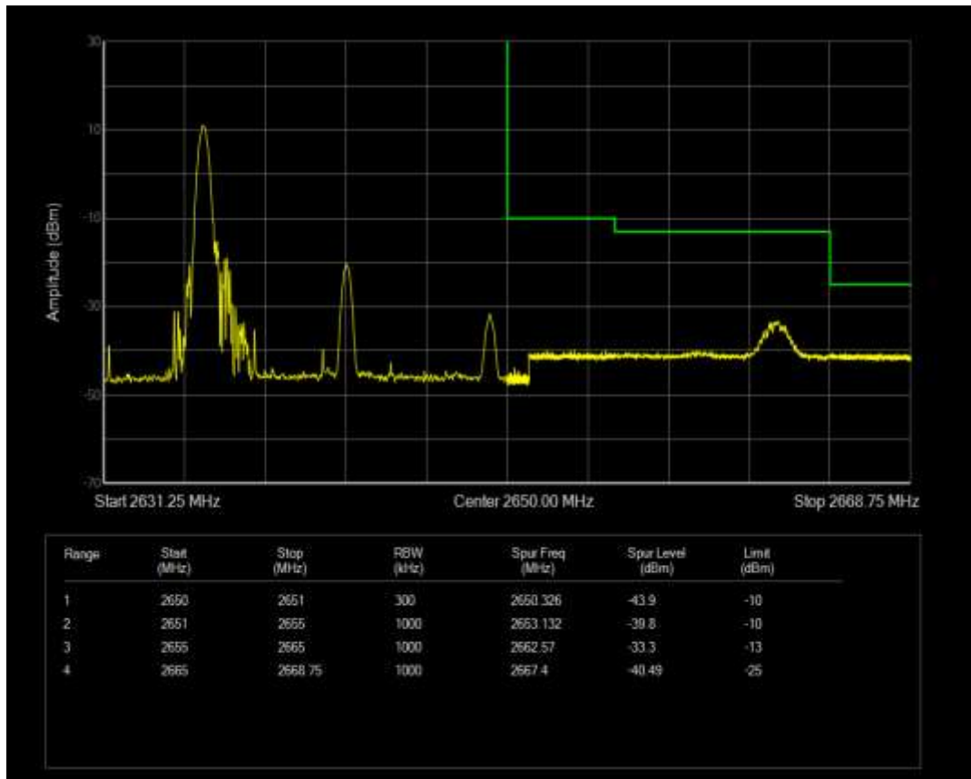
Band41 QPSK BW=15MHz Channel=41115 RB Size=1 Position=#Max
