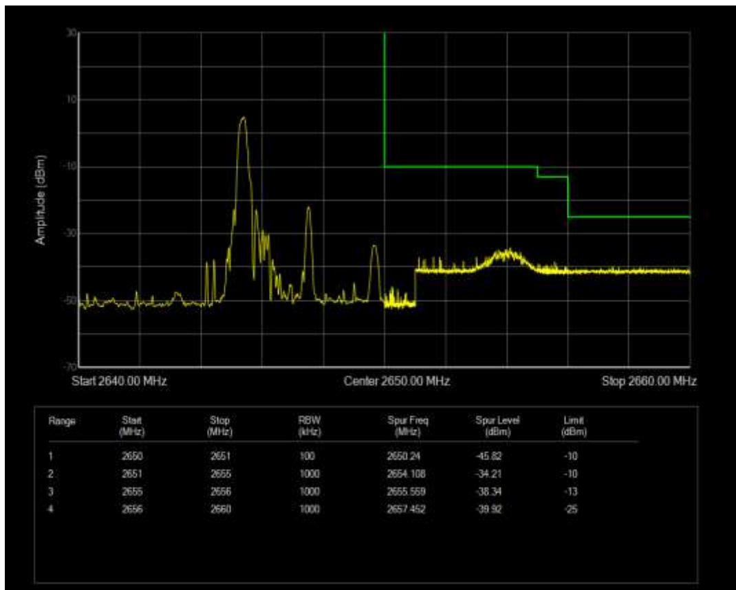
Band41 16QAM BW=5MHz Channel=41165 RB Size=1 Position=#Max
