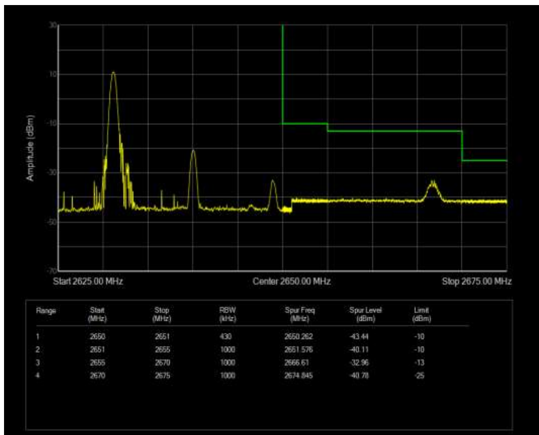
Band41 QPSK BW=20MHz Channel=41090 RB Size=1 Position=#Max
