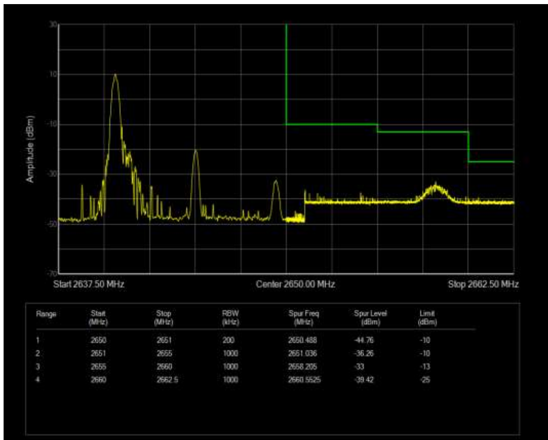
Band41 16QAM BW=10MHz Channel=41140 RB Size=1 Position=#Max
