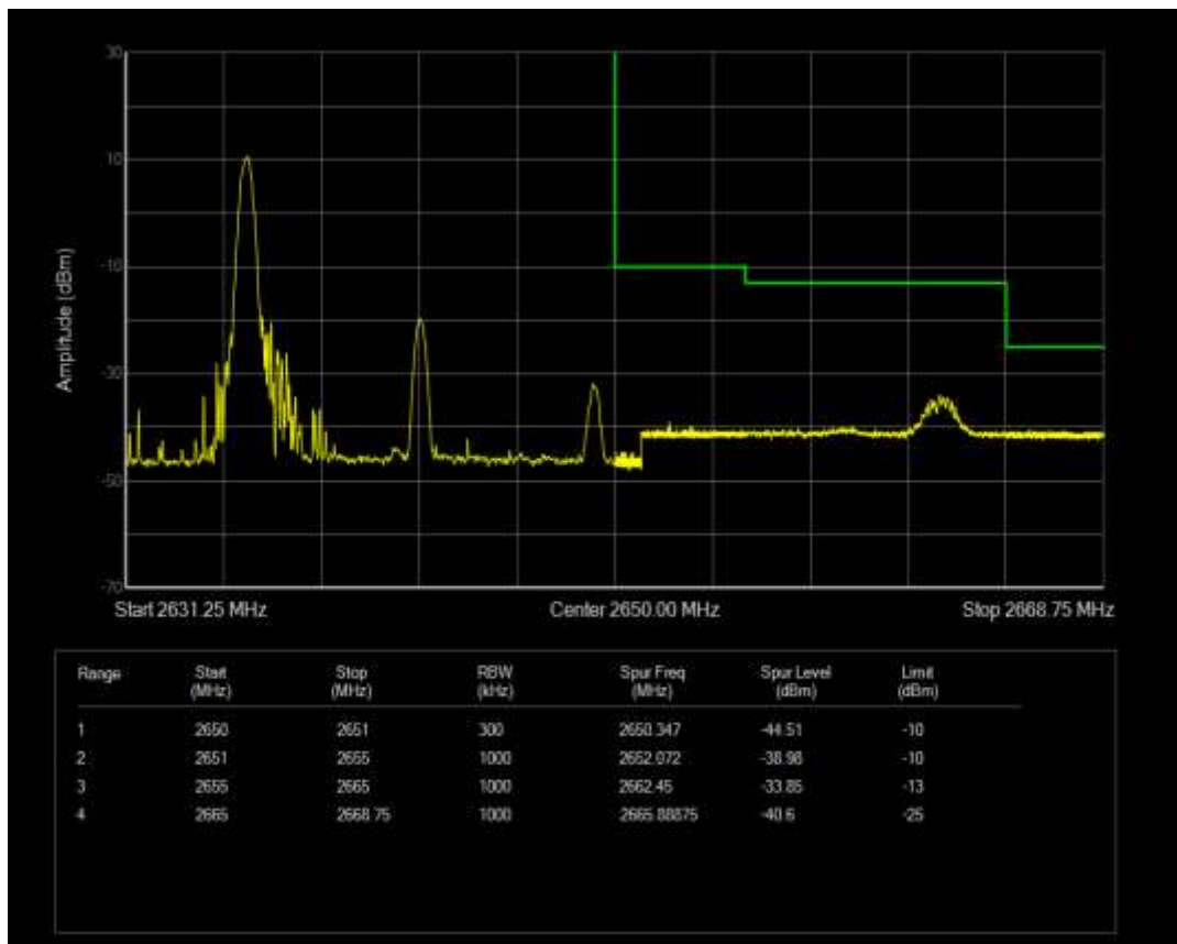
Band41 16QAM BW=15MHz Channel=41115 RB Size=1 Position=#Max
