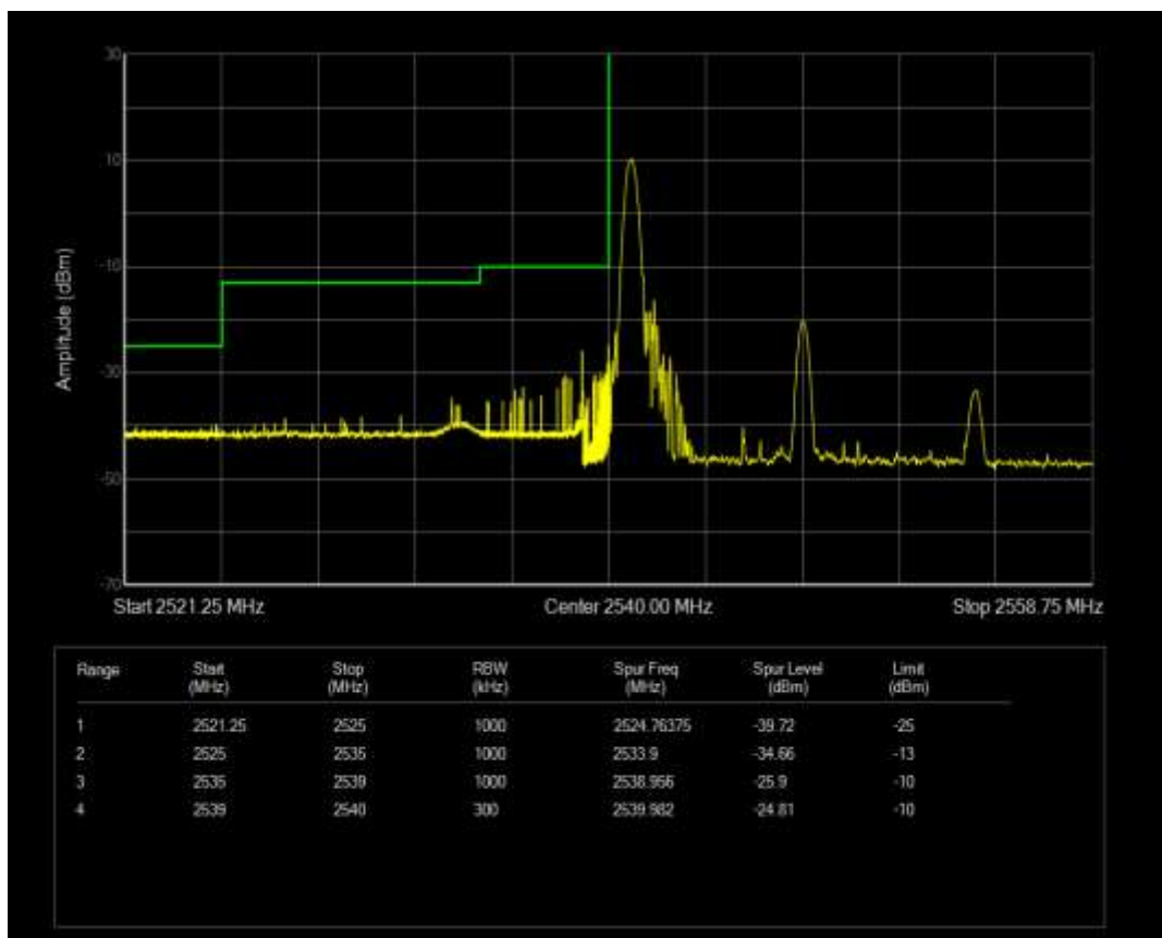
Band41 QPSK BW=15MHz Channel=40165 RB Size=1 Position=#Max
