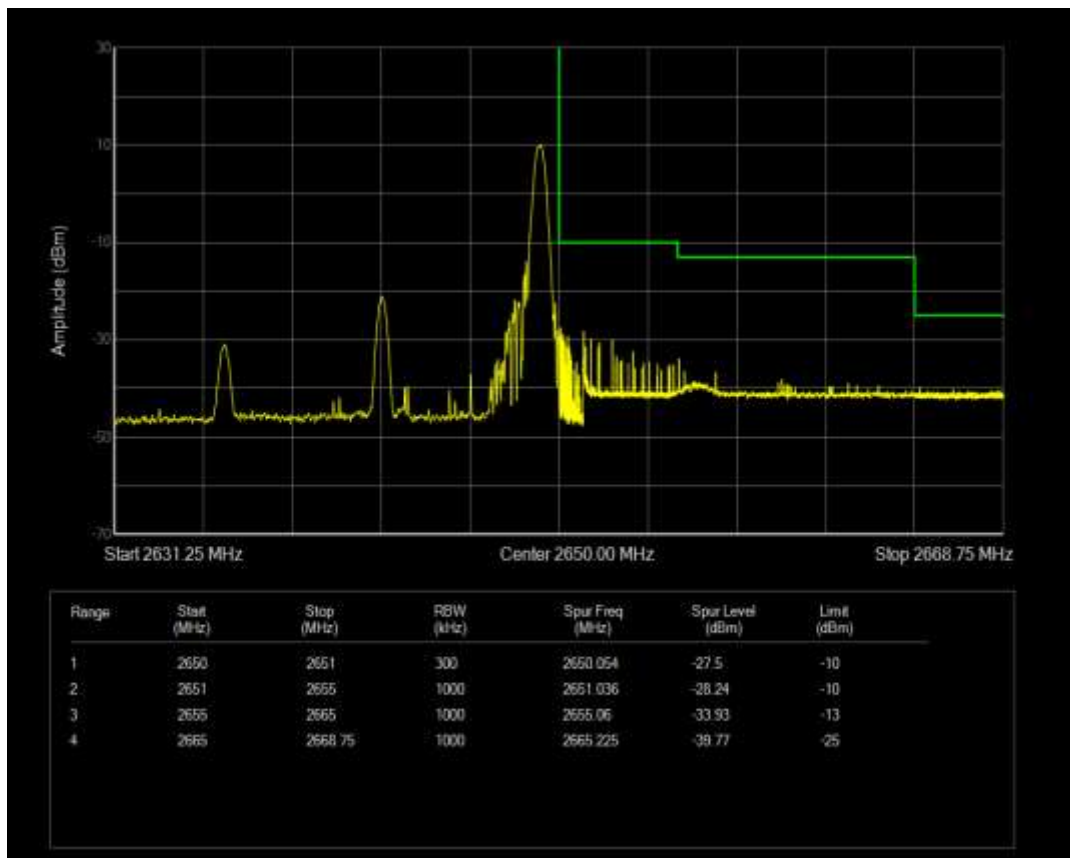
Band41 QPSK BW=15MHz Channel=41115 RB Size=75 Position=#0
