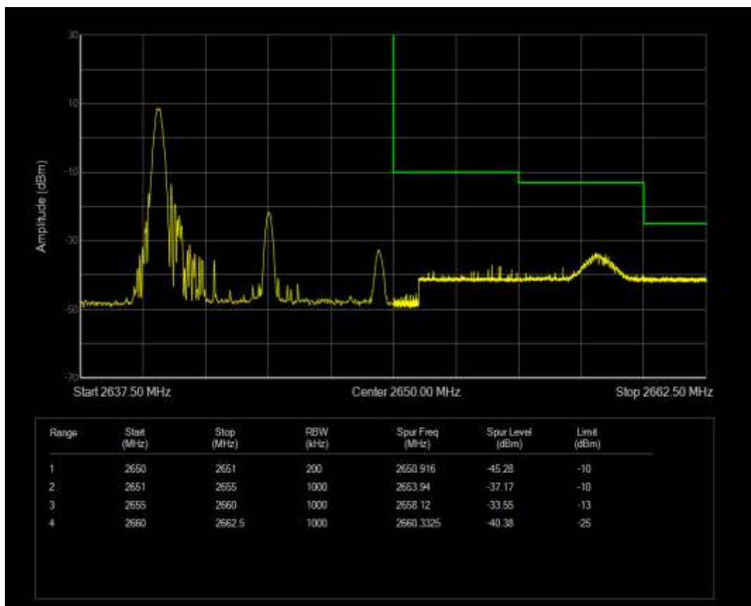
Band41 QPSK BW=10MHz Channel=41140 RB Size=1 Position=#Max
