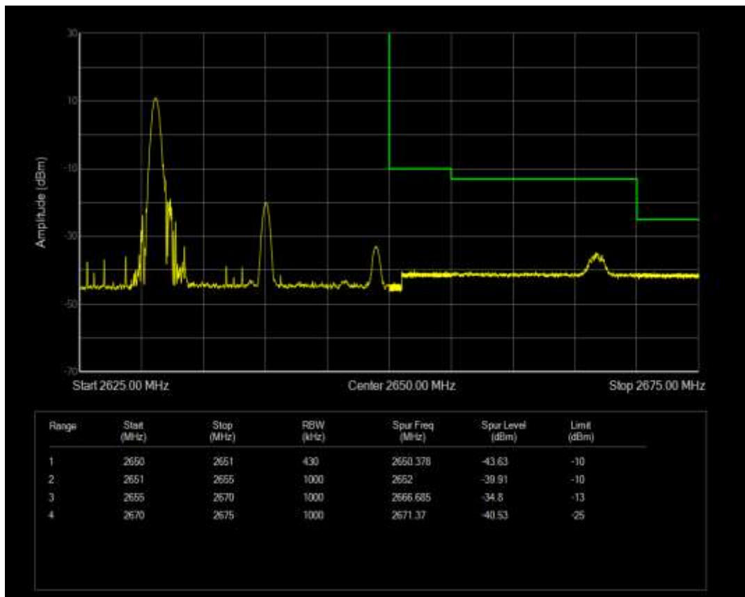
Band41 16QAM BW=20MHz Channel=41090 RB Size=1 Position=#Max
