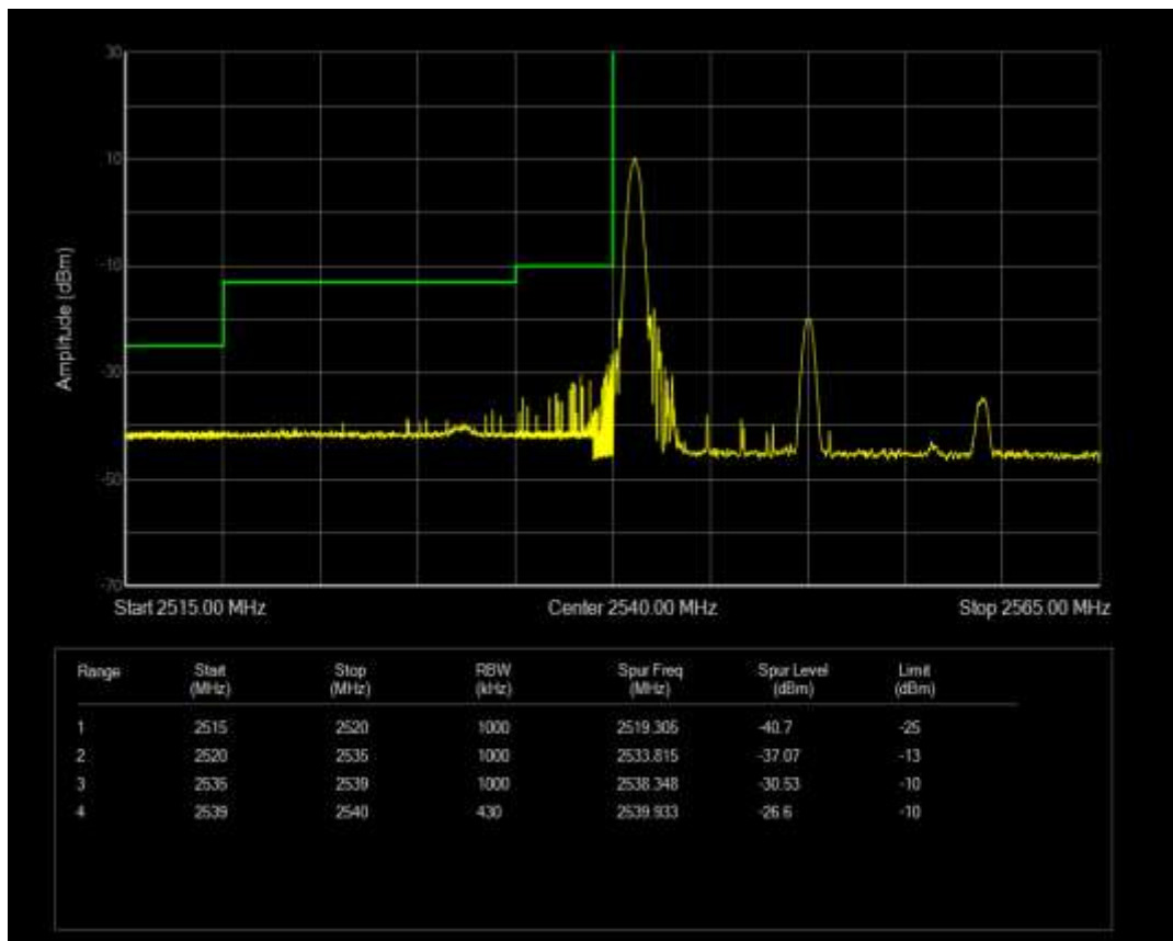
Band41 16QAM BW=20MHz Channel=40190 RB Size=1 Position=#Max
