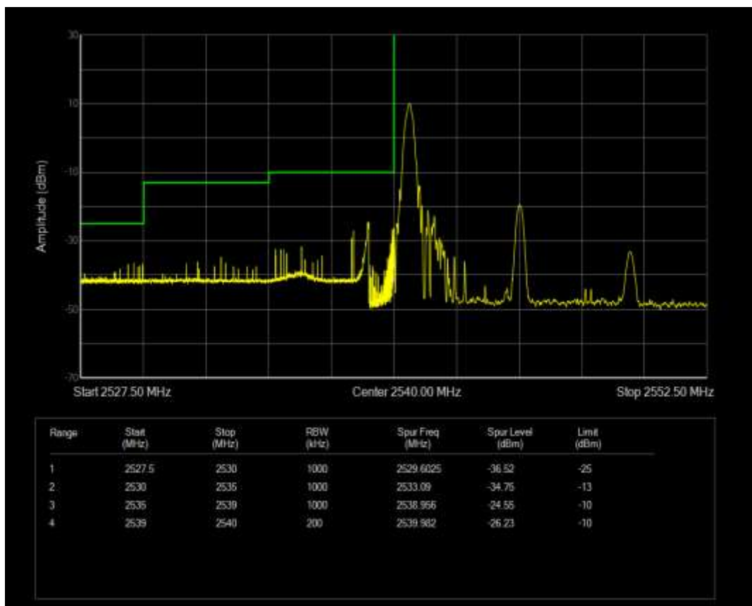
Band41 16QAM BW=10MHz Channel=40140 RB Size=1 Position=#Max
