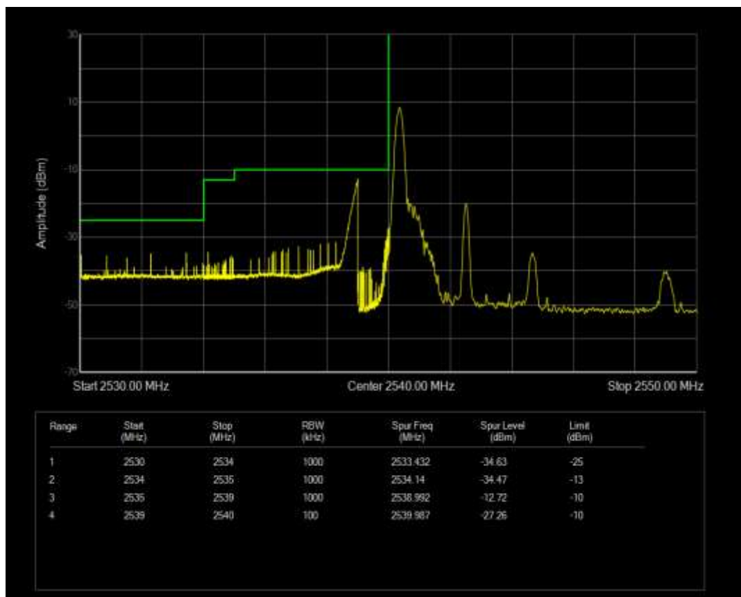
Band41 QPSK BW=5MHz Channel=40115 RB Size=1 Position=#Max
