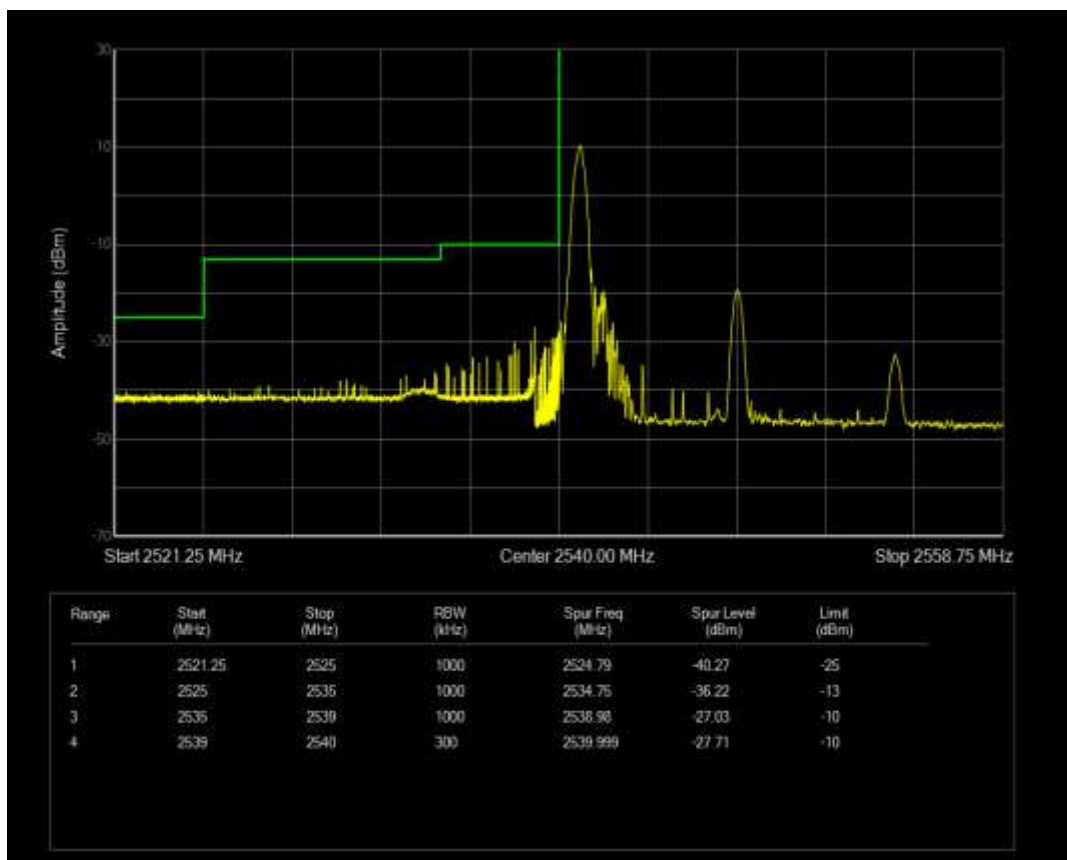
Band41 16QAM BW=15MHz Channel=40165 RB Size=1 Position=#Max
