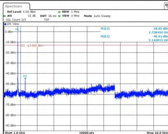
Band66-15MHz-16QAM-132322-1RB#0-Range2:1000~10000MHz
