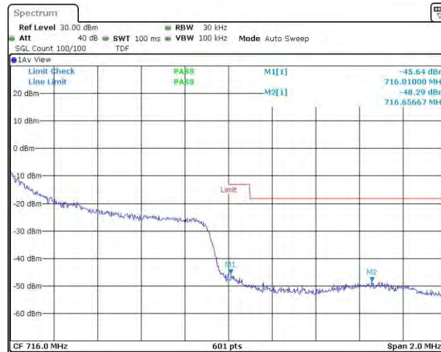
Band12-1.4MHz-16QAM-23173-1RB#5
