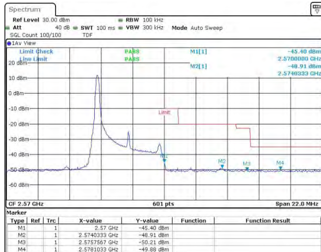
Band7-5MHz-16QAM-21425-1RB#24
