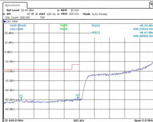
Band12-1.4MHz-16QAM-23017-6RB#0
