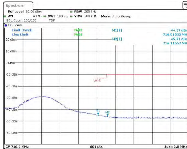
Band12-10MHz-QPSK-23130-1RB#49
