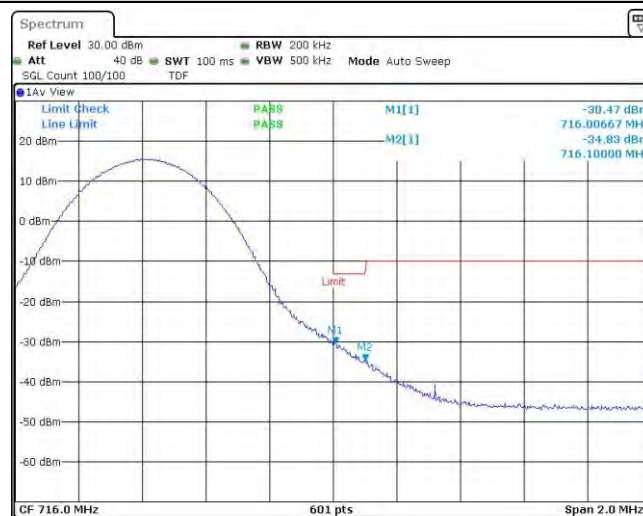
Band12-10MHz-QPSK-23130-50RB#0
