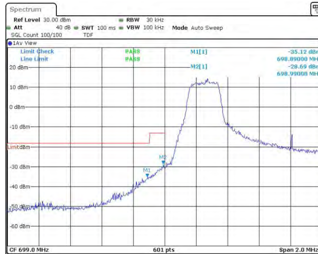
Band12-1.4MHz-16QAM-23017-1RB#5
