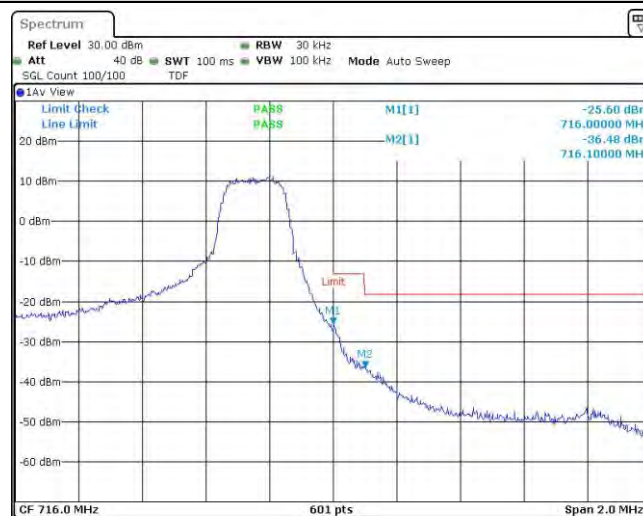
Band12-1.4MHz-16QAM-23173-6RB#0
