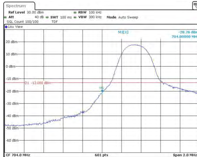
Band17-5MHz-QPSK-23755-1RB#24
