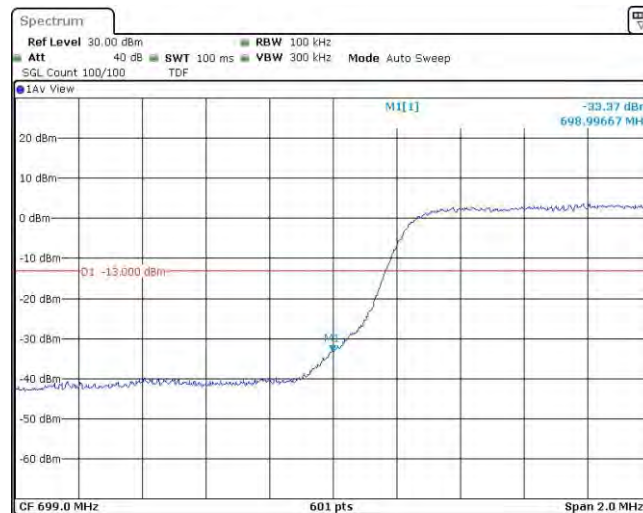
Band12-5MHz-QPSK-23035-1RB#24
