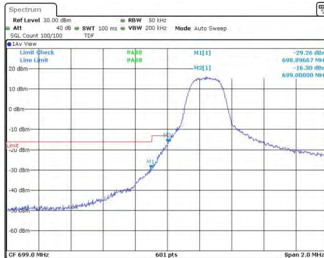
Band12-3MHz-QPSK-23025-1RB#14
