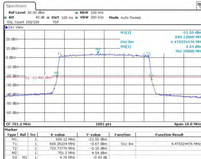
Band12-5MHz-16QAM-23095-25RB#0
