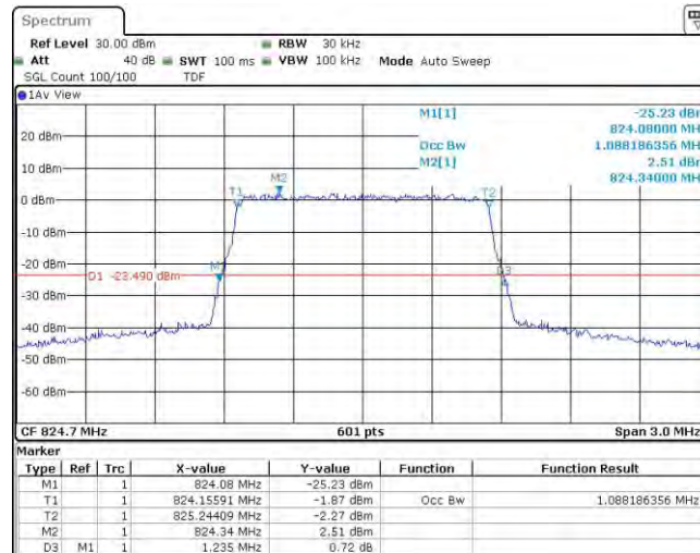
Band5-1.4MHz-16QAM-20525-6RB#0
