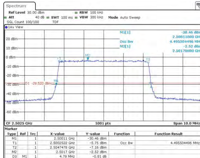
Band7-5MHz-16QAM-21100-25RB#0
