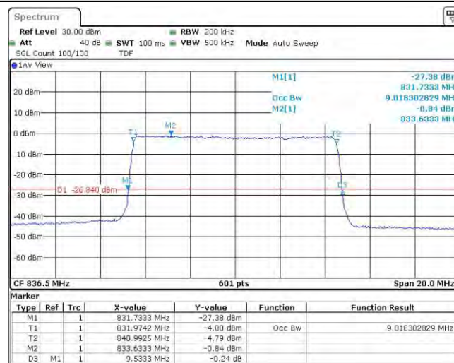
Band5-10MHz-QPSK-20600-50RB#0
