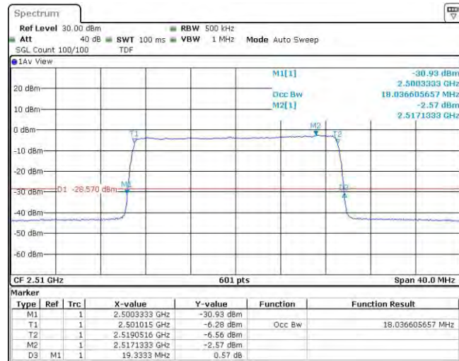
Band7-20MHz-QPSK-21100-100RB#0
