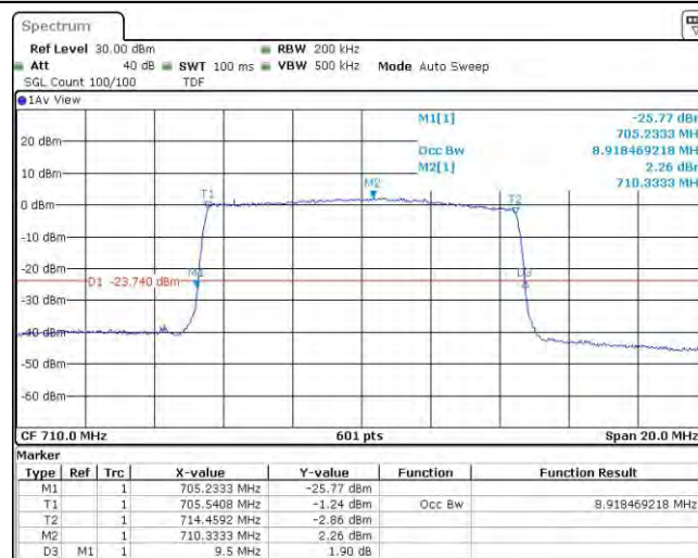
Band17-10MHz-16QAM-23790-50RB#0
