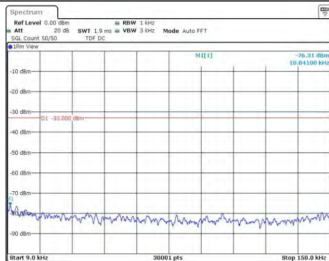
Band5-4132-4-0.009~0.15MHz
