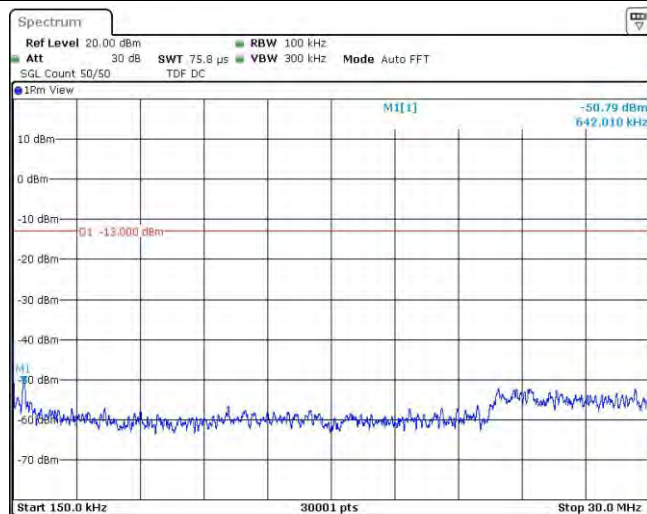
Band5-4182-1-0.15~30MHz
