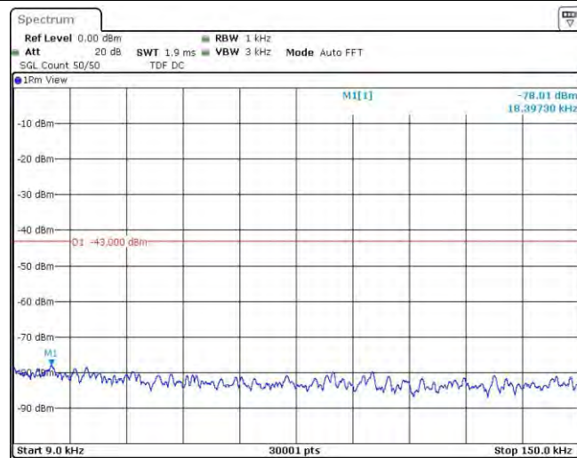
Band4-1413-3-0.009~0.15MHz
