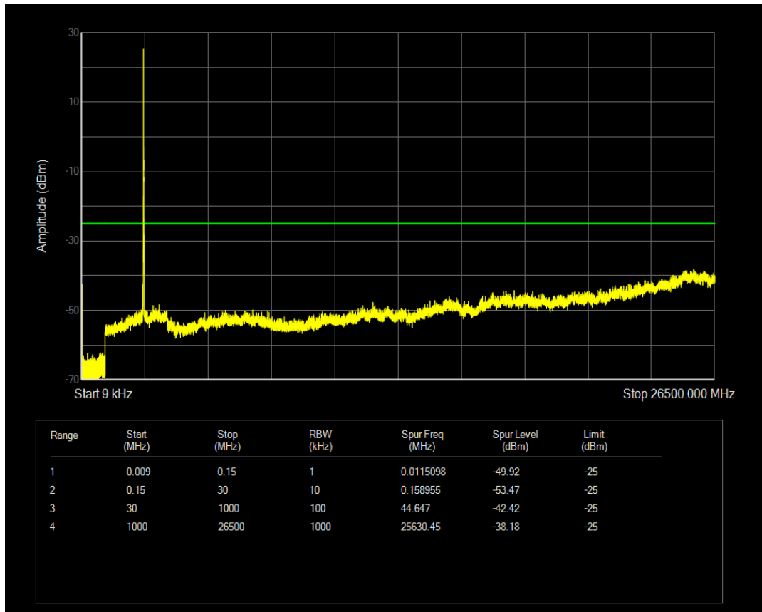
Band41 16QAM BW=15MHz Channel=40815 RB Size=75 Position=#0
