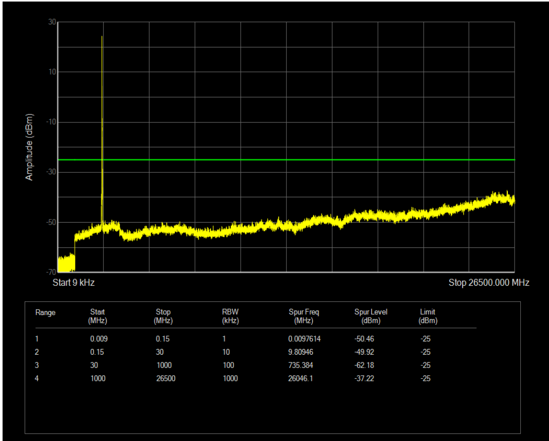
Band41 16QAM BW=20MHz Channel=40490 RB Size=100 Position=#0
