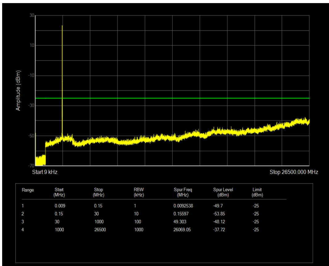
Band41 QPSK BW=10MHz Channel=40840 RB Size=50 Position=#0
