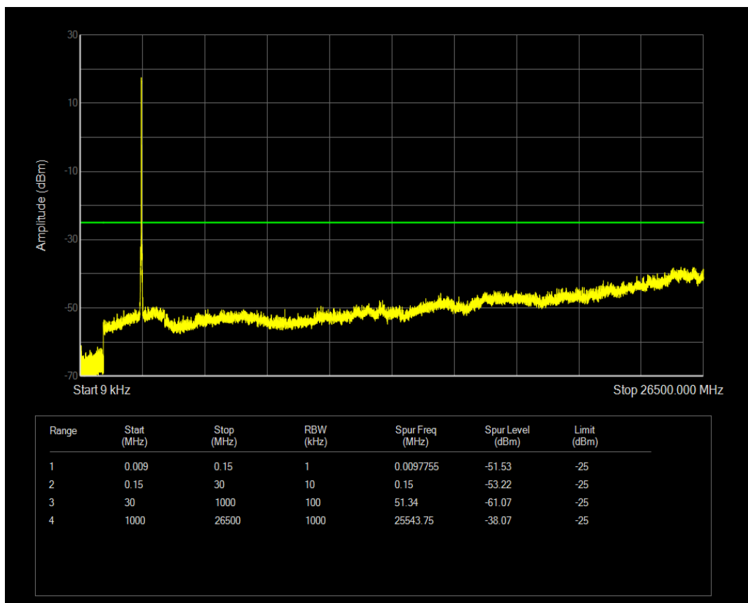
Band41 16QAM BW=15MHz Channel=40815 RB Size=1 Position=#0
