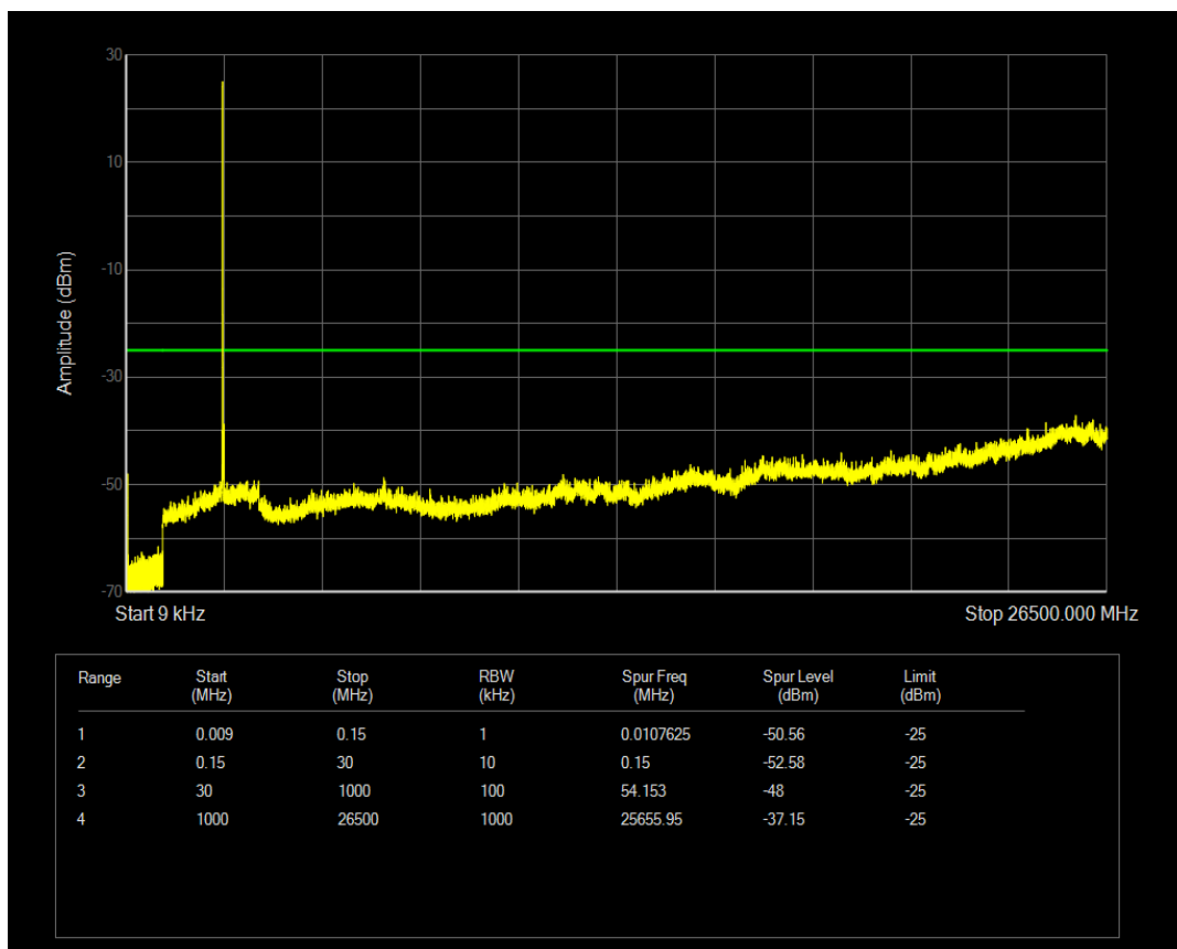
Band41 QPSK BW=5MHz Channel=40865 RB Size=25 Position=#0
