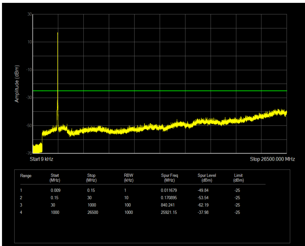
Band41 16QAM BW=20MHz Channel=40790 RB Size=1 Position=#0
