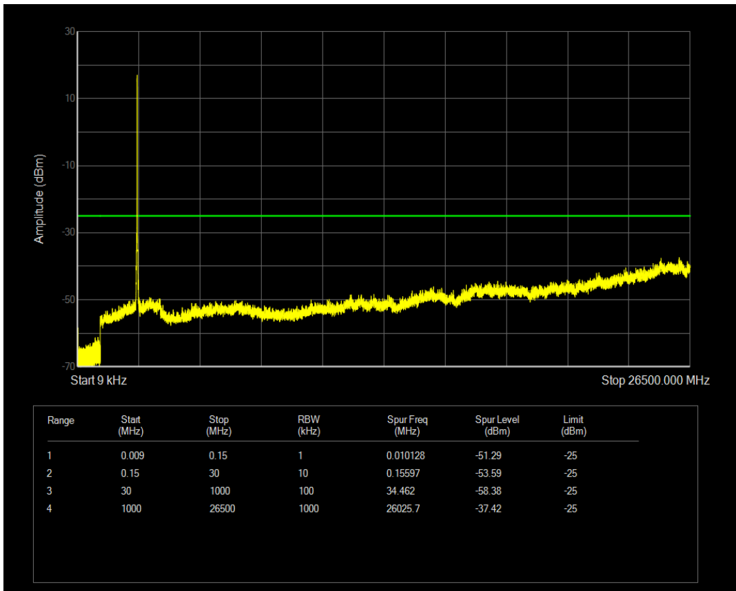
Band41 QPSK BW=15MHz Channel=40815 RB Size=1 Position=#0
