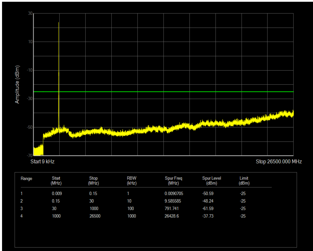
Band41 16QAM BW=15MHz Channel=40465 RB Size=75 Position=#0
