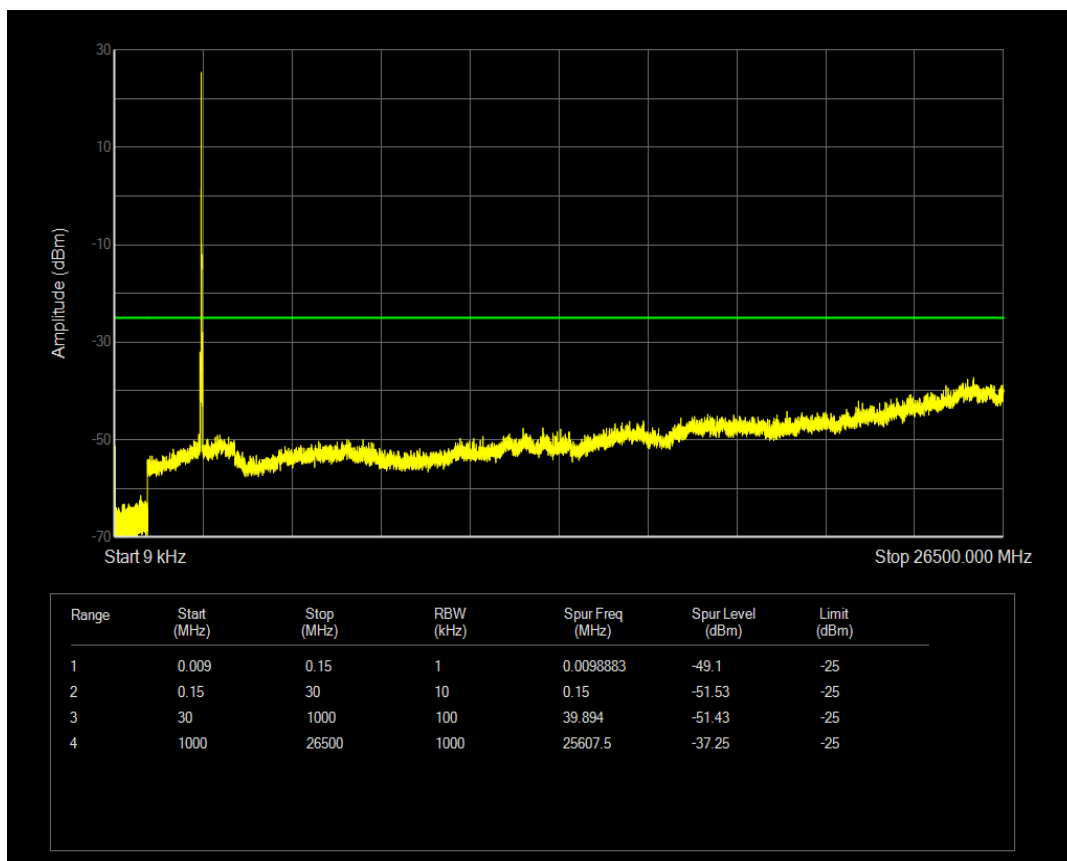
Band41 16QAM BW=20MHz Channel=40790 RB Size=100 Position=#0
