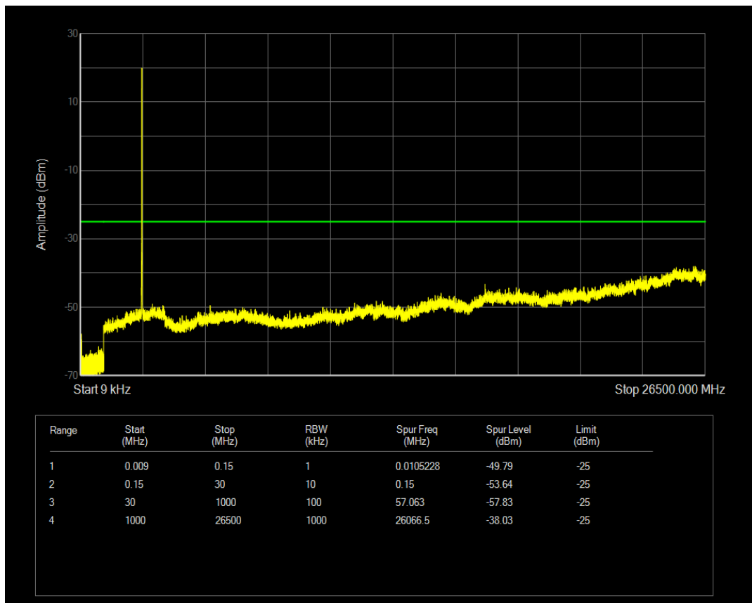
Band41 QPSK BW=10MHz Channel=40440 RB Size=1 Position=#0
