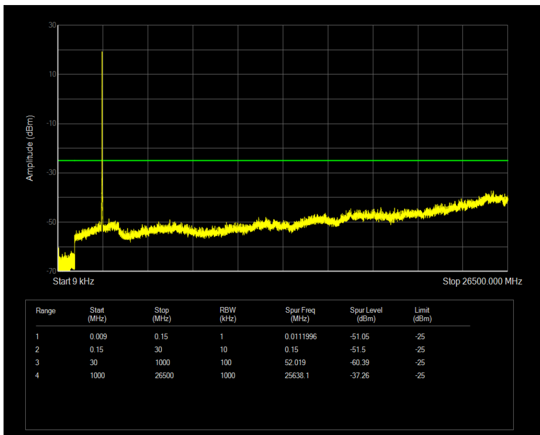
Band41 QPSK BW=15MHz Channel=40465 RB Size=1 Position=#0
