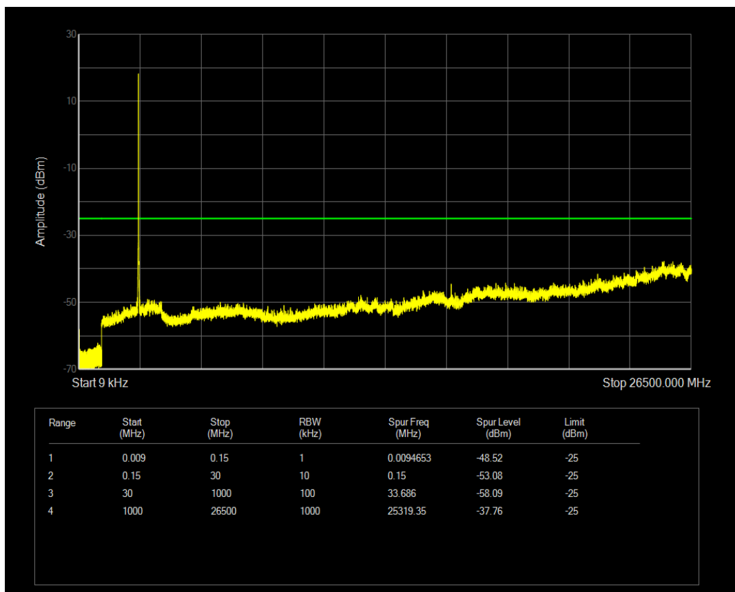
Band41 QPSK BW=10MHz Channel=40840 RB Size=1 Position=#0
