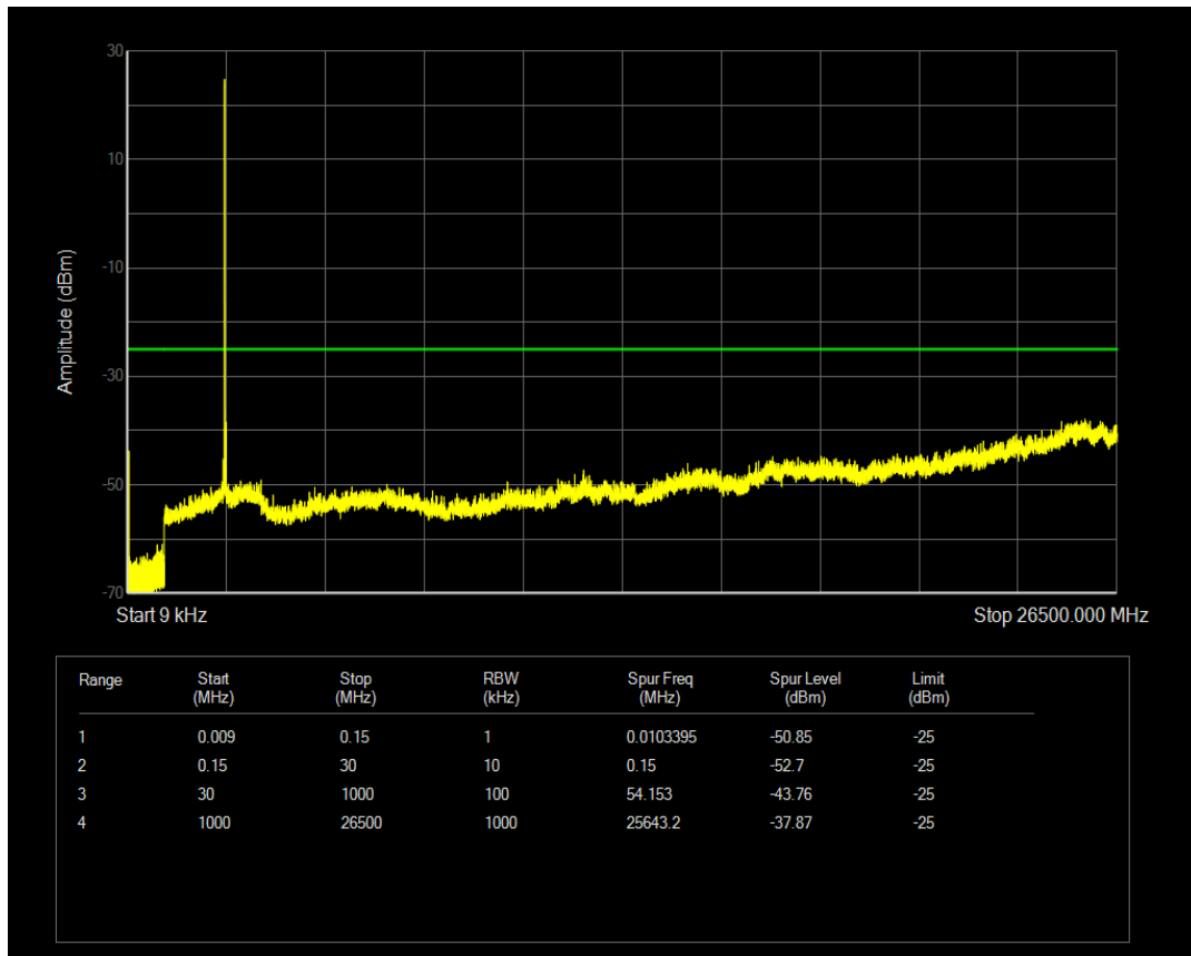
Band41 16QAM BW=5MHz Channel=40865 RB Size=25 Position=#0
