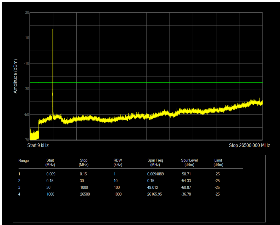
Band41 QPSK BW=20MHz Channel=40490 RB Size=1 Position=#0
