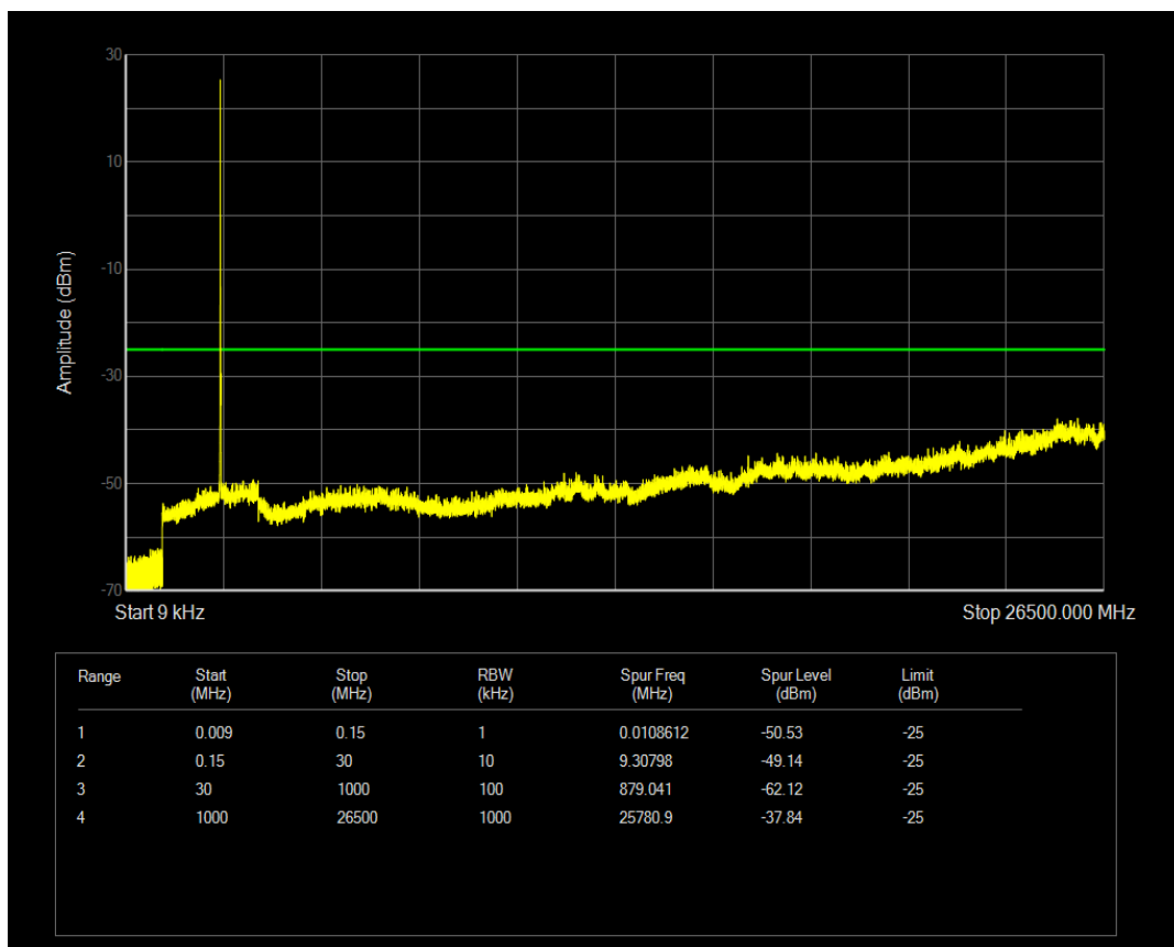
Band41 16QAM BW=10MHz Channel=40440 RB Size=50 Position=#0
