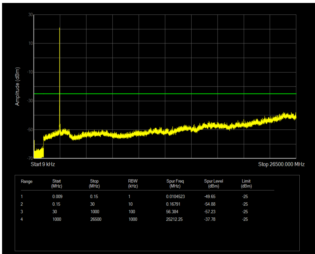
Band41 16QAM BW=5MHz Channel=40865 RB Size=1 Position=#0
