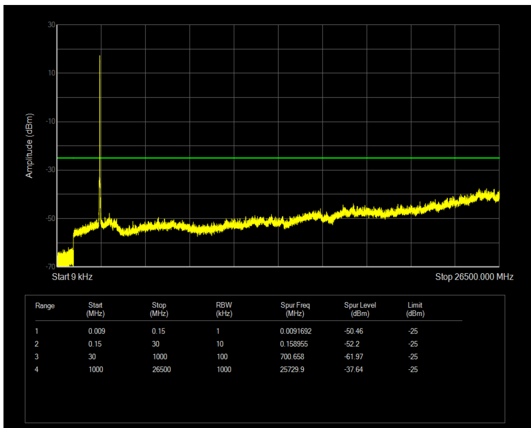
Band41 16QAM BW=15MHz Channel=40465 RB Size=1 Position=#0
