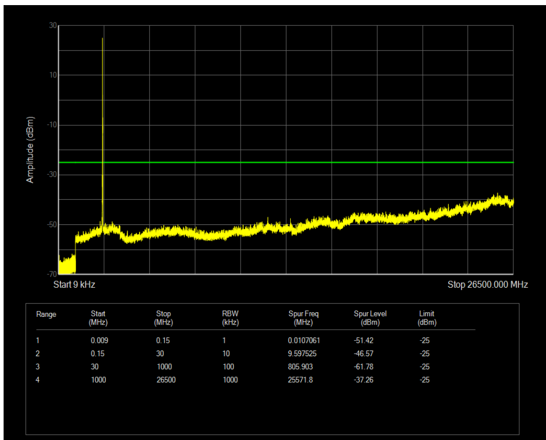
Band41 QPSK BW=15MHz Channel=40465 RB Size=75 Position=#0
