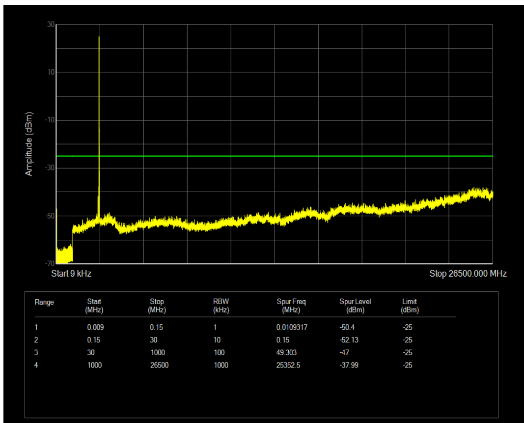
Band41 16QAM BW=10MHz Channel=40840 RB Size=50 Position=#0
