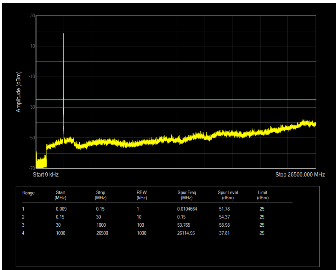
Band41 16QAM BW=10MHz Channel=40840 RB Size=1 Position=#0
