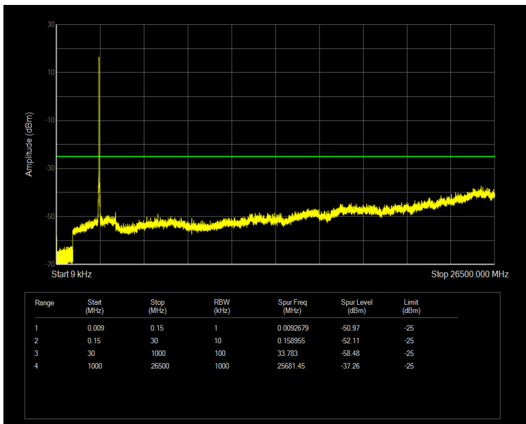
Band41 16QAM BW=20MHz Channel=40640 RB Size=1 Position=#0
