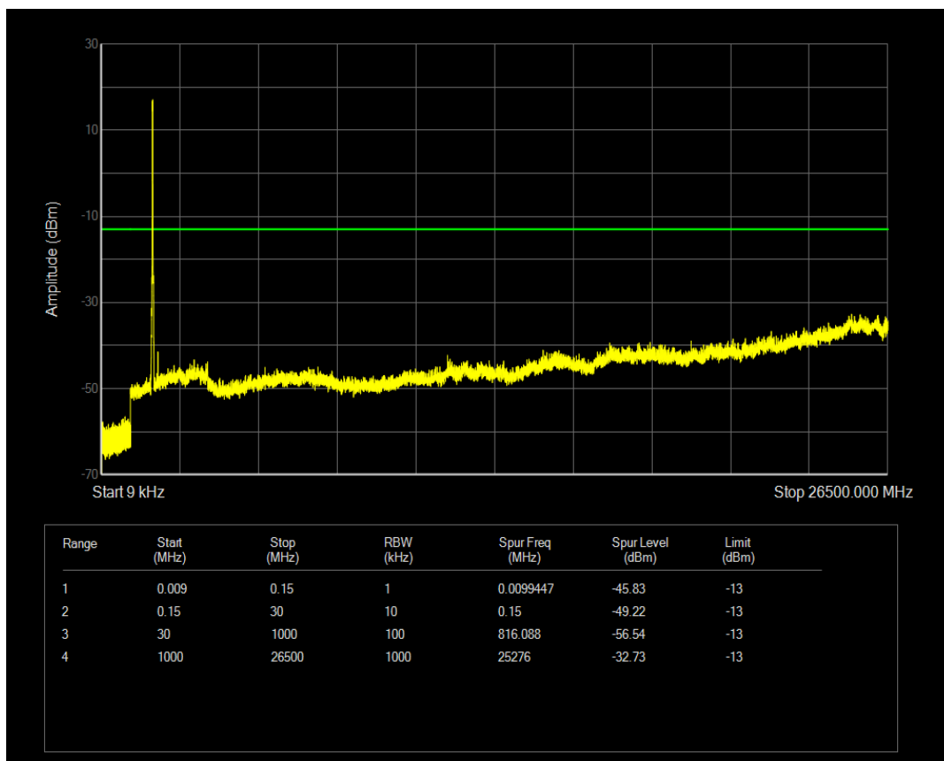
Band41 QPSK BW=5MHz Channel=40415 RB Size=1 Position=#0
