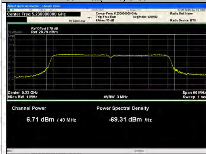
802.11ac(VH40)-5230
