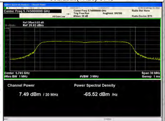
802.11ac(VH20)-5745
