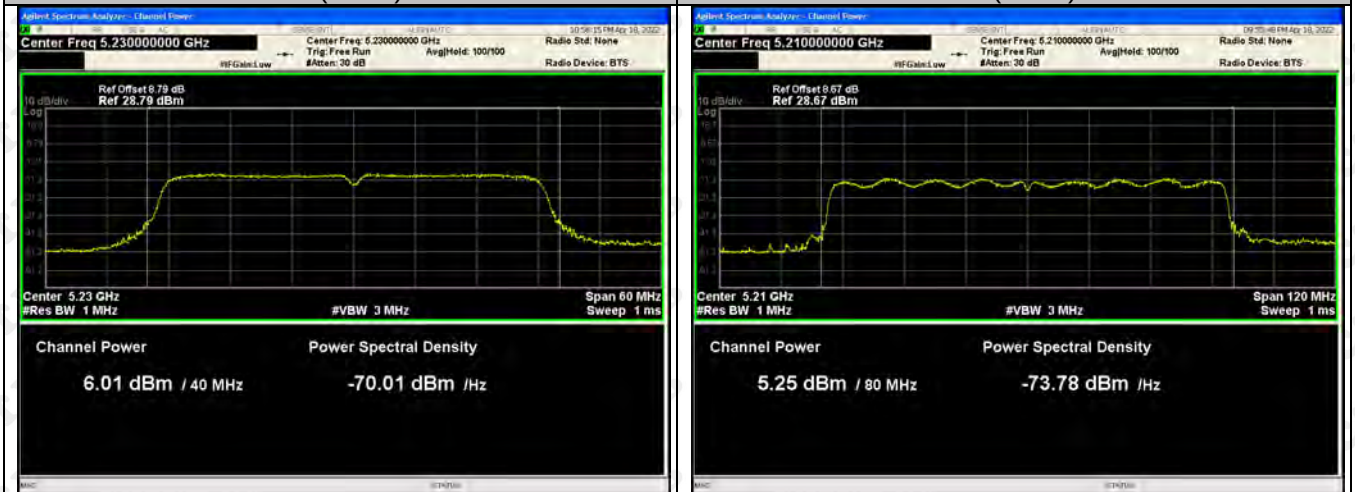
802.11ac(VH40)-5230
