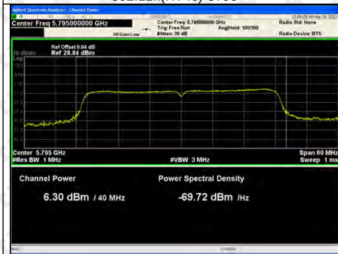
802.11n(HT40)-5795
