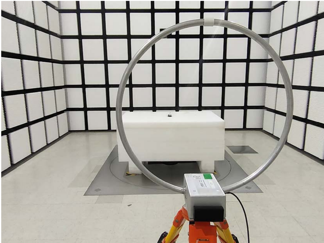
Radiated Emission 9 kHz-30 MHz Perpendicular View PCBA_1
