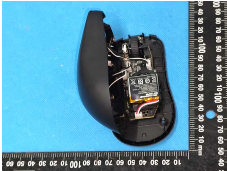
PCBA_1
