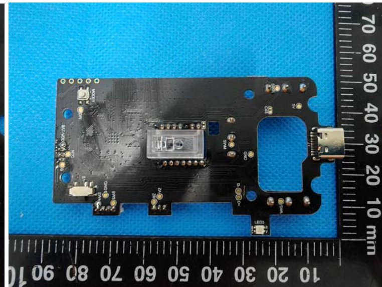
PCBA_1
