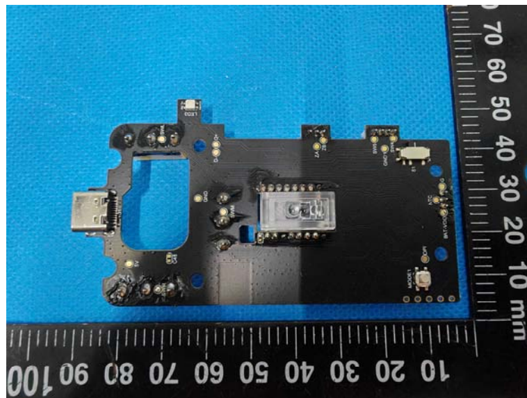
PCBA_2
