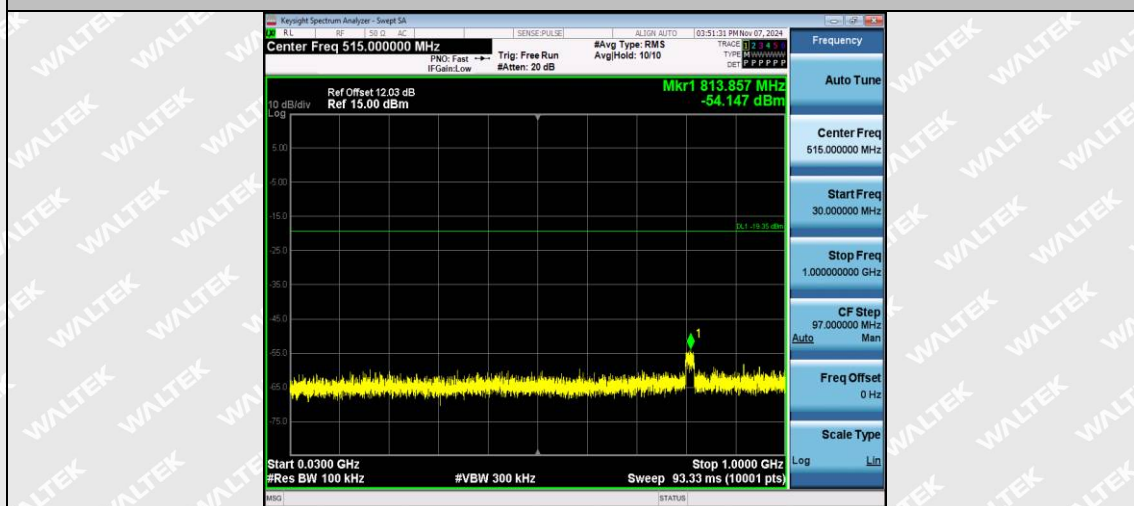
11N20SISO-Ant1-2437-30~1000-PASS
