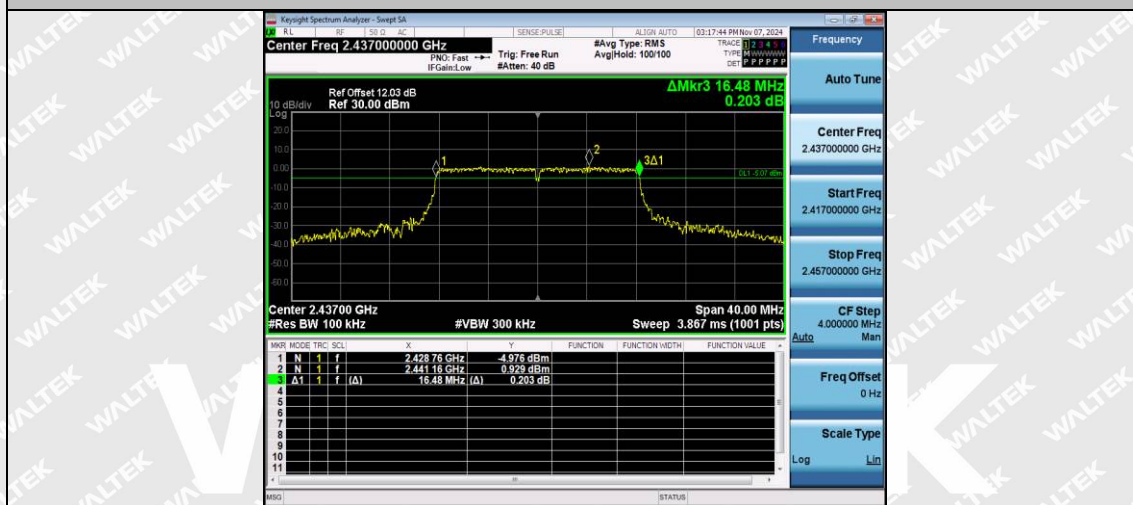
11G-Ant1-2437-PASS
