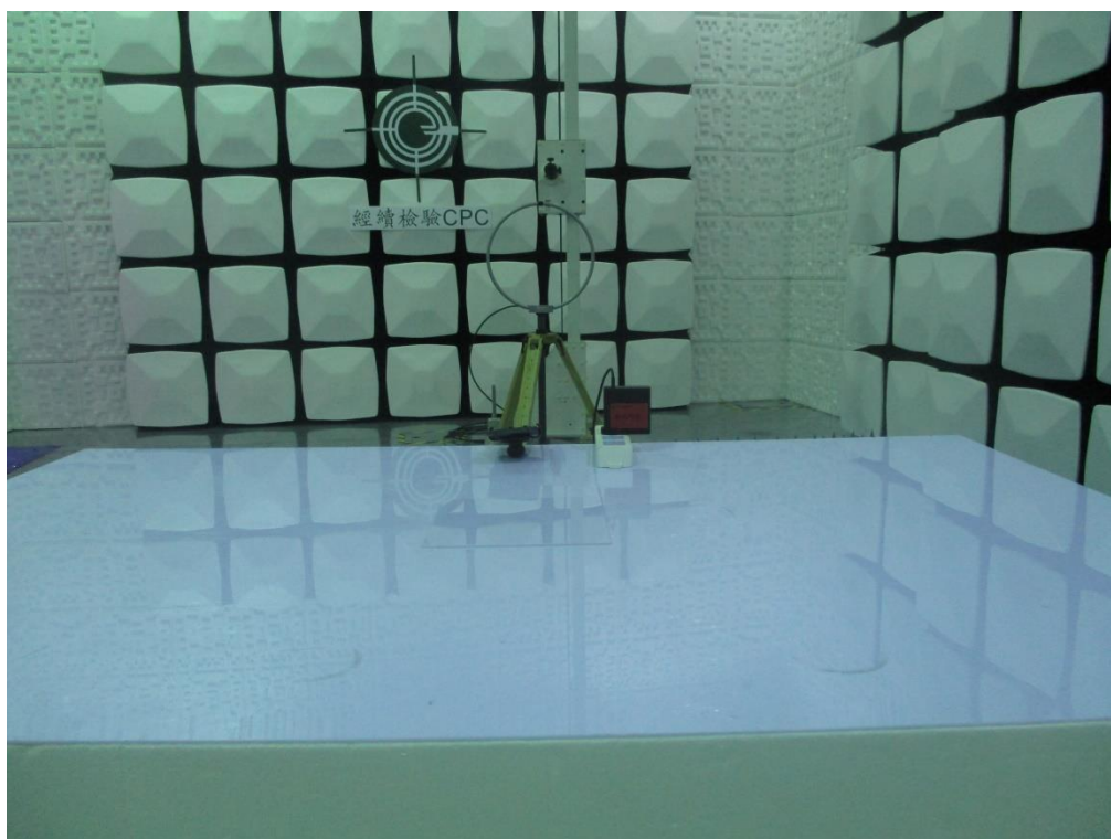
Setup Photo FCC ID: 2A7CC118A-15W
